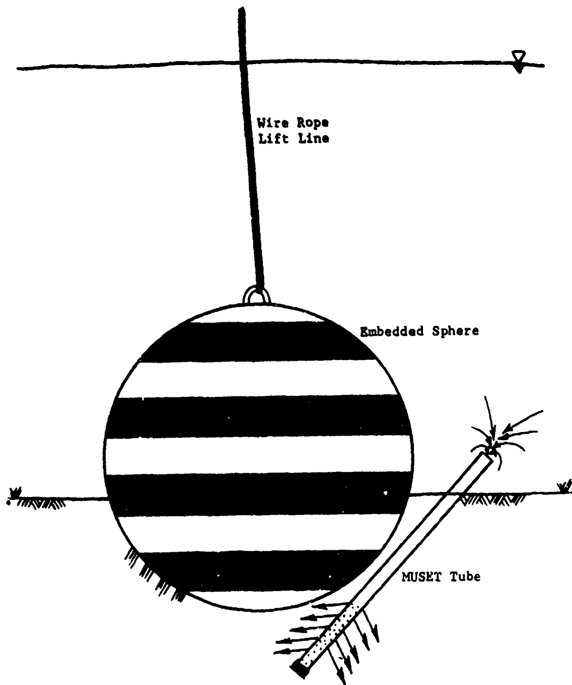
Figure 1. Placement of MUSET Tubes
