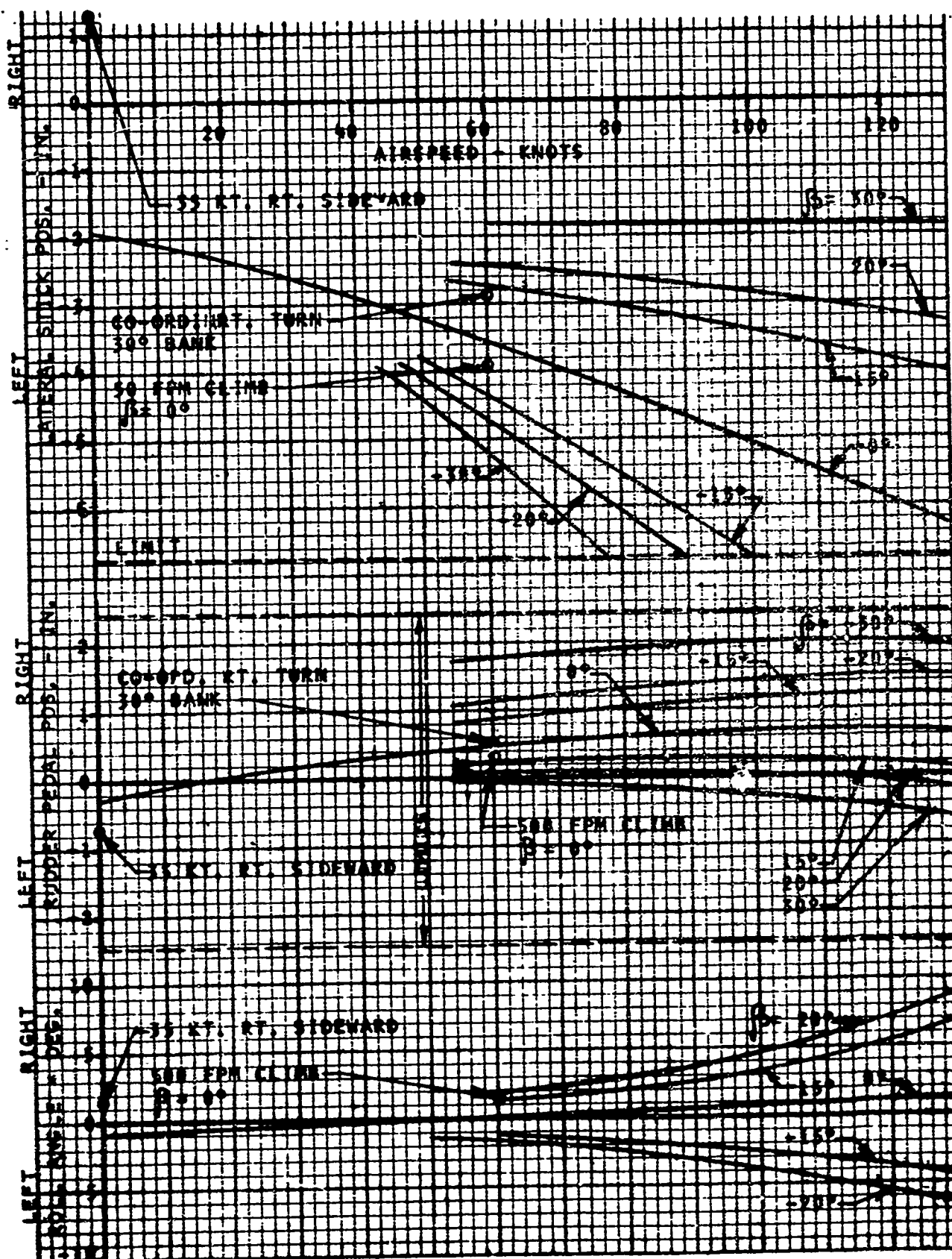
FIGURE 4-28. MHHLS LATERAL-DIRECTIONAL TRIM G.W. = 87,300 LB., S.L., 59°F.
