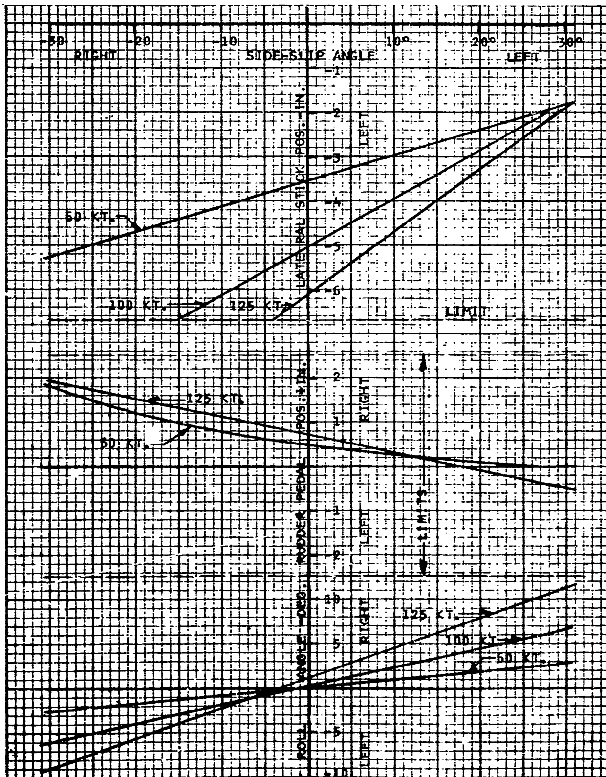
FIGURE 4-31. MHHLS LATERAL-DIRECTIONAL STATIC STABILITY G.W. = 87,300 LB., S.L. 59°F.
