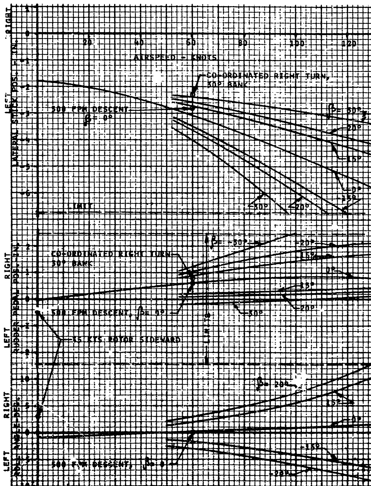
FIGURE 4-27. MHHLS LATERAL-DIRECTIONAL TRIM G.W. = 59,486 LB., S.L. 59°F.
