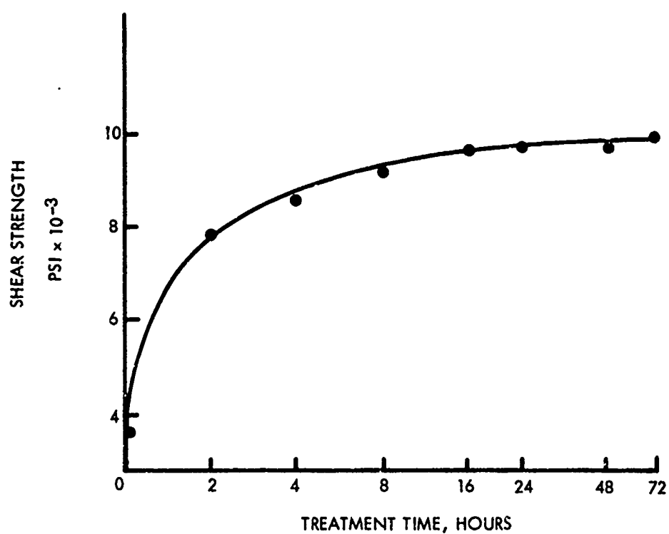
FIG. 2 SHEAR STRENGTH VS. TREATMENT TIME FOR THE SODIUM HYPOCHLORITE OXIDATION TREATMENT (1)
