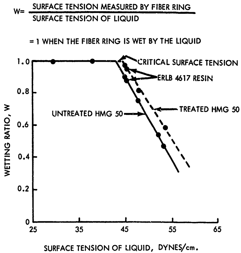
FIG. B-1 CRITICAL SURFACE TENSION OF FIBERS DETERMINED BY THE FIBER RING METHOD
