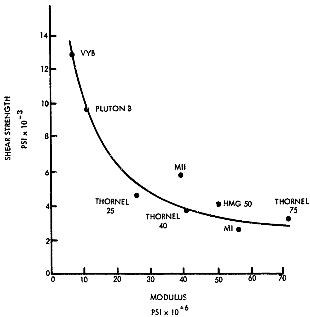
FIG. 14 SHEAR STRENGTH VS. FIBER MODULUS (51) (UNTREATED FIBERS)
