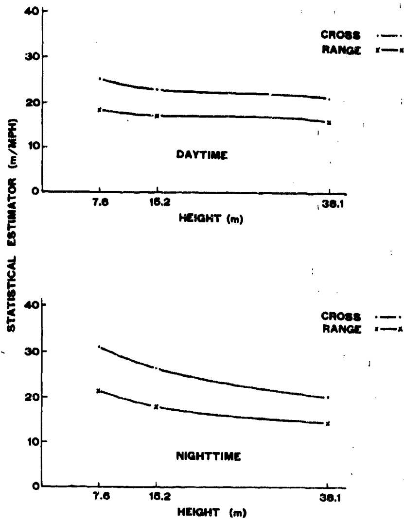
FIGURE 2. WSMR 200 MILS G.E., STATISTICAL ESTIMATOR VERSUS HEIGHT; VALID FOR SPRING 1969 DATA— 184 DAYTIME AND 140 NIGHTTIME WIND PROFILES.
