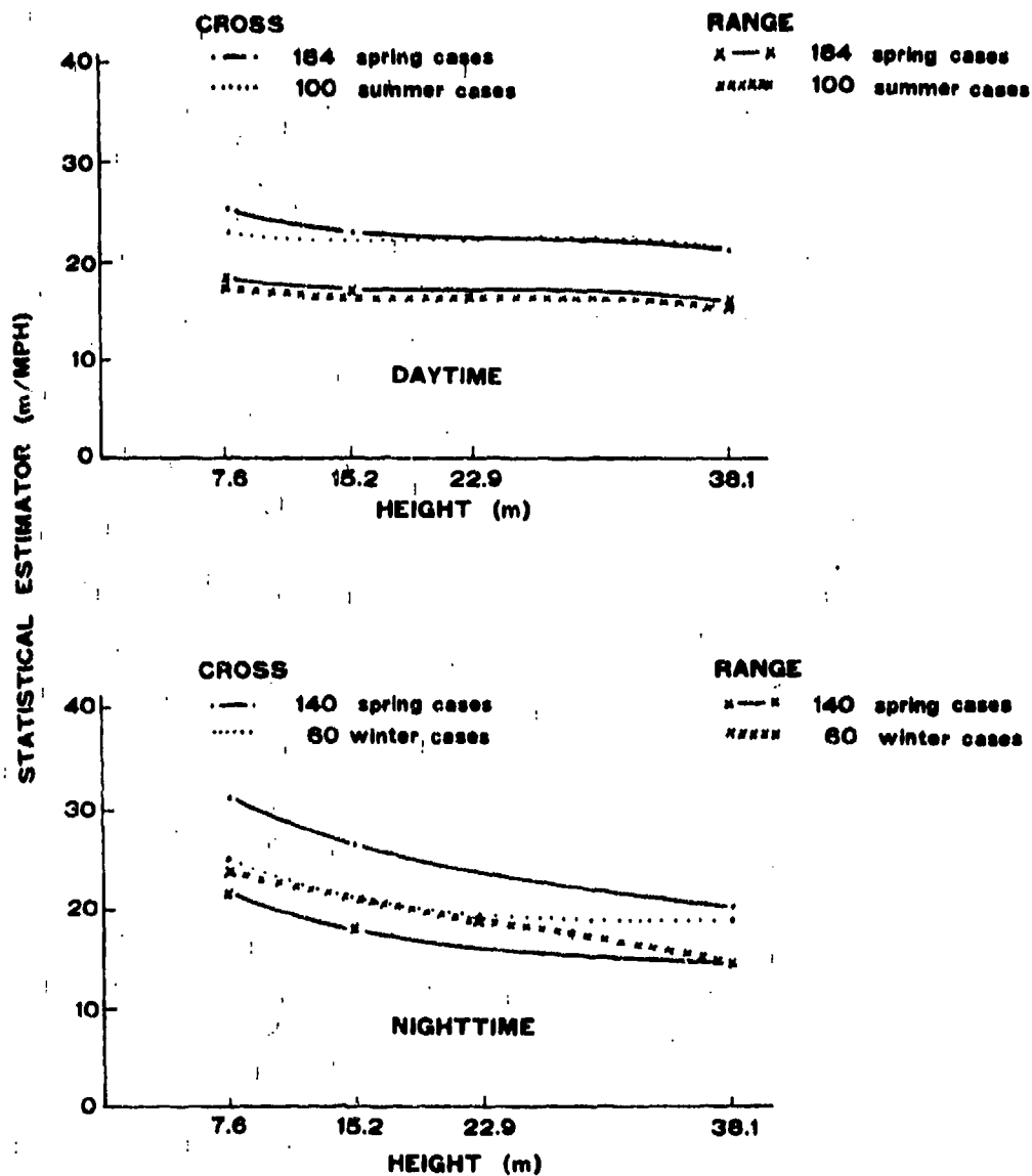
FIGURE 3. WSMR 200 MILS Q.E., STATISTICAL ESTIMATOR COMPARED SEASONALLY; 184 AND 140 MARCH 1969 WIND PROFILES AGAINST 100 JUNE-JULY 1967 AND 60 DECEMBER 1967 WIND PROFILES.
