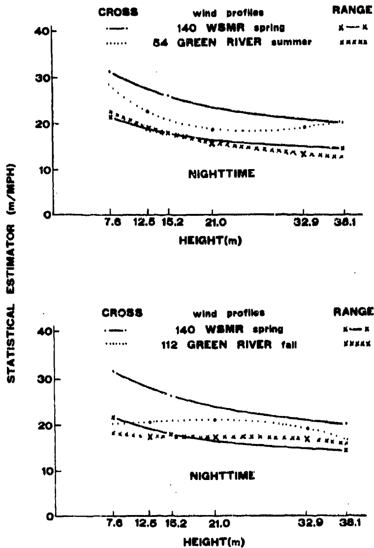
FIGURE 4. WSMR AND GREEN RIVER 200 MILS G.E., STATISTICAL ESTIMATOR COMPARISON; WSMR 140 MARCH 1969 WIND PROFILES AND GREEN RIVER 54 JUNE 1969 AND 112 AUGUST, SEPTEMBER, AND OCTOBER 1967 WIND PROFILES.
