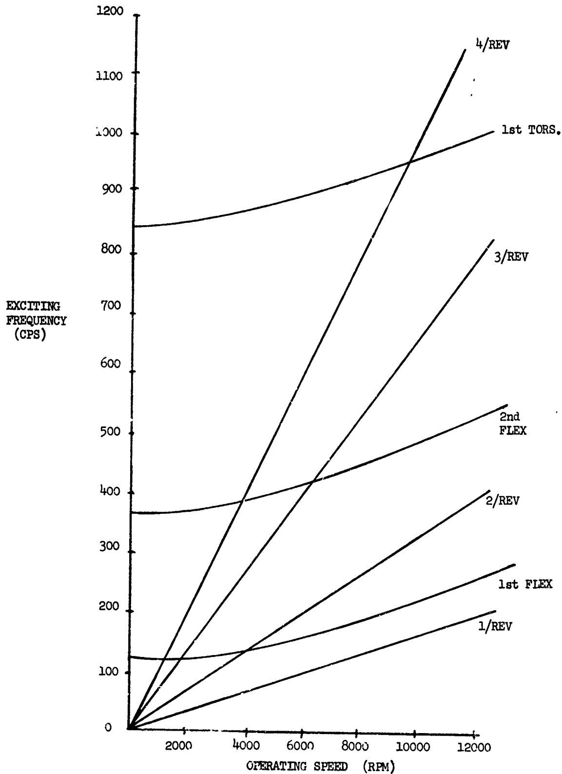
Figure 12. Campbell Diagram
