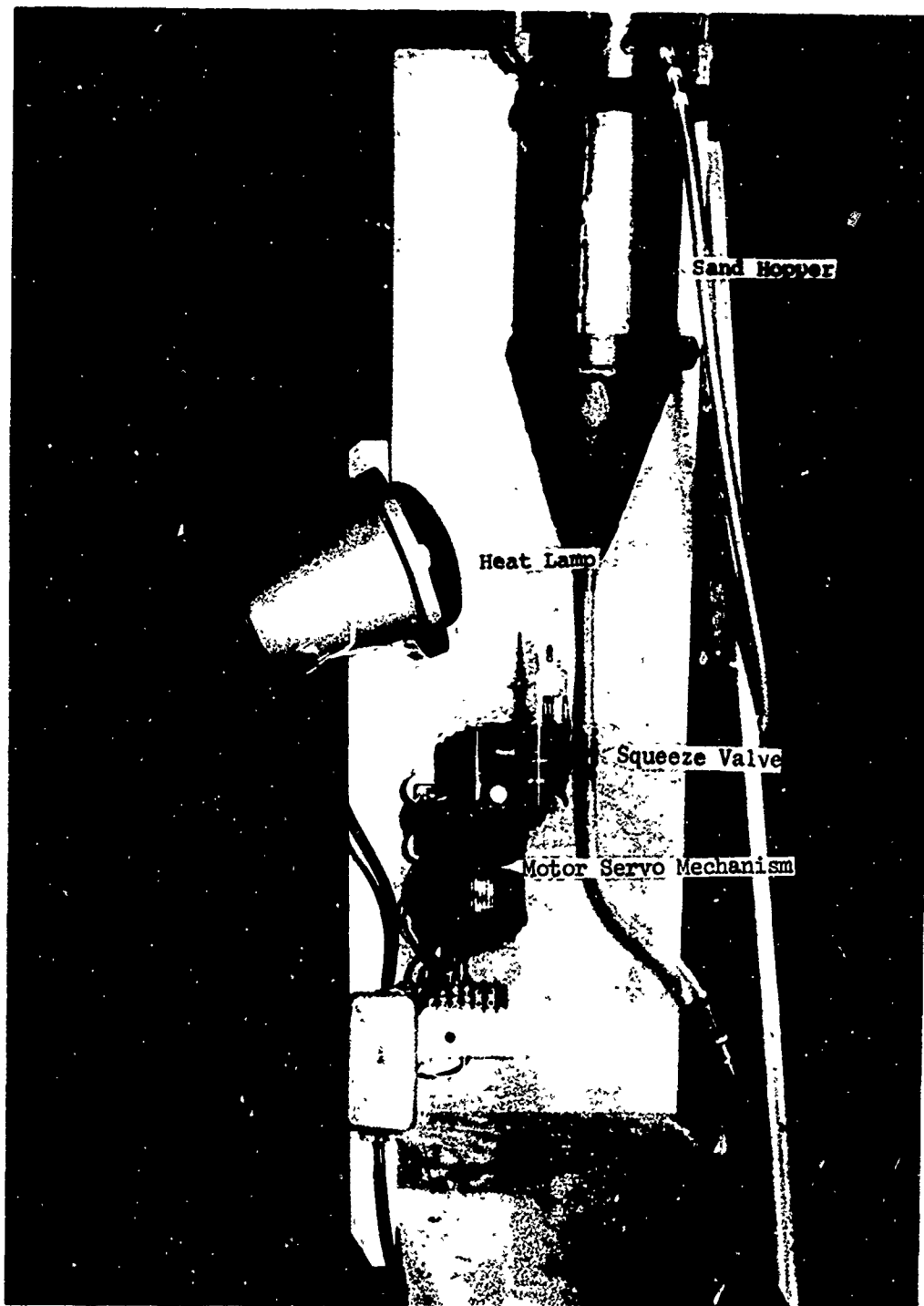
Figure 7. Sand Feed Mechanism
