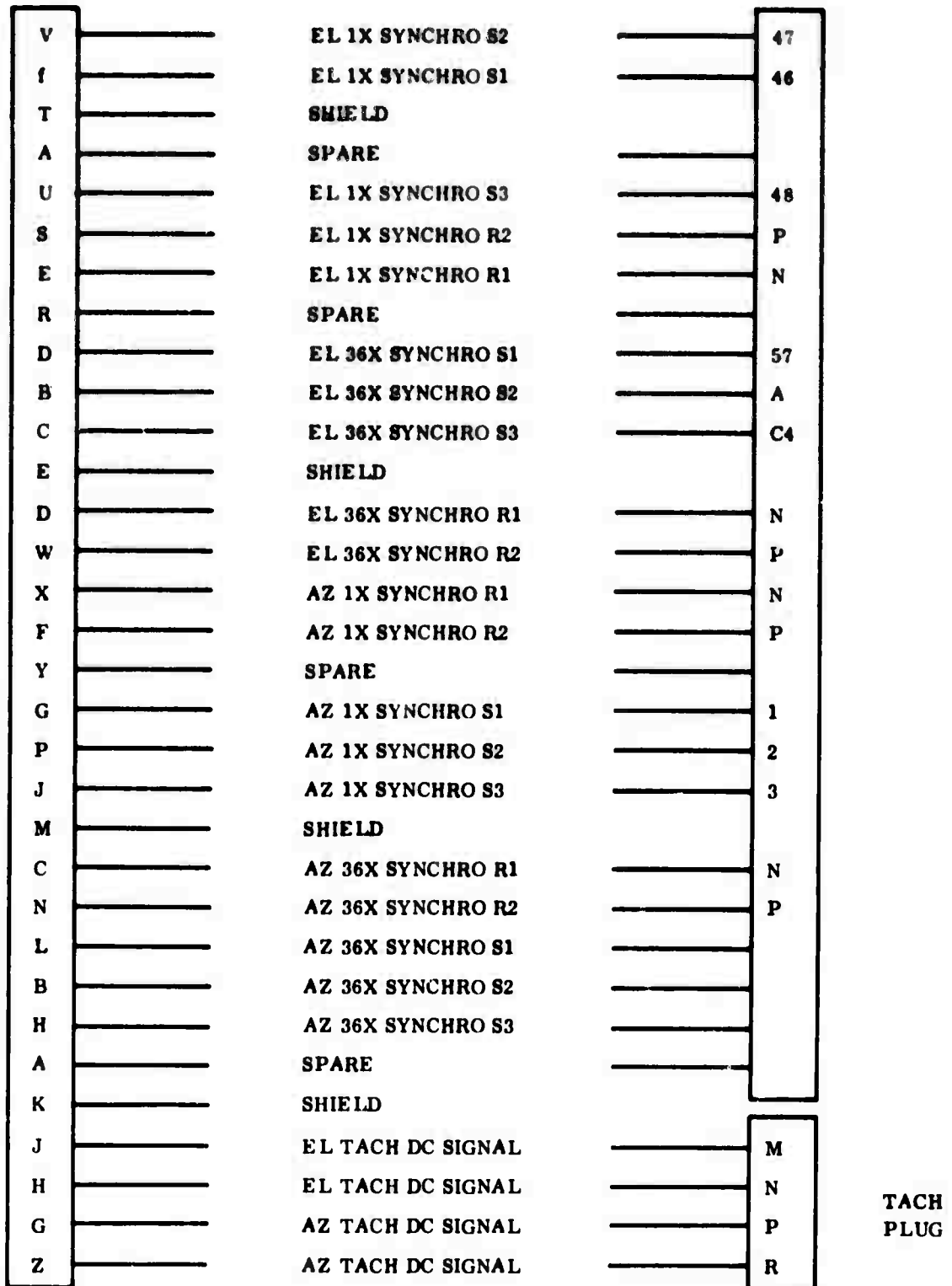
Figure 8-8. Synchro Plug to Azimuth Control Box Wiring Diagram
