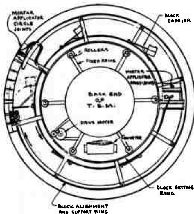
CONTINUOUS BLOCK SETTING MACHINE
