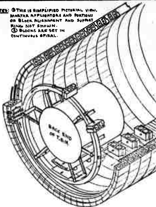
CONTINUOUS BLOCK SETTING MACHINE
