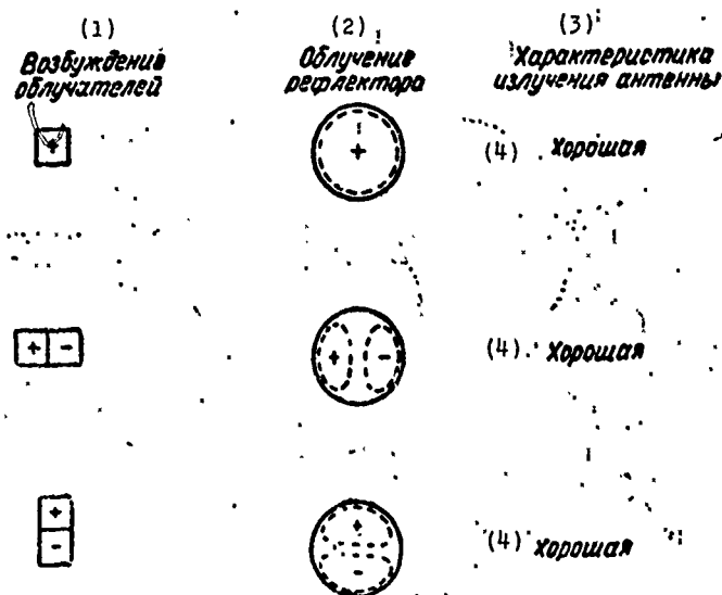
Fig. 2.28. Optimal irradiation in the antenna of a monopulse radar. KEY: (1) Excitation of irradiator; (2) Irradiation of reflector; (3) Characteristic of antenna radiation; (4) Good.
