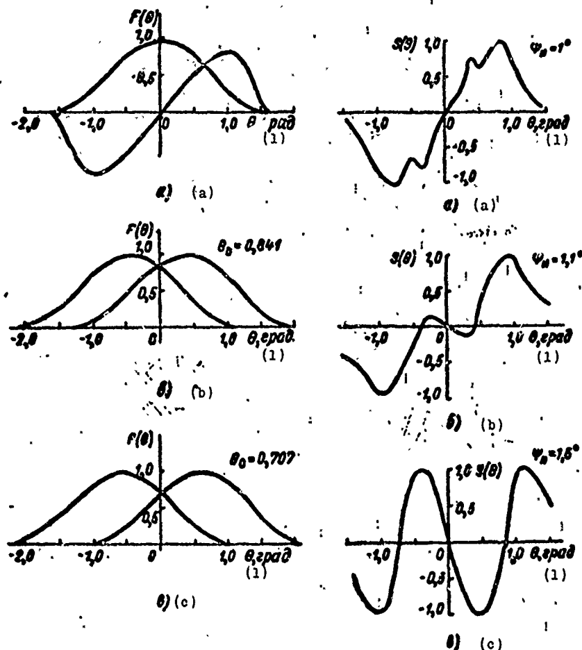
Fig. 4.6. Radiation pattern for compared coordinate system: a) a monopulse system; b) a system with dual switching of antenna radiation patterns; c) a system with conical beam scanning; d) a system with sequential switching of antenna radiation patterns.
