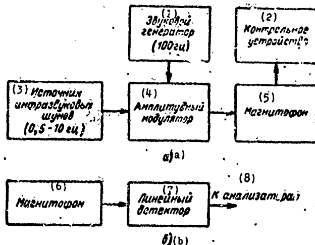
Fig. 5.11. Block diagram of installation: a) for recording subsonic noises; b) for reproducing them.
