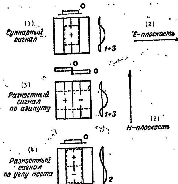
Fig. 2.30. Excitation of a four-horn irradiator operating on the highest types of waves. KEY: (1) Sum signal; (2) Plane; (3) Difference signal for azimuth; (4) Difference signal for elevation.
