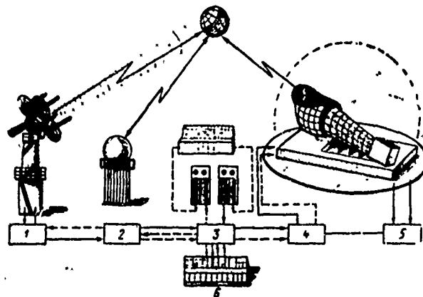
Fig. 9.6. Functional diagram of ground equipment. 1 - coarse guidance station; 2 - precise guidance station; 3 - computer; 4 - antenna of automatic tracking station; 5 - autotracking system; 6 - control panel.
