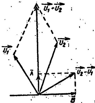
Fig. 1.20. Vector diagram illustrating the principle of a combined direction finding system: A - is the in-phase component of the difference signal (elevation error); B is the quadrature-phase component of the difference signal (azimuth error).
