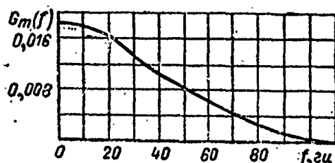
Fig. 5.6. Fluctuations spectrum for signals reflected from ship.
