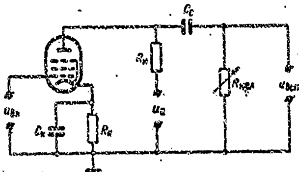
Fig. 3.2. Simplified diagram of a stage with a nonlinear element.
