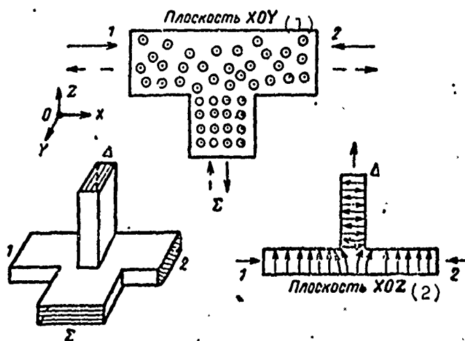
Fig. 2.37. Double waveguide T-joint KEY: (1) Plane XDY; (2) Plane XOZ.
