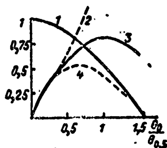
Fig. 2.34. Dependence of relative values on separation angle: 1) F_c(0) ; 2) F'_p(0)/F_c(0) ; 3) F'_p(0) ; 4) F_c(0)F'_p(0) .
