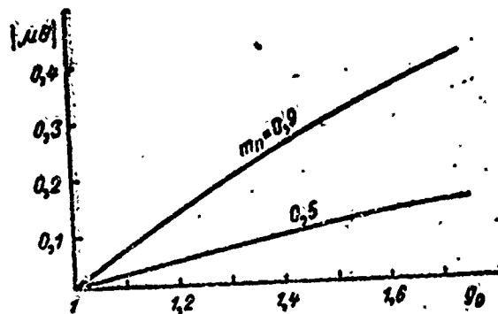
Fig. 7.4. Dependence of generalized systematic direction finding error on the value of nonidentity of transmission factors for receiving channels under the effect of amplitude-modulated noise on switching frequency.
