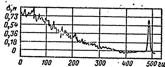
Fig. 5.14. Sample of recording of typical angular noise spectrum from aircraft.
