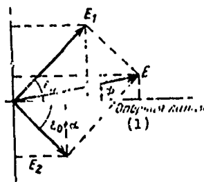
Fig. 5.8. Vector diagram of signals received from a two-point source. KEY: (1) Reference line.
