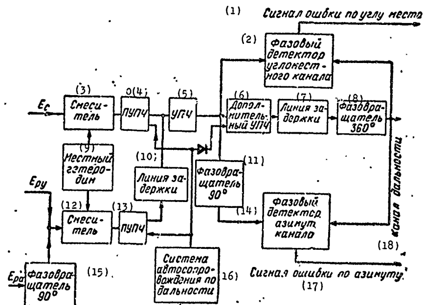
Fig. 6.14. Simplified block diagram of a receiver in an amplitude sum-difference monopulse radar with interconnection of range-measuring and angle-measuring channels on intermediate frequency with the use of phase shifts and time delay of signals. E_c sum signal; E_p difference signal of elevation channels; E_p a difference signal of azimuth channel.
