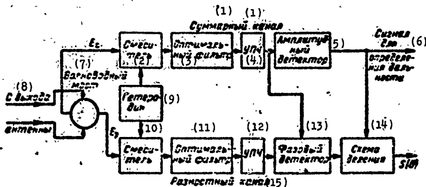
Fig. 1.13. Block diagram of an amplitude sum-difference monopulse scanning system for determining coordinates in one plane.
