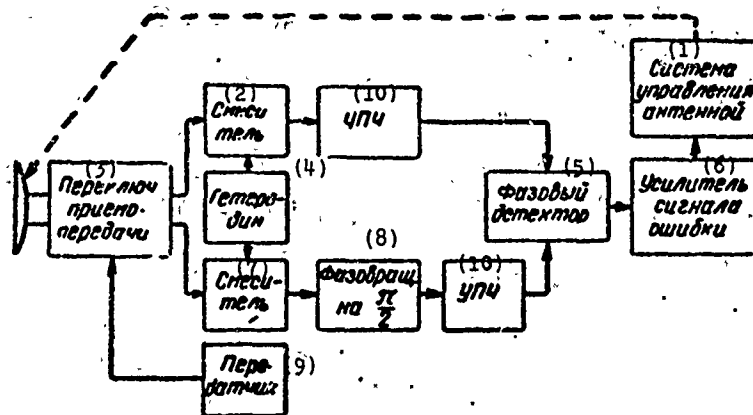
Fig. 1.8. Block diagram of phase-phase monopulse system for tracking a target in one plane.
