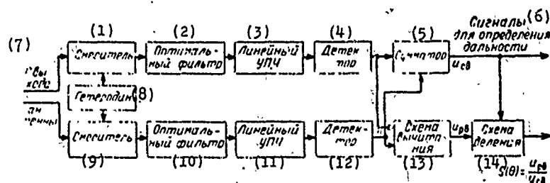
Fig. 1.12. Block diagram of amplitude-amplitude monopulse scanning system for determining coordinates in one plane.
