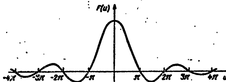
Fig. 2.2. Antenna radiation pattern in the case of uniform field distribution in the aperture.
