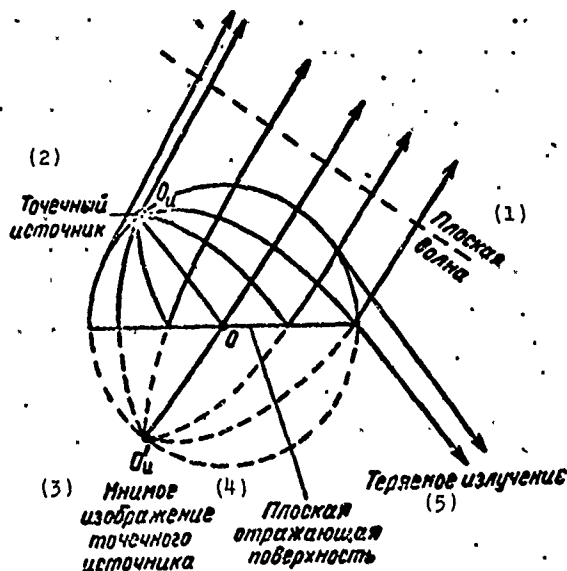
Fig. 2.15. Luneberg hemispherical lens.
