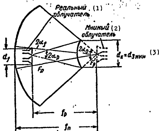
Fig. 2.10. Minimum shading of primary radiator. KEY: (1) Actual feed; (2) Imaginary feed; (3) d_k = d_3 \text{ min} .
