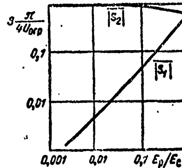
Fig. 6.18. Standardized calculated dependence of signal amplitude at band-pass filter output on the amplitude ratio of difference and sum signals at input of an ideal limiter.
