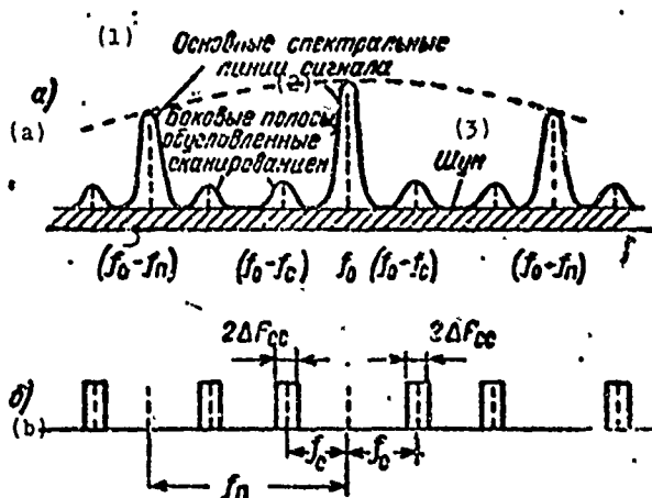
Fig. 5.17. Passage of signal and noise in radar with conical scanning: a) elements of spectrum of signal and noise; b) bandwidth of servosystem.
