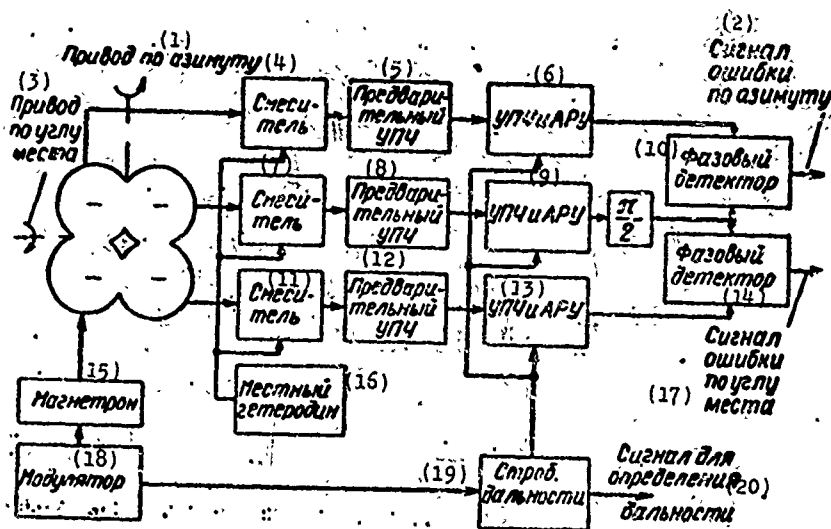
Fig. 1.15. Block diagram of a phase-phase monopulse system for direction finding in two planes.
