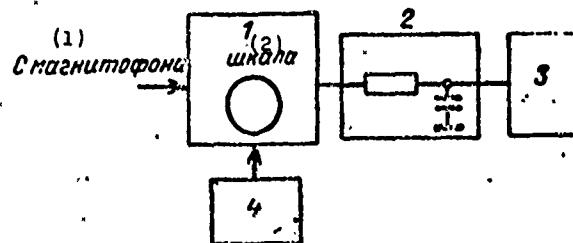
Fig. 5.12. Block diagram of equipment for analyzing noise power spectrum distribution: 1 - main spectral analyzer; 2 - integrator ( R = 20 \text{ k}\Omega , C = 50 \text{ }\mu\text{F} ); 3 - recorder; 4 - cam drive of analyzer for linear scan.
