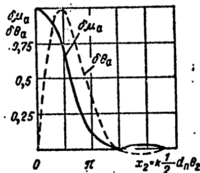
Fig. 4.4. Variation and direction finding sensitivity \delta\mu_a and angular direction finding error \delta\theta_a of an amplitude sum-difference monopulse radar because of interfering target.
