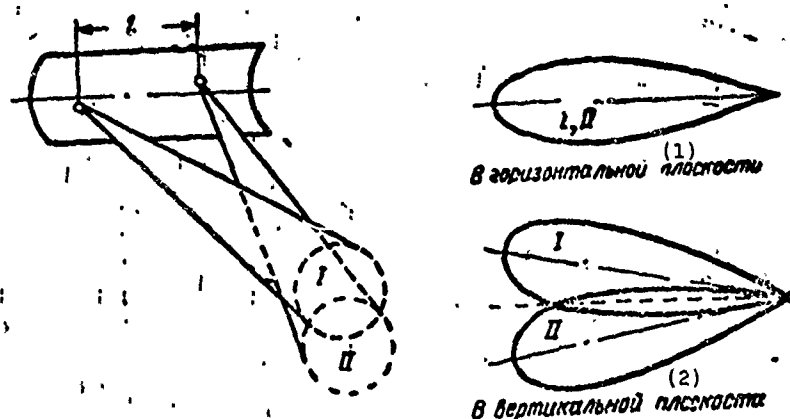
Fig. 1.21. The principle of forming radiation patterns and combined monopulse systems.
