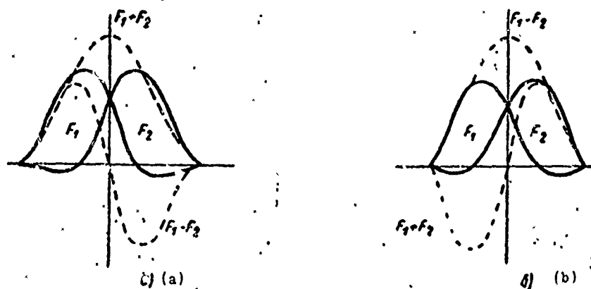
Fig. 6.8. Radiation patterns for difference and sum channels: a) when \psi = 0 ; b) when \psi = \pi .
