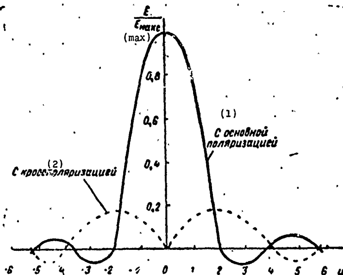
Fig. 2.19. Radiation pattern of a mirror antenna irradiated by an electrical dipole.
