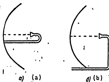
Fig. 2.5. Methods of attaching feeds to parabolic antennas.
