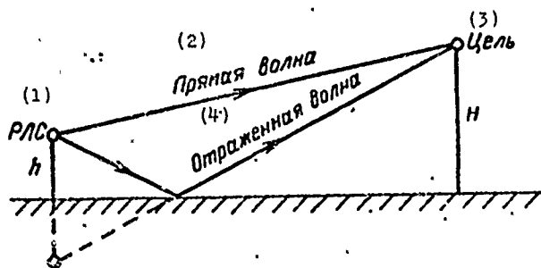
Fig. 5.1. Radio wave propagation over a flat reflecting surface. KEY: (1) Radar; (2) Direct wave; (3) Target; (4) Reflected wave.
