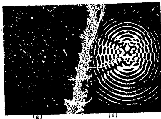
Fig. 5.9.. Phase front of waves radiated by a two-point source: a) calculated; b) experimental.
