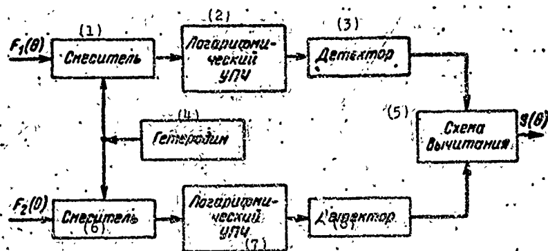
Fig. 1.4. Block diagram of an amplitude angular discriminator.
