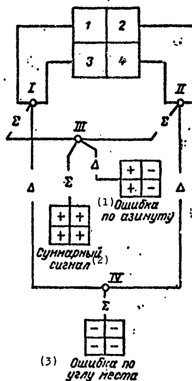
Fig. 2.26. Excitation diagram of a four-horn irradiator.
