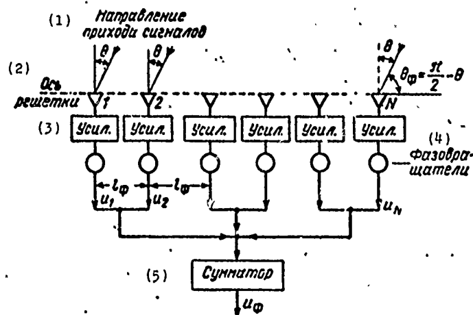
Fig. 2.22. Diagram of a phased array.
