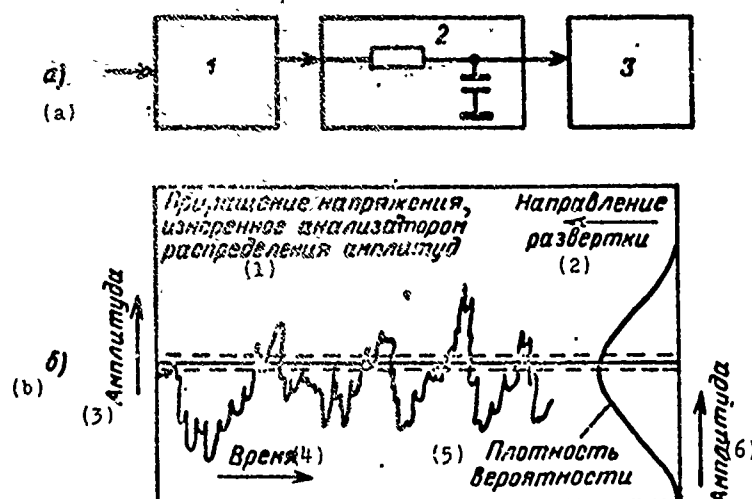
Fig. 5.13. Block diagram of the installation for analyzing amplitude distribution (a) and a sample of the working graph (b): 1 - amplitude distribution analyzer; 2 - integrator ( R = 100 \text{ k}\Omega , C = 50 \text{ }\mu\text{F} ); 3 - recorder.
