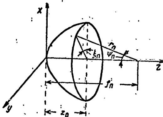
Fig. 2.16. System of coordinates for determining field in paraboloid aperture.
