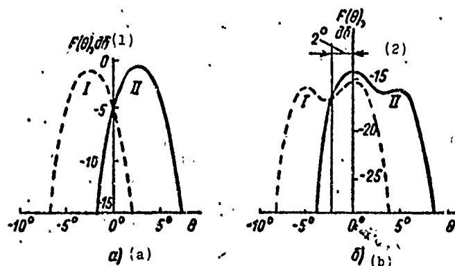
Fig. 5.26. Antenna radiation pattern on an amplitude sum-difference monopulse system: a) for main polarization; b) for crosspolarization. KEY: (1) F(\theta) , dB; (2) F(\theta) , dB.
