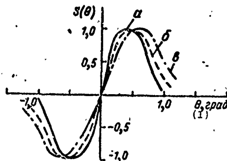
Fig. 4.11. Standardized direction finding characteristics of radars during the direction finding of a point source: a) monopulse systems; b) system with sequential and dual switching of antenna patterns; c) system with conical scanning. KEY: (1) deg.
