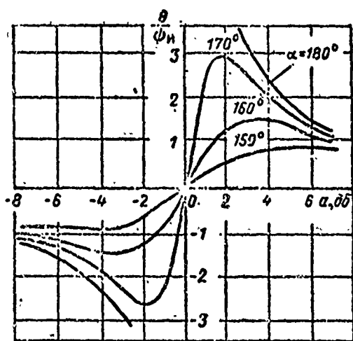
Fig. 7.7. Dependence of relative angular direction finding error for a two-point target on signal ratios for selected values of phase shift.
