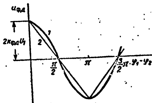
Fig. 3.9. Characteristics of a phase detector: 1 - when U_1 \ll U_2 ; 2 - when U_1 = U_2 .
