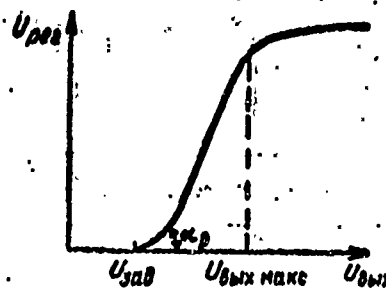
Fig. 3.14. Amplitude characteristic of an AGC circuit.
