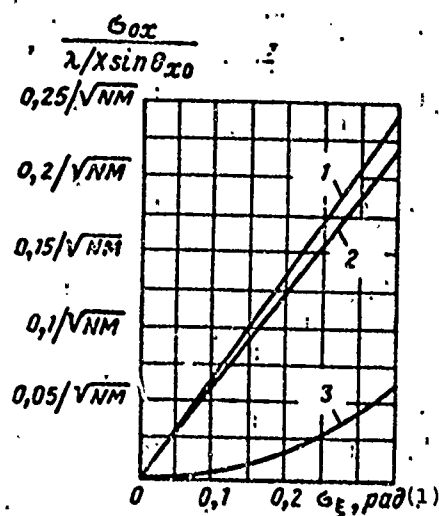
Fig. 6.2. Dependence of standard tracking error on the value of standard phase error in antenna excitation: 1 - sum error; 2 - error from displacement of equisignal direction; 3 - error from change in direction finding sensitivity. KEY: (1) rad.
