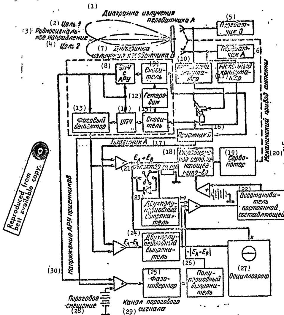
Fig. 4.12. Block diagram of a monopulse radar with high resolution. KEY: (1) Radiation pattern of transmitter A; (2) Target 1; (3) Equisignal direction; (4) Target 2; (5) Transmitter B; (6) Transmitter A; (7) Radiation pattern of transmitter B; (8) I-f amplifier with AGC; (9) Mixer; (10) Antenna switch; (11) Antenna switch; (12) Heterodyne; (13) Phase detector; (14) I-f amplifier; (15) Mixer; (16) Receiver B; (17) Receiver A; (18) Gated storage device; (19) Servomotor; (20) Mechanical antenna drive; (21) Target selector; (22) D-C restorer; (23) Full-wave rectifier; (24) Full-wave rectifier; (25) Phase inverter; (26) Wave rectifier; (27) Oscillograph; (28) Threshold bias; (29) Threshold signal channel; (30) Direction AGC receiver.
