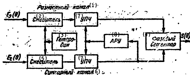
Fig. 1.6. Block diagram of sum-difference angular discriminator. KEY: (1) Difference channel; (2) Mixer; (3) Heterodyne; (4) Phase Detector; (5) Mixer; (6) Sum channel; (7) I-f amplifier; (8) AGC.
