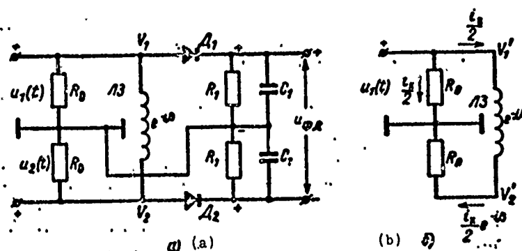
Fig. 3.10. The Kirkpatrick phase detector: a - simplified detector circuit; b - part of circuit illustrating the formation of voltages acting on diodes.
