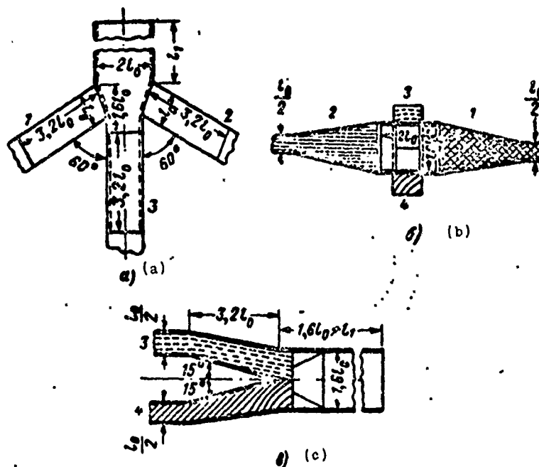
Fig. 2.33. Overall view of a one-horn irradiator: a) top view; b) front view; c) vertical cross-section along the axis of symmetry; 1 - left side arm; 2 - right side arm; 3 - upper arm; 4 - lower arm.
