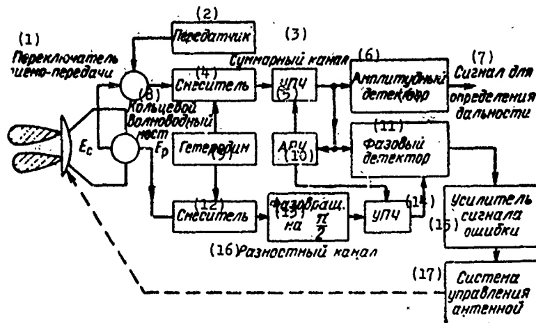
Fig. 1.11. Block diagram of a phase sum-difference monopulse system of target tracking in one plane.
