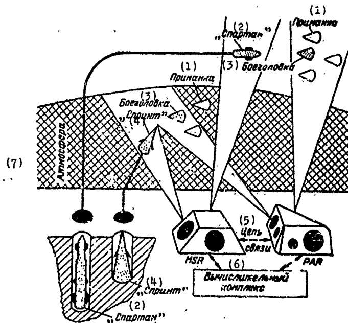
Fig. 9.14. Elements of the "limited" ABM system, the Safeguard.
