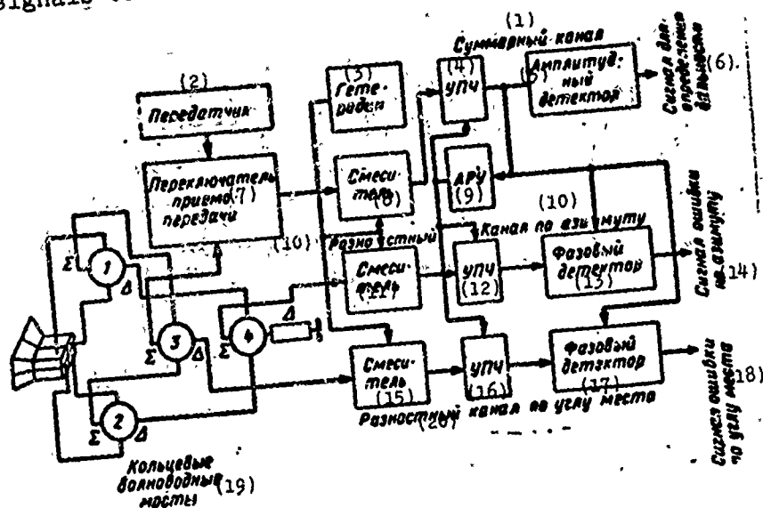
Fig. 1.16. Block diagram of an amplitude sum-difference monopulse system for direction finding in two planes. \Sigma - sum output of bridge; \Delta - difference output of bridge. KEY: (1) Sum channel; (2) Transmitter; (3) Heterodyne; (4) I-f amplifier; (5) Amplitude detector; (6) Signals for determining range; (7) Send-receive switch; (8) Mixer; (9) AGC; (10) Difference channel for azimuth; (11) Mixer; (12) I-f amplifier; (13) Phase detector; (14) Azimuth error signal; (15) Mixer; (16) I-f amplifier; (17) Phase detector; (18) Elevation error signal; (19) Annular waveguide bridges; (20) Difference channels for elevation.
