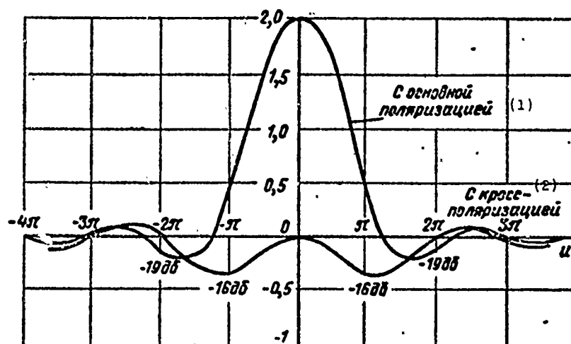
Fig. 2.21. Calculated radiation pattern of a square horn with circular polarization.
