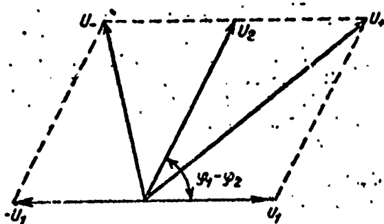
Fig. 3.8. Vector diagram of voltages for phase detector.
