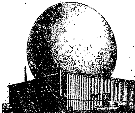
Fig. 9.4. Antenna dome for AN/FPS-49 radar.
