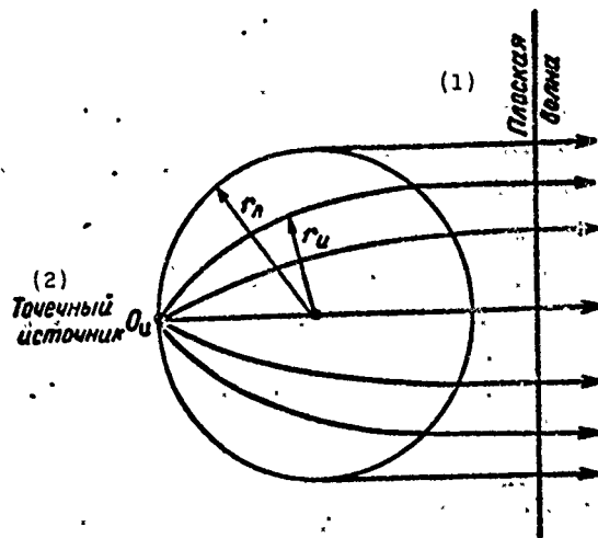
Fig. 2.14. Spherical Luneberg lens.
