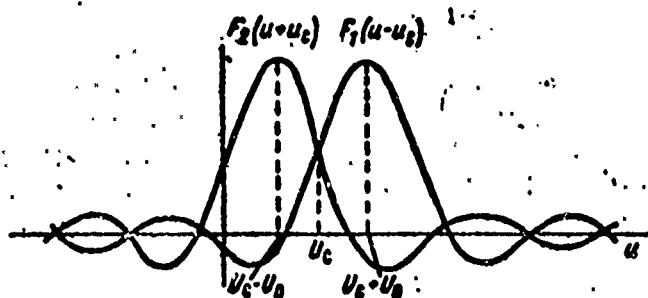
Fig. 2.3. Antenna radiation patterns with displaced equisignal direction.
