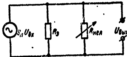
Fig. 3.4. Equivalent circuit of a nonlinear resonance stage.
