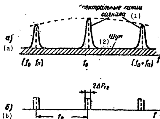
Fig. 5.16. Passage of signal and noise in monopulse radar: a) elements of the spectrum of signal and noise; b) servosystem bandwidth.
