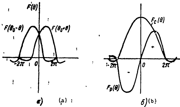
Fig. 1.10. Radiation pattern of an amplitude sum-difference monopulse system with direction finding in one plane: a) partial patterns; b) sum and difference patterns.
