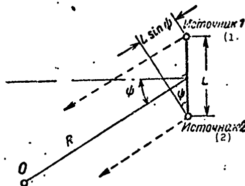
Fig. 5.7. Geometric relationships of a two-point signal source. KEY: (1) Source 1; (2) Source 2.
