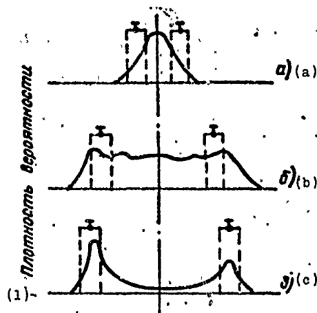
Fig. 4.10. Distribution of antenna direction probability during the tracking of two targets with different angular distances: a) \psi_n = 0.3 \theta_{0.5} ; b) \psi_n = 0.75 \theta_{0.5} ; c) \psi_n = 0.85 \theta_{0.5} .
