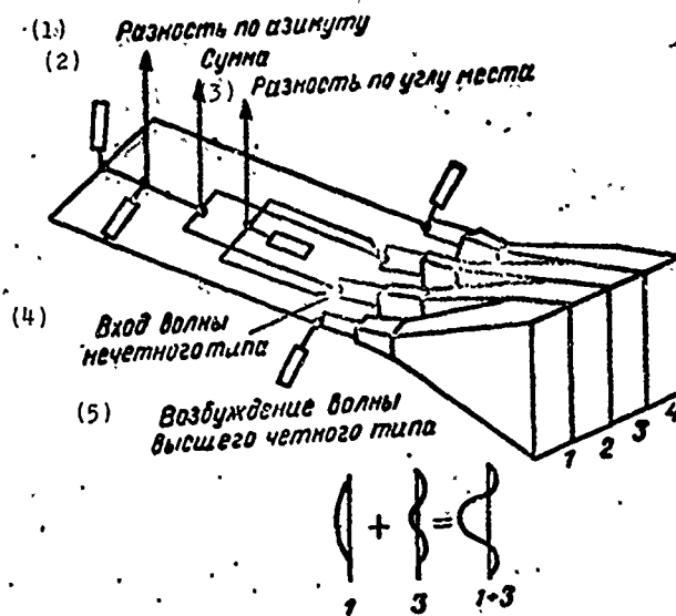
Fig. 2.29. A four-horn irradiator operating on several types of waves. KEY: (1) Azimuth difference; (2) Sum; (3) Elevation difference; (4) Input of uneven wave; (5) Excitation of highest even wave.
