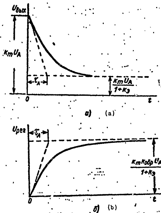
Fig. 3.17. Transition characteristics of an AGC system when the input signal acts intermittently.
