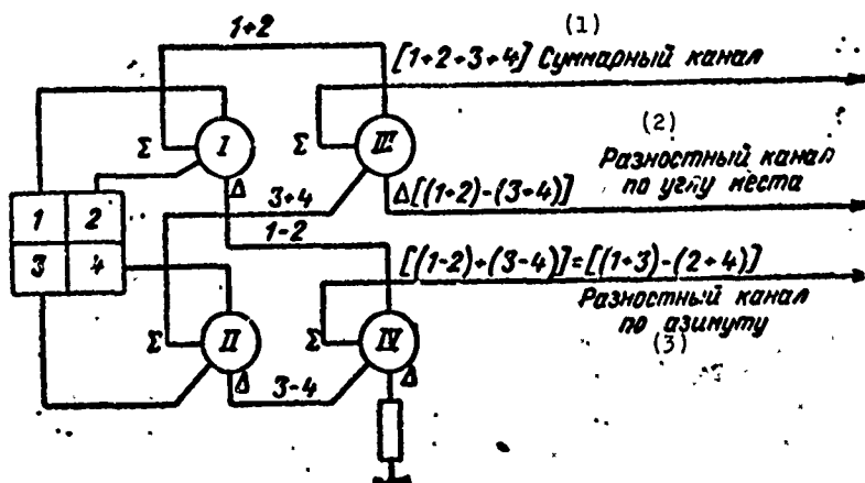
Fig. 1.17. Diagram for forming sum and difference signals with the use of four waveguide bridges. Σ - sum output of bridge; Δ - difference output of bridge.
