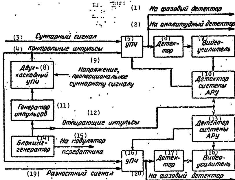
Fig. 3.18. Block diagram of an AGC system and an amplitude sum-difference monopulse radar. KEY: (1) Phase detector; (2) To amplitude detector; (3) Sum signal; (4) Reference pulses; (5) I-f amplifier; (6) Detector; (7) Video amplifier; (8) Two-stage i-f amplifier; (9) Voltage proportional to sum signal; (10) Detector of AGC system; (11) Pulse oscillator; (12) Trigger pulse; (13) Detector of AGC system; (14) Blocking oscillator; (15) To modulator transmitter; (16) I-f amplifier; (17) Detector; (18) Video amplifier; (19) Difference signal; (20) To phase detector.
