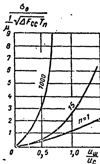
Fig. 5.18. The dependence of error in automatic tracking on the gating factor.
