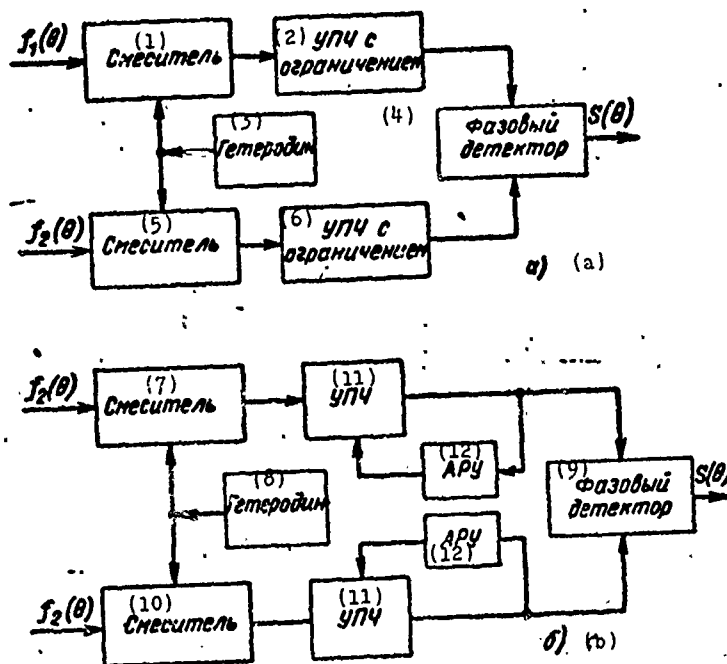
Fig. 1.5. Block diagram of a phase angular discriminator with different methods of normalization, limiting (a) and AGC (b).
