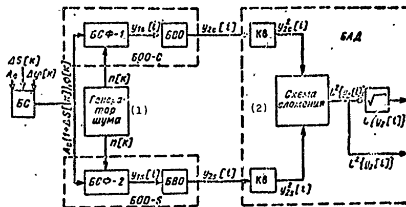
Fig. 8.2. Block diagram of a model of one receiving channel in a scanning monopulse radar.
