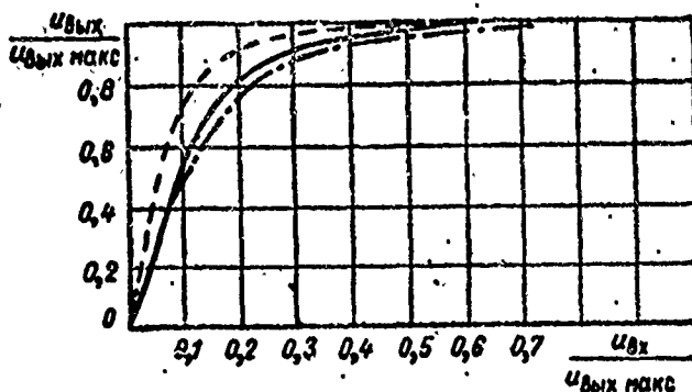
Fig. 3.6. Theoretical amplitude characteristics of a stage. - - - k_1 = 10 , n = 5 ; — k_1 = 5 , n = 5 ; -.- k_1 = 5 , n = 4 .
