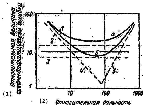
Fig. 5.20. Dependence of standard errors in automatic tracking on target range: 1 - sum error of radar with conical scanning (a) and monopulse radar (b); 2 - errors from amplitude fluctuations; 3 - errors of servosystem; 4 - errors from displacement of reflection center; 5 - errors from receiver noises. KEY: (1) Relative value of standard error; (2) Relative range.
