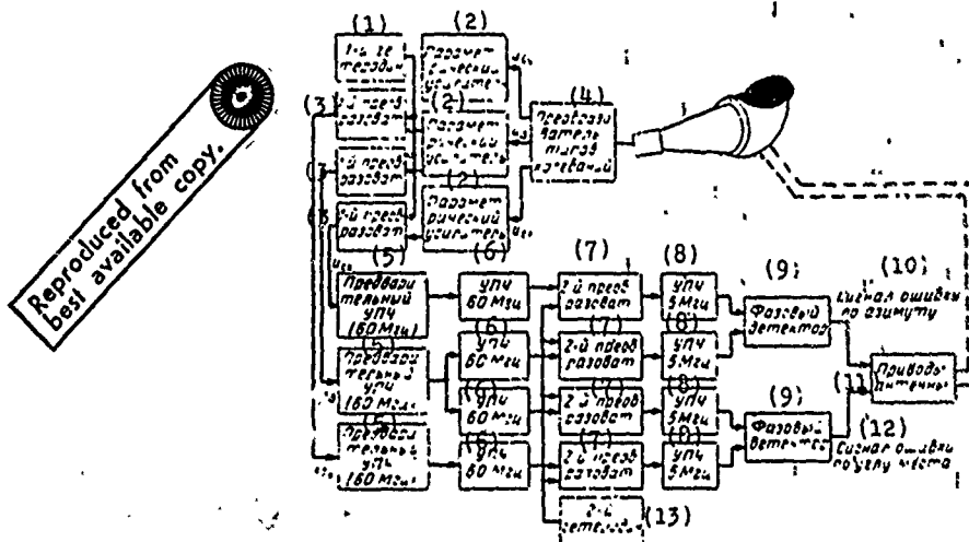
Fig. 9.11. Block diagram of an automatic tracking station. KEY: (1) 1st heterodyne; (2) Parametric amplifier; (3) 1st converter; (4) Converter of types of oscillations; (5) Preliminary i-f amplifier (60 MHz); (6) I-f amplifier 60 MHz; (7) 2nd converter; (8) I-f amplifier 5 MHz; (9) Phase detector; (10) Azimuth error signal; (11) Antenna drive; (12) Elevation error signal; (13) 2nd heterodyne.
