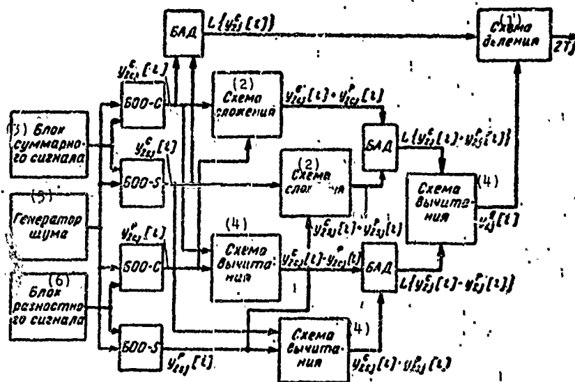
Fig. 8.4. Block diagram of a model of an amplitude sum-difference scanning monopulse radar for determining coordinates in one plane. KEY: (1) Division circuit; (2) Add circuit; (3) Sum signal unit; (4) Subtraction circuit; (5) Noise generator; (6) Difference signal unit.
