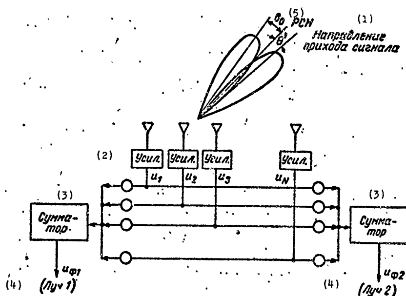
Fig. 2.23. The formation of beams by an antenna array in a monopulse radar with amplitude direction finding. KEY: (1) Direction of signal approach; (2) Ampl.; (3) Summator; (4) Beam; (5) ESD [equisignal direction].
