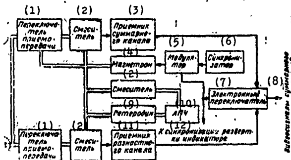
Fig. 9.26. Block diagram of a ground target detection radar. KEY: (1) Send-receive switch; (2) Mixer; (3) Sum channel receiver; (4) Magnetron; (5) Modulator; (6) Synchronizer; (7) Electronic switch; (8) Video signals of sum and difference channels; (9) Heterodyne; (10) ASC; (11) Difference channel receiver; (12) Two indicator sweep synchronization.
