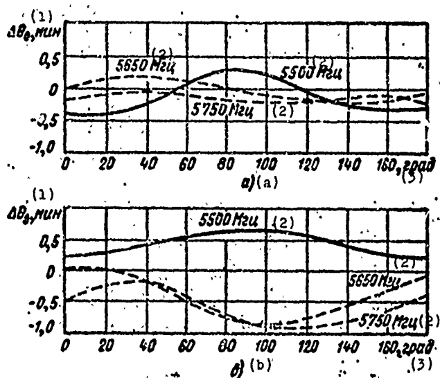
Fig. 5.27. Dependence of equisignal displacement on the angle of slope in the polarization plane of received signals: a) in azimuth; b) in elevation.
