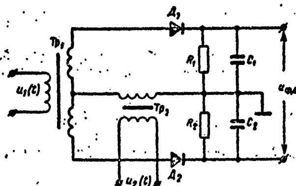
Fig. 3.7. Diagram of a vector measuring balance phase detector.
