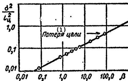
Fig. 5.23. Experimental dependence of standard tracking error on servosystem bandwidth in a radar with low AGC and zero delay error. \beta - ratio of servosystem bandwidth to width of amplitude spectrum of fluctuations at half power.
