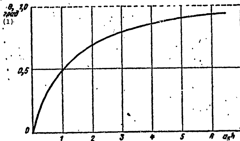
Fig. 5.25. Calculated dependence of the displacement of equisignal direction on the value of a_h b when \theta_{0.5} = 1.0^\circ and \theta_0 = 0.5^\circ .
