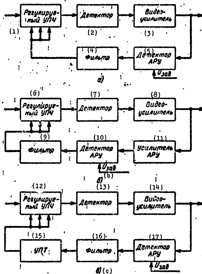
Fig. 3.12. Block diagram of pulse AGC system: a) "unamplified" AGC system; b) "amplified" AGC system with alternate voltage amplification; c) "amplified" AGC system with d-c amplification. KEY: (1) Variable gain i-f amplifier; (2) Detector; (3) Video amplifier; (4) Filter; (5) AGC detector; (6) Variable gain i-f amplifier; (7) Detector; (8) Video amplifier; (9) Filter; (10) AGC detector; (11) AGC amplifier; (12) Variable gain i-f amplifier; (13) Detector; (14) Video amplifier; (15) D-C amplifier; (16) Filter; (17) AGC detector.
