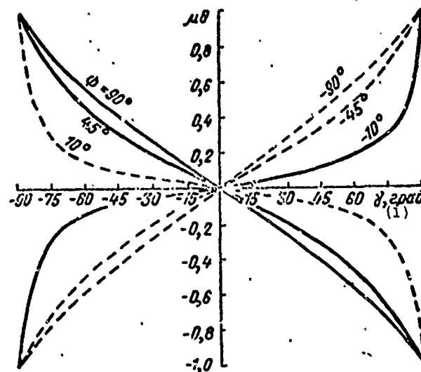
Fig. 6.10. Dependence of generalized direction finding error on value of out-of-phase condition for sum and difference receiving channels calculated with various values for out-of-phase condition of high-frequency channels. KEY: (1) deg.
