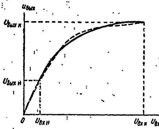
Fig. 3.1. Amplitude characteristic of a logarithmic amplifier. — calculated; - - - experimental.
