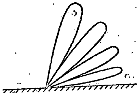
Fig. 5.2. Multilobe antenna radiation pattern caused by the effect of a flat reflecting surface.
