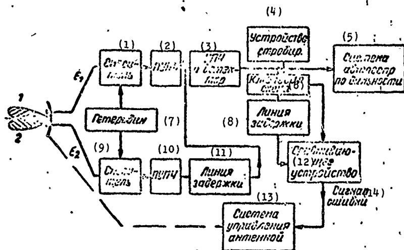
Fig. 6.12. Simplified block diagram of the receiving part of an amplitude-amplitude monopulse radar with interconnection of intermediate-frequency receiving channels. KEY: (1) Mixer; (2) PIFA; (3) I-f amplifier and detector; (4) Gating device; (5) System of automatic range tracking; (6) Key circuit; (7) Heterodyne; (8) Delay line; (9) Mixer; (10) PIFA; (11) Delay line; (12) Comparing device; (13) Antenna control system; (14) Error signal.
