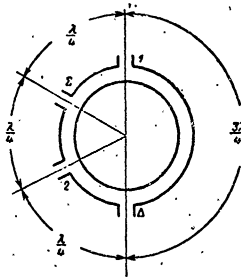
Fig. 2.36. Annular waveguide bridge.
