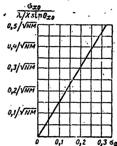
Fig. 6.3. Dependence of standard tracking error on the value of standard amplitude error in antenna excitation.
