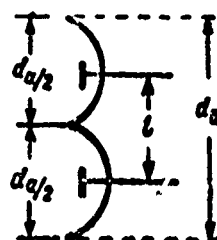
Fig. 2.35. Relationship between separation of irradiators and antenna aperture in a monopulse radar with phase direction finding.
