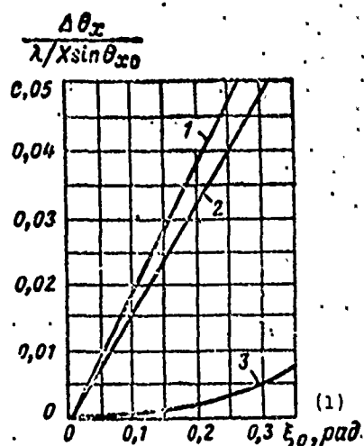
Fig. 6.1. Dependence of standard tracking error on the value of cubic phase antenna excitation error: 1 - sum error; 2 - error from displacement of equisignal direction; 3 - error from change in direction finding sensitivity.
