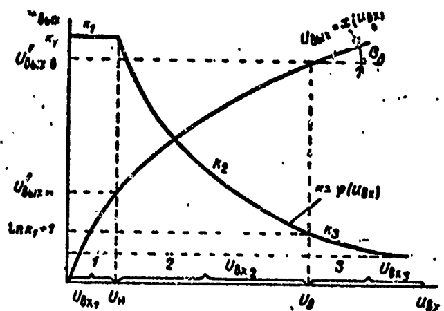
Fig. 3.3. Amplitude characteristic of a nonlinear stage.
