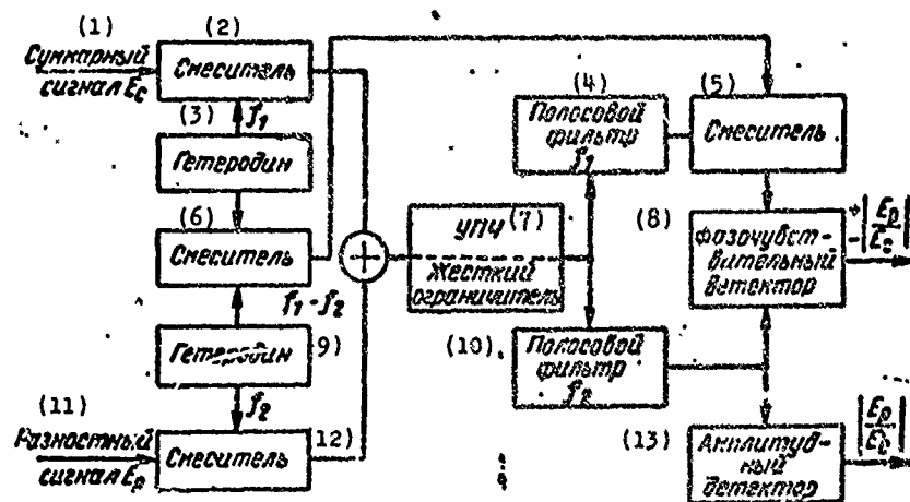
Fig. 6.17. Simplified block diagram of a receiver for an amplitude sum-difference pulse radar with the use of single-channel signal processing with frequency shift.
