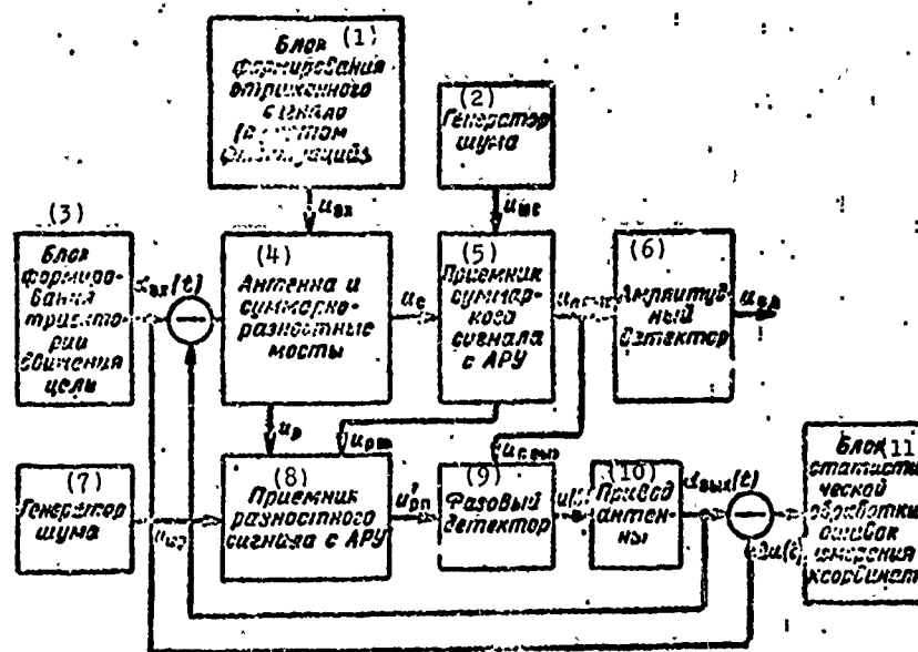
Fig. 8.1. Block diagram of a model of an amplitude sum-difference monopulse tracking radar.
