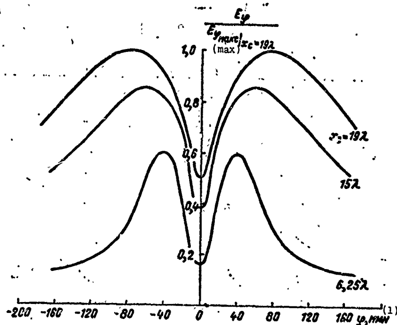
Fig. 2.20. Amplitude radiation patterns in \phi planes for components E_\phi/E_{\phi \text{ max}} when x_c = 19\lambda . KEY: (1) min.
