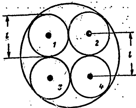
Fig. 2.24. Arrangement of feeds in the antenna system of a monopulse radar with phase direction finding.
