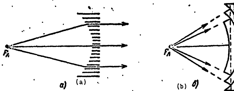
Fig. 2.13. Laminated metal lenses: a) waveguide; b) staggered.
