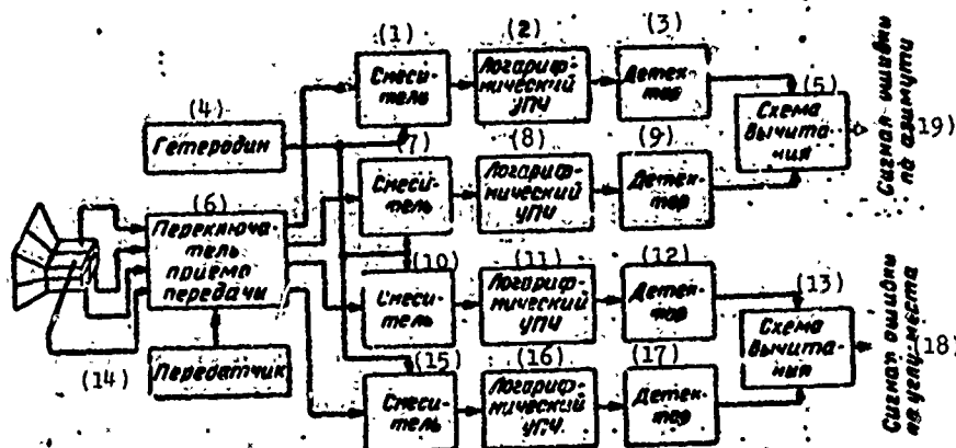
Fig. 1.14. Block diagram of amplitude-amplitude monopulse system for direction finding in two planes.
