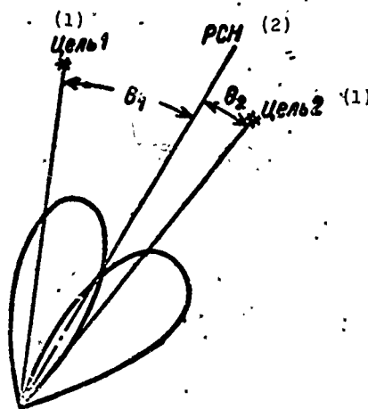
Fig. 4.3. Angles during direction finding of two point targets. KEY: (1) Target; (2) ESD.
