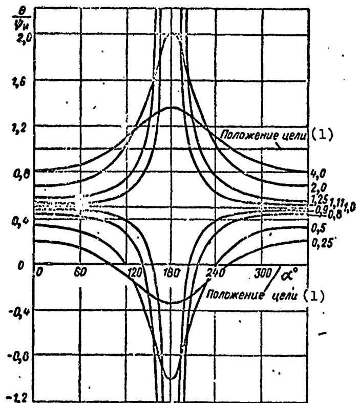
Fig. 7.6. Calculated dependence of angular direction finding errors for a two-point target on amplitude and phase ratios of coherent signals radiated by the target.
