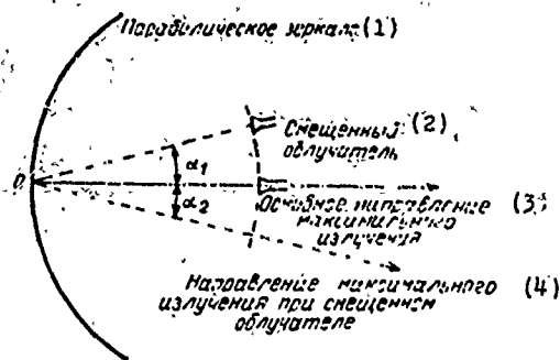
Fig. 2.6. Change in direction of maximum radiation with displacement of feed.
