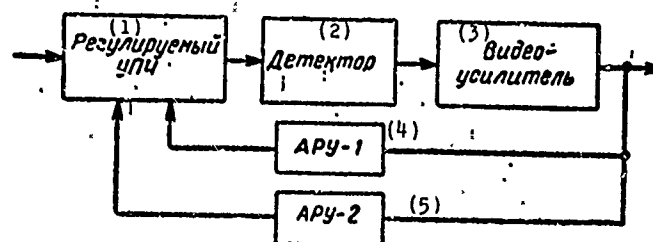
Fig. 3.13. Block diagram of a multiple-loop AGC system. KEY: (1) Variable gain i-f amplifier; (2) Detector; (3) Video amplifier; (4) AGC-1; (5) AGC-2.
