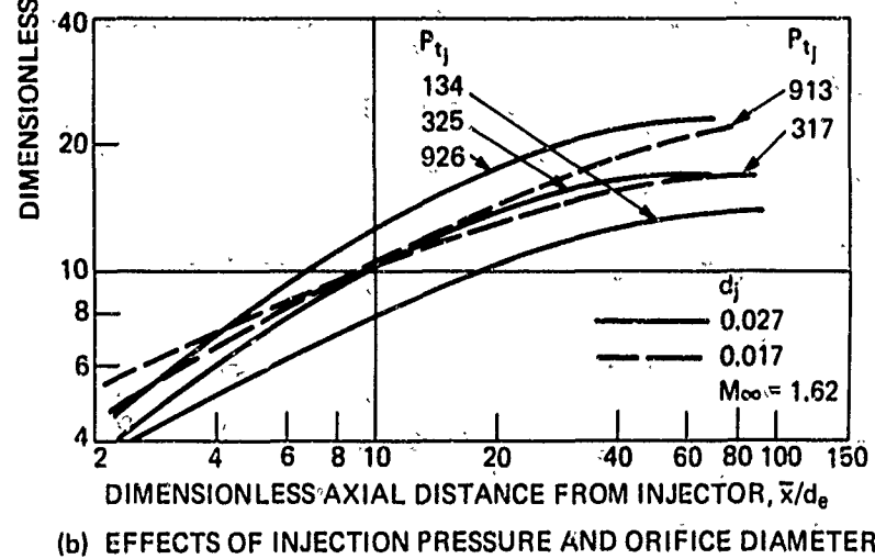
FIGURE 10 TYPICAL JET SPREADING RESULTS.
