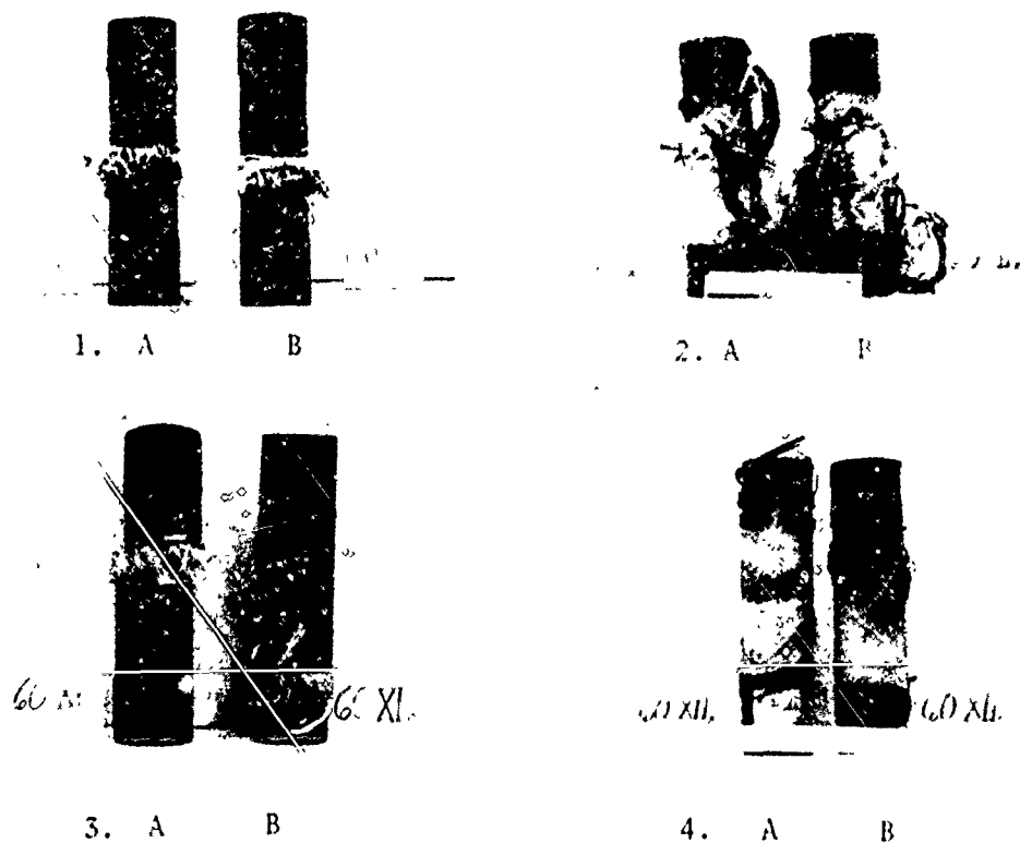
Figure 10 Fiberglass Liner Cylinders After Pressure Testing
