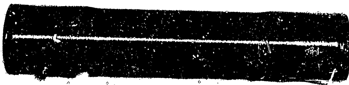
Figure 21 Steel Liner Test Cylinder Before Testing with Strain Gages Attached
