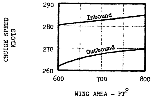
FIGURE 38 WING SIZE TRADE OFF TWO SEGMENT TELESCOPING ROTOR
