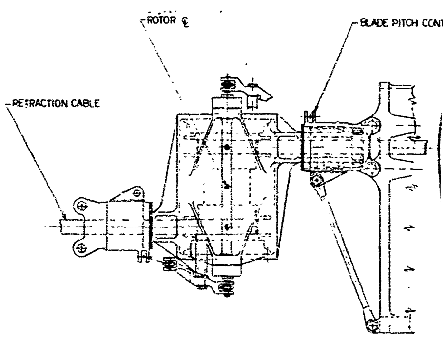
TWO BLADED TEETERING ROTOR HEAD
