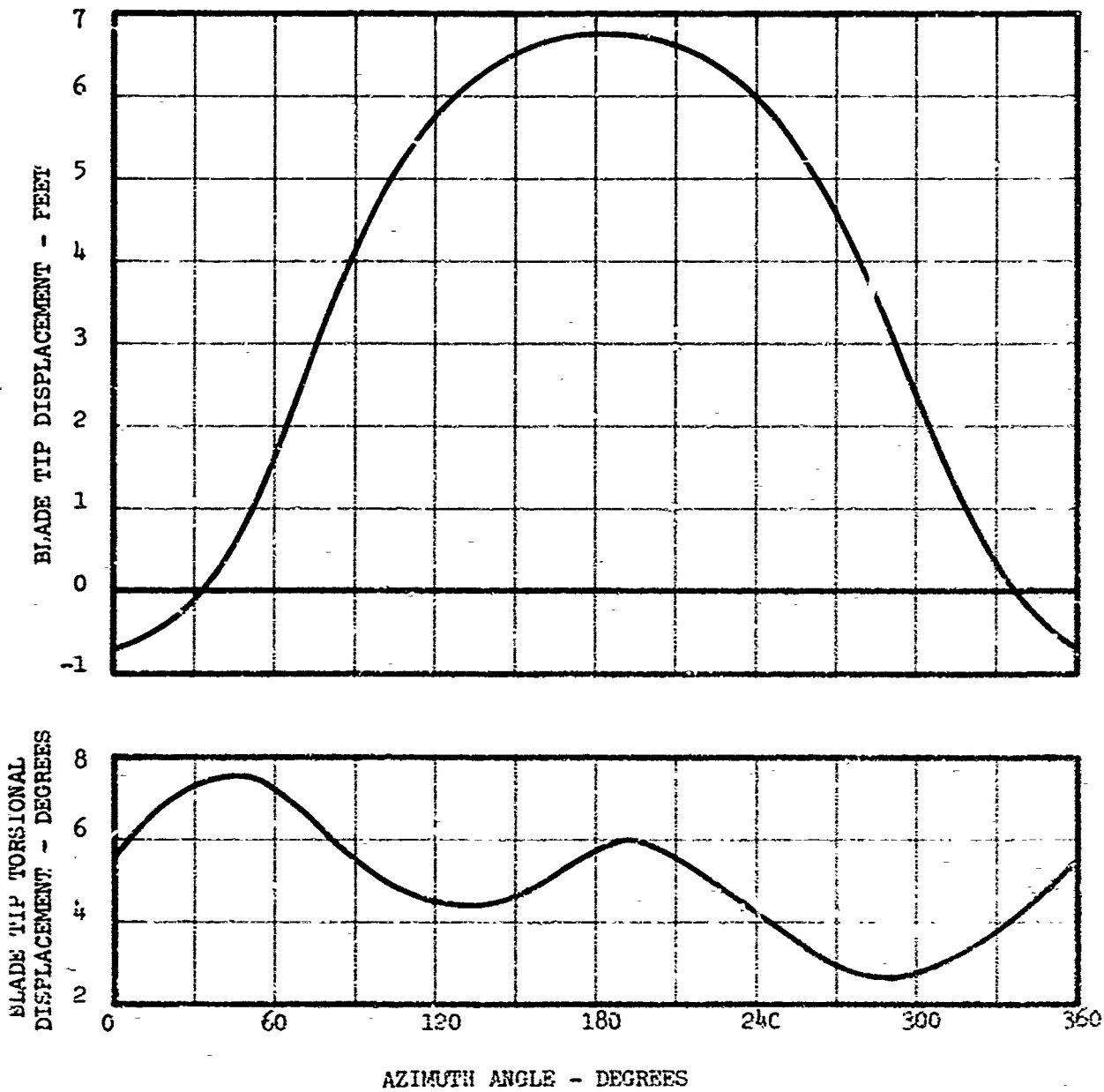
FIGURE 18 ROLL-UP ROTOR FLATWISE AND TORSIONAL RESPONSE AT 100 KNOTS, 36500 LBS LIFT ELASTIC AXIS & MASS AXIS AT 23% CHORD; AERODYNAMIC AXIS AT 25% CHORD BLADE TIP PITCH CONTROL
