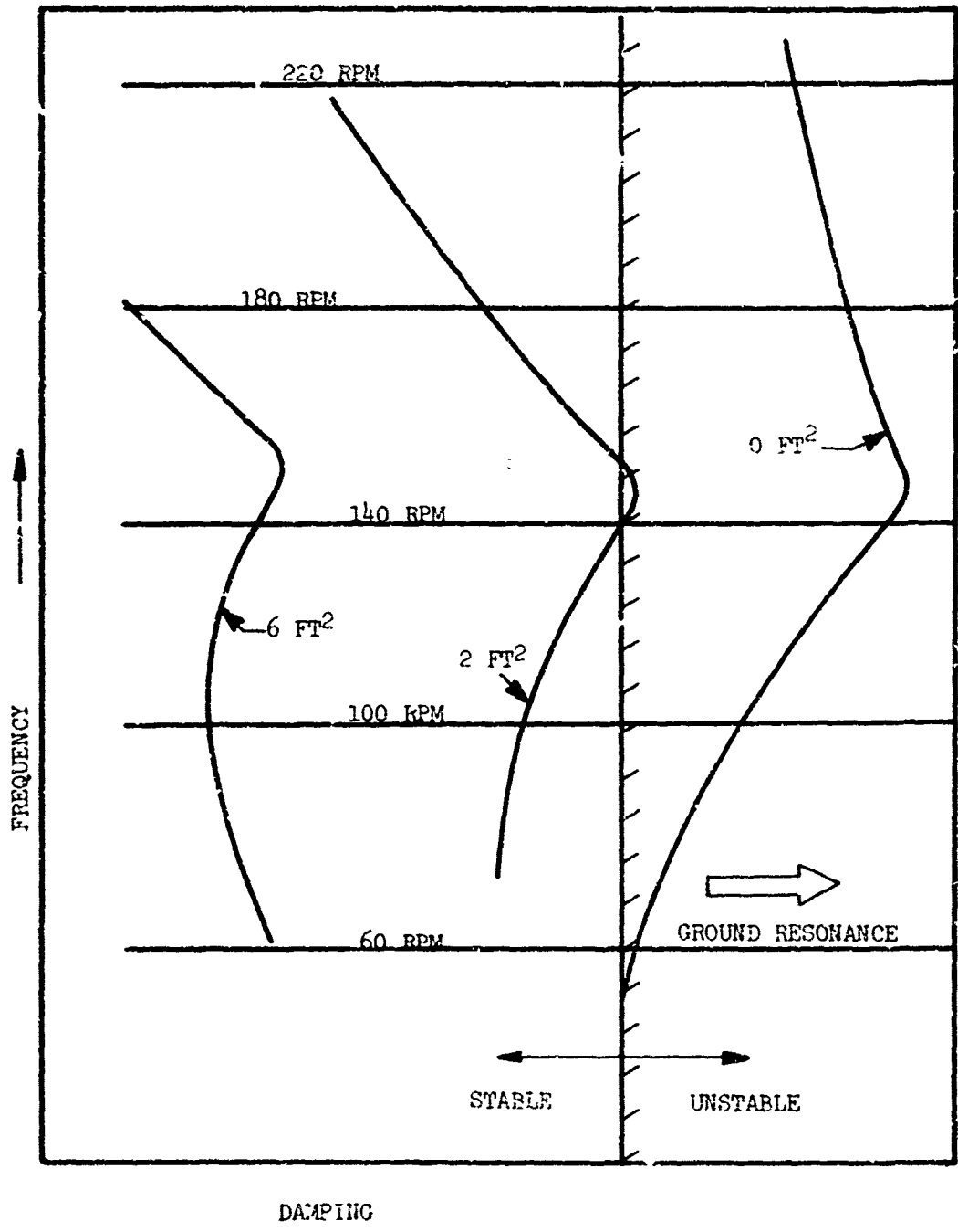
FIGURE 15 ROLL-UP ROTOR EFFECT OF DRAG AREA AND ROTOR SPEED ON STABILITY
