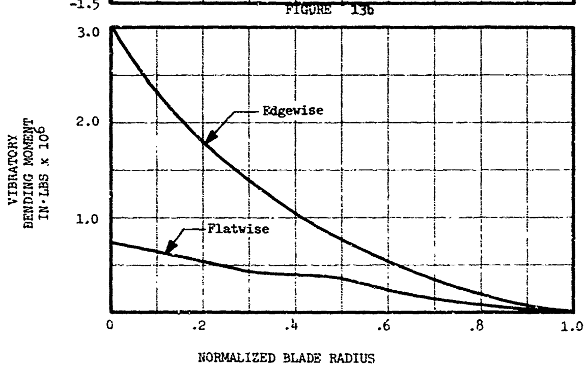
FIGURE 13 EIGHT SEGMENT TELESCOPING ROTOR STEADY AND VIBRATORY BLADE FLATWISE AND EDGEWISE MOMENTS 120 KNOTS, 45000 LBS LIFT
