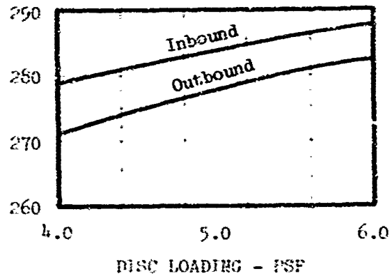
FIGURE 47 DISC LOADING TRADE OFF ROLL-UP ROTOR, FOUR PNEUMATIC BLADES
