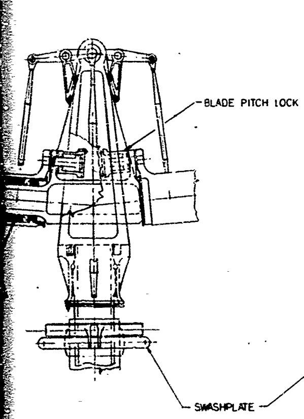
6 TWO BLADED ROTOR HEAD
