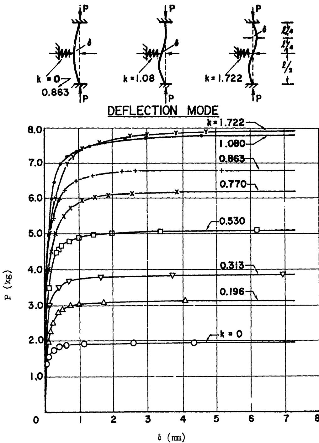
Figure 17. Plots of P vs \delta for the Buckling of Elastically Supported Columns.
