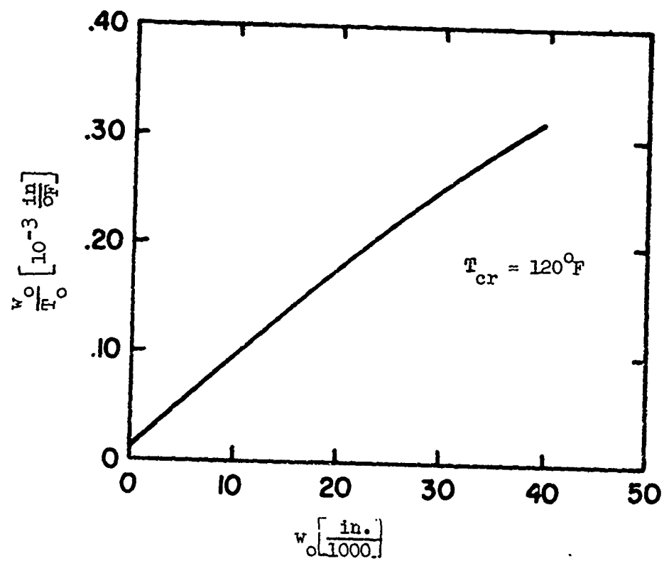
Figure 58. Southwell Plot for Test No. 3 From Reference 40.
