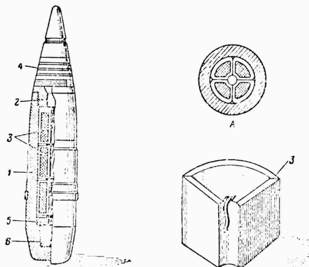
Figure 46. Incendiary shell:
