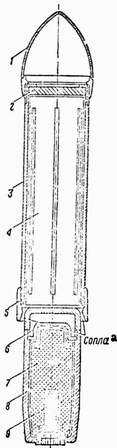
Figure 50. Spin-stabilized projectile:
