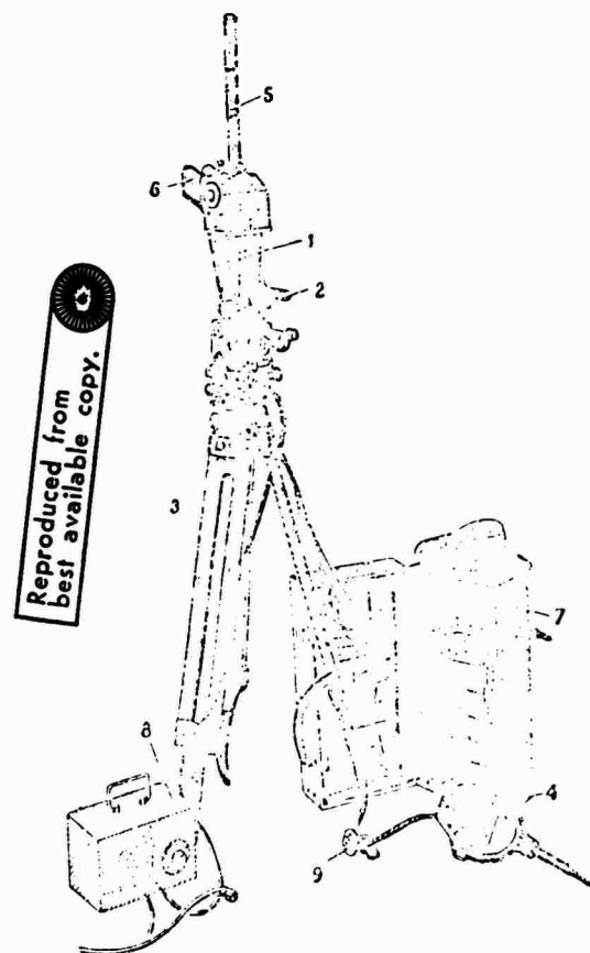
Figure 75. Exploration-theodolite kit:
