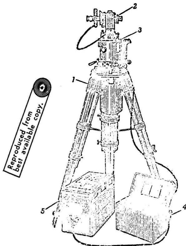
Figure 81. Artillery gyrocompass:
