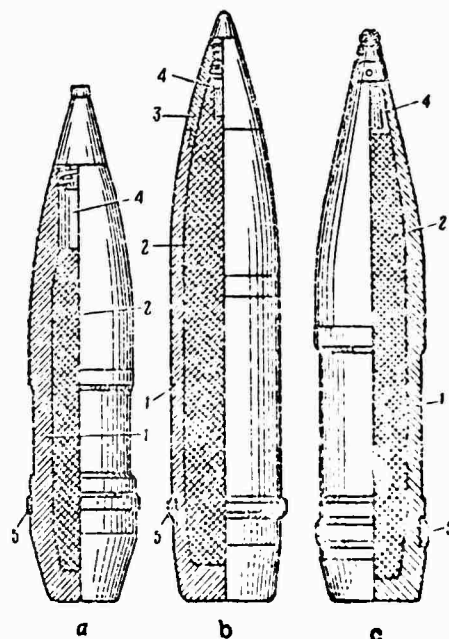
Figure 37. Shells:
