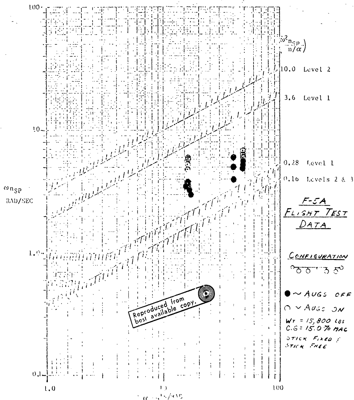
SHORT PERIOD FREQUENCY AND ACCELERATION SENSITIVITY
