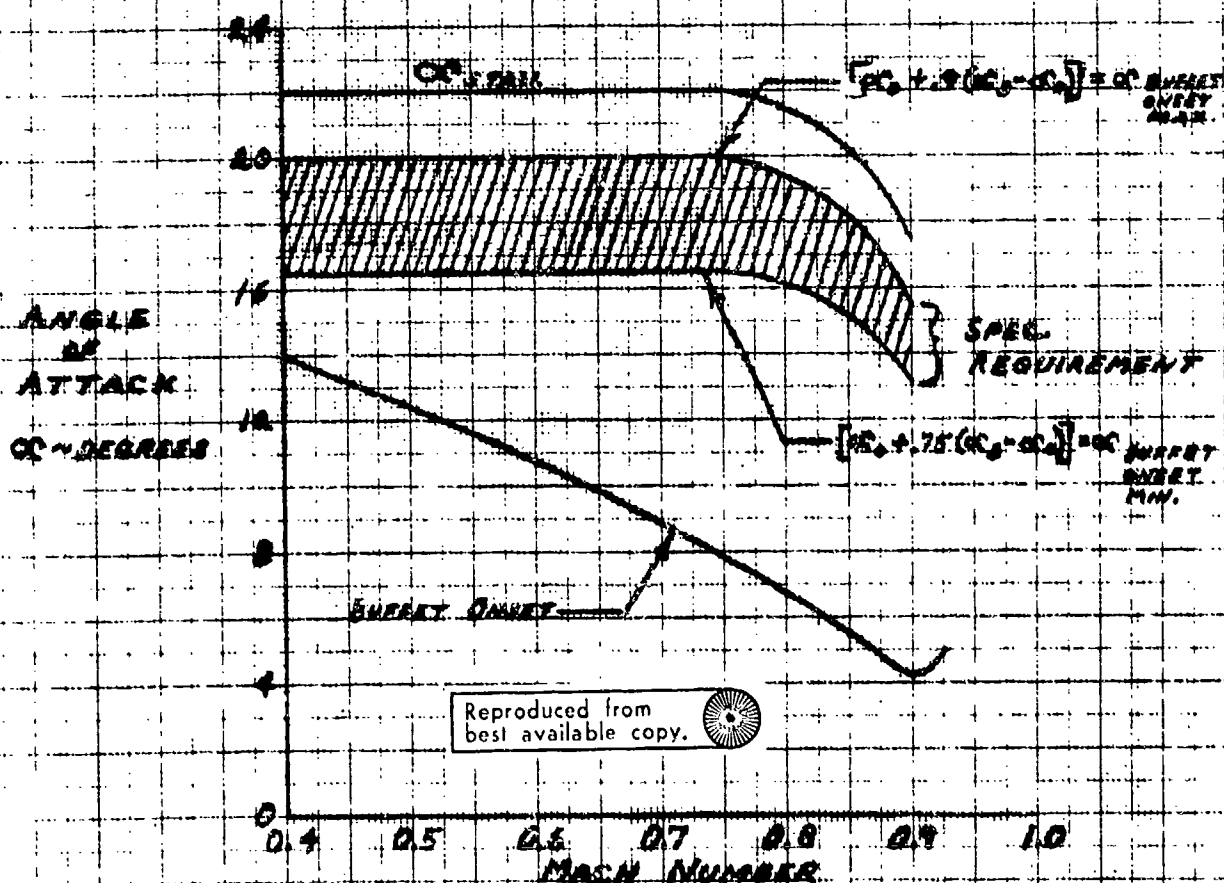
WARNING RANGE FOR ACCELERATED STALLS FIGURE 1 (3.4.2.2.2)
