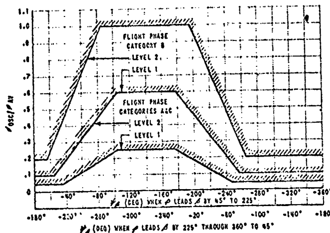
FIGURE 5. Bank Angle Oscillation Limitations
