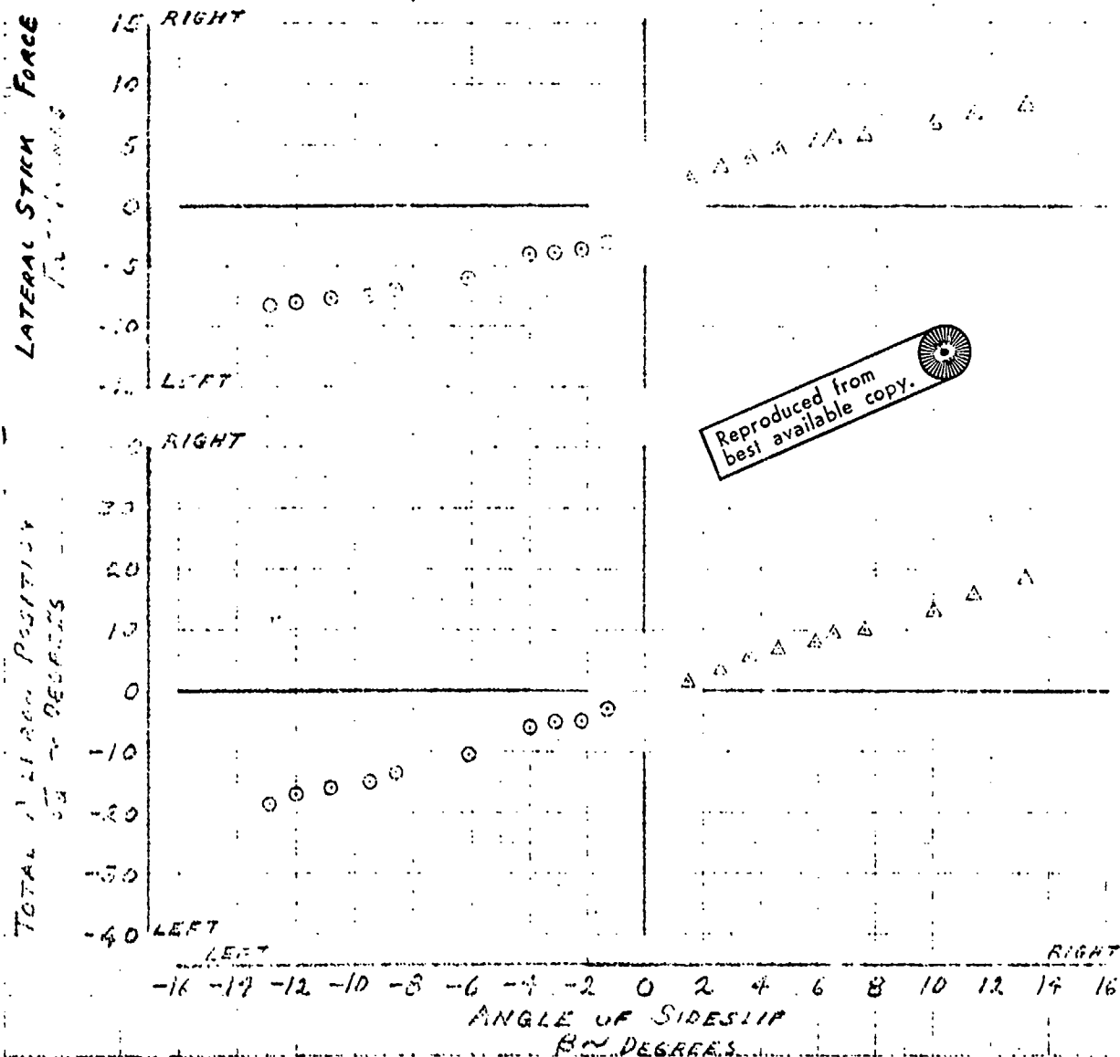
FINAL APPROACH IN CROSS WINDS
