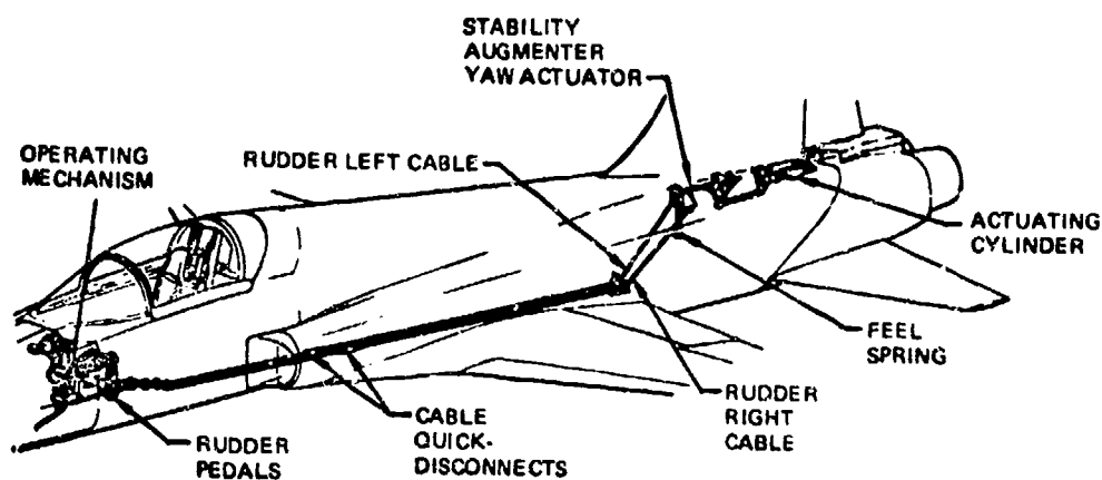
RUDDER CONTROL SYSTEM
