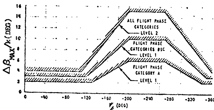
FIGURE 6. Sideslip Excursion Limitations
