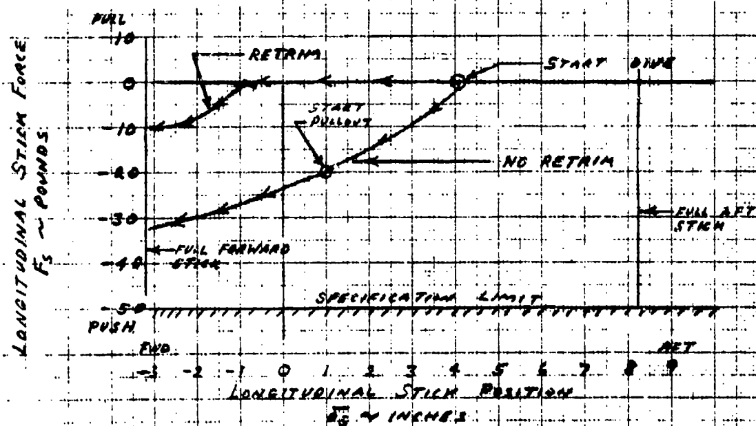
LONGITUDINAL CONTROL FORCES IN DIVES PERMISSIBLE FLIGHT ENVELOPE
