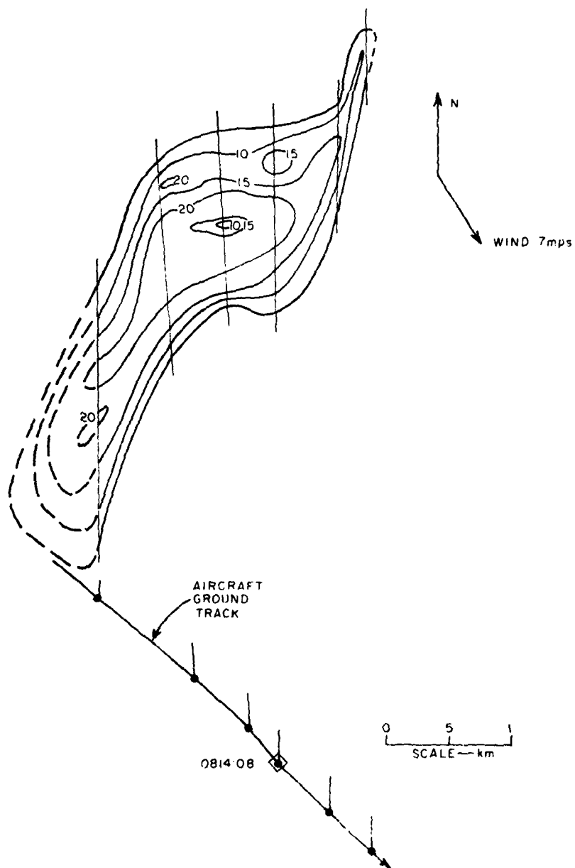
FIG. 8 RELATIVE HUMIDITY VARIATIONS OF 1-10-1965, 15 HRS. CLOUD RUN / 6.5 km FROM GZ IN DB ABOVE 51700 ft. (V)
