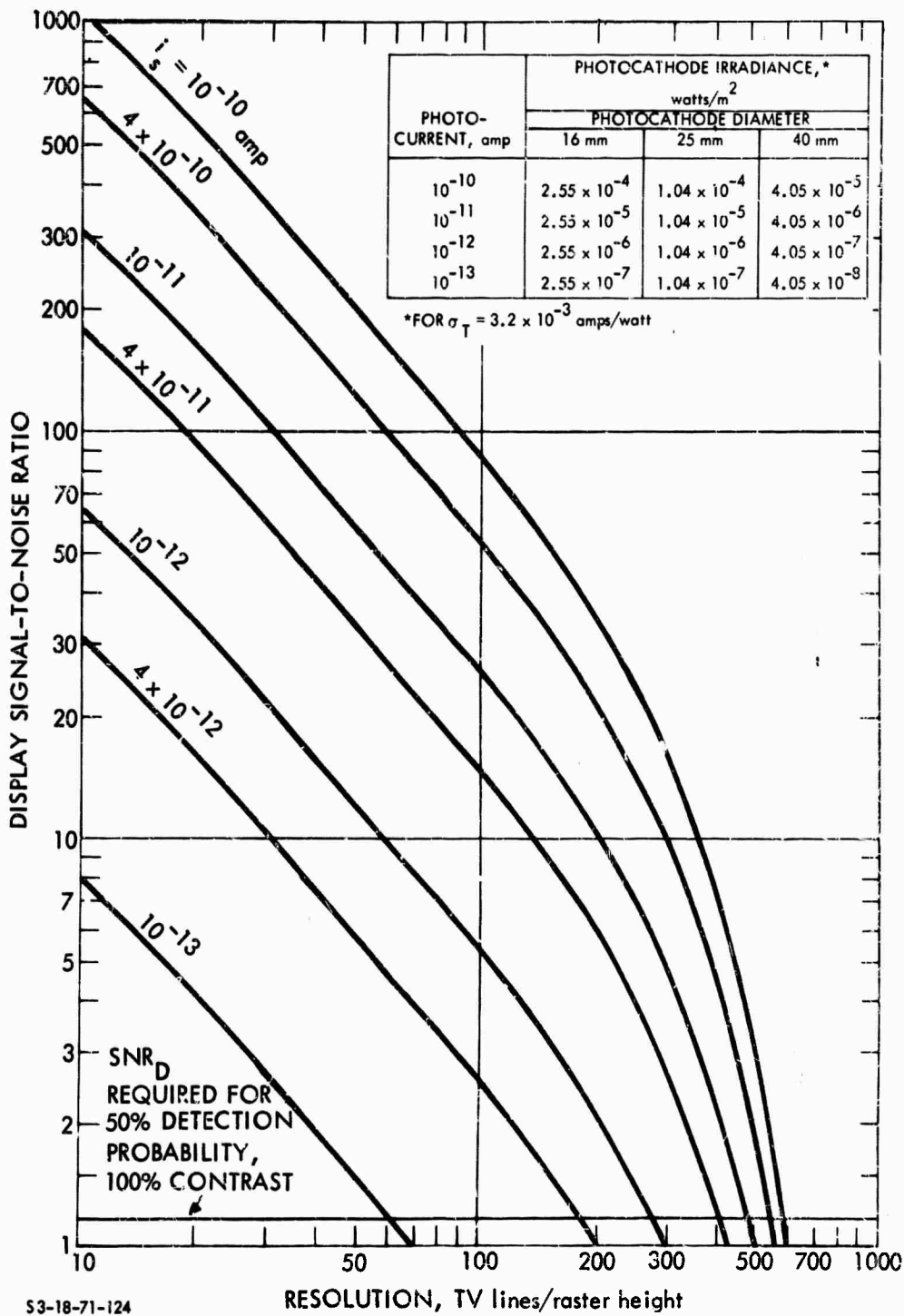
53-18-71-124 FIGURE V-F-8. Display Signal-to-Noise Ratio for SEBIR Cameras for Various Input Photocathode Currents as a Function of Pattern Resolution.
