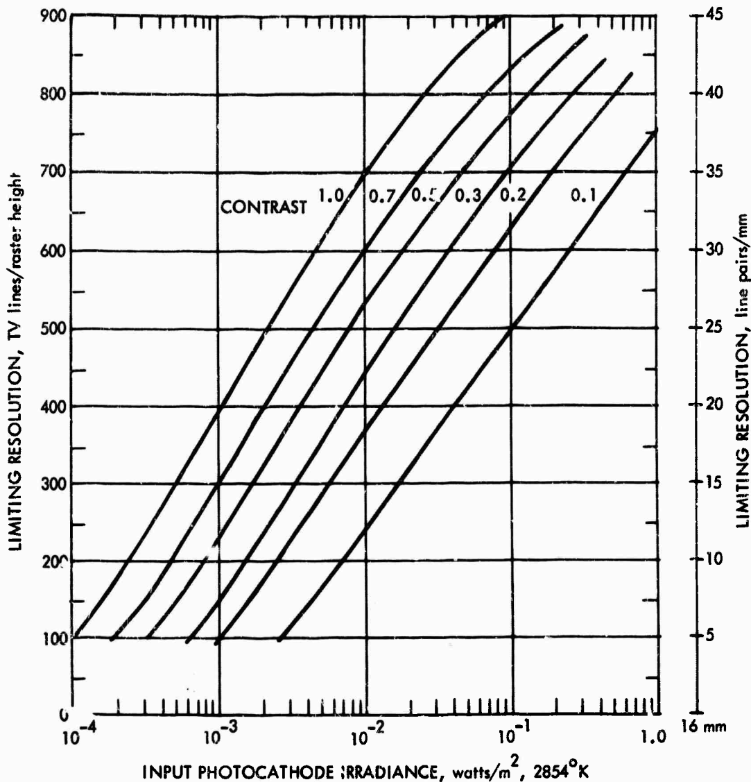
FIGURE V-C-15. Limiting Resolution Versus Input Photocathode Irradiance for the 16-mm Vidicon with 0.02 \mu\text{a} Dark Current
