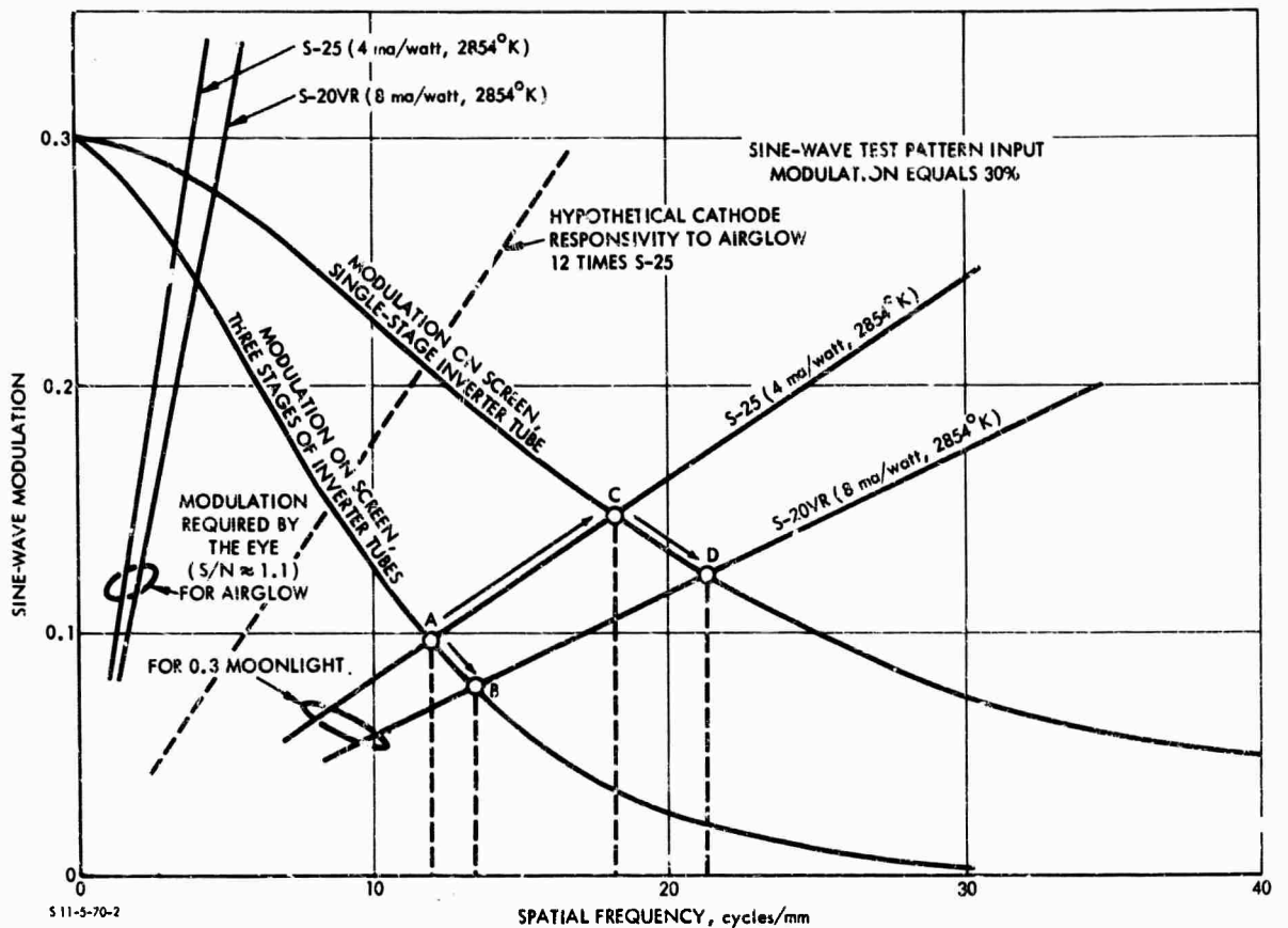
FIGURE IV-4. Predicted Effect of Cathode Responsivity Versus MTF on Image-Intensifier Performance
