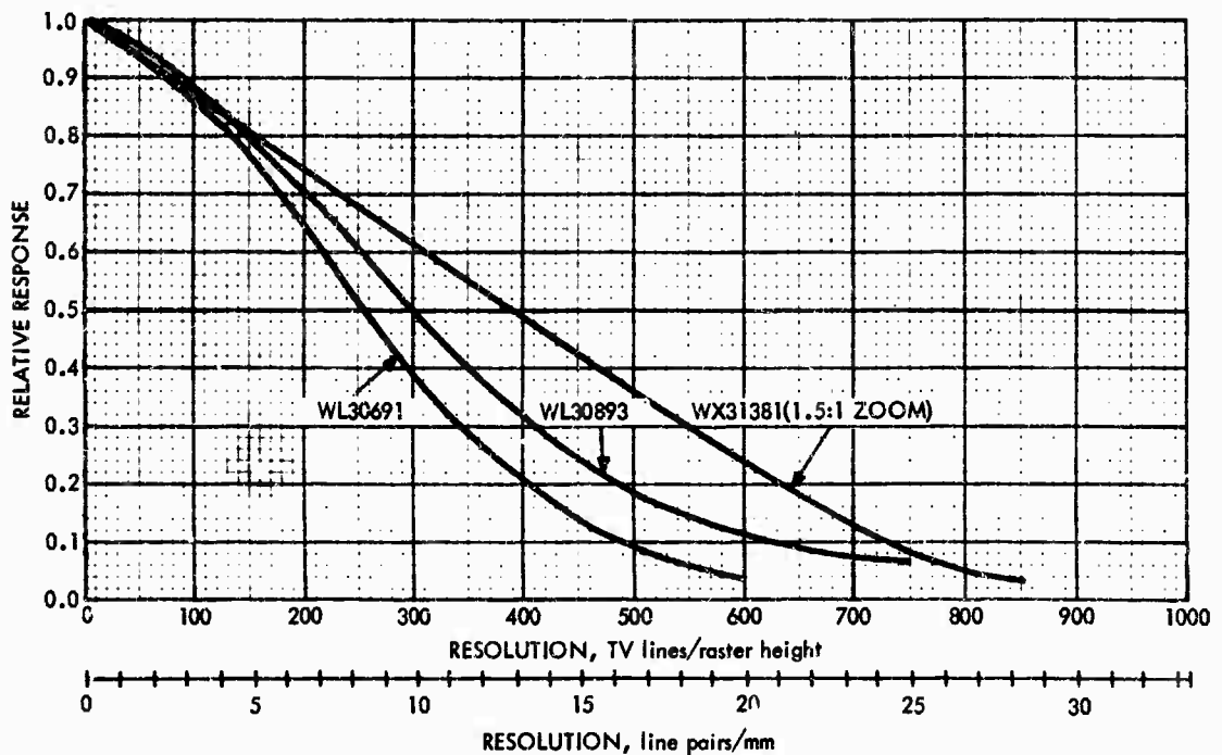
FIGURE V-D-5. Uncompensated Horizontal Square-Wave Response for SEC Cameras with 25-mm Input Photocathodes
