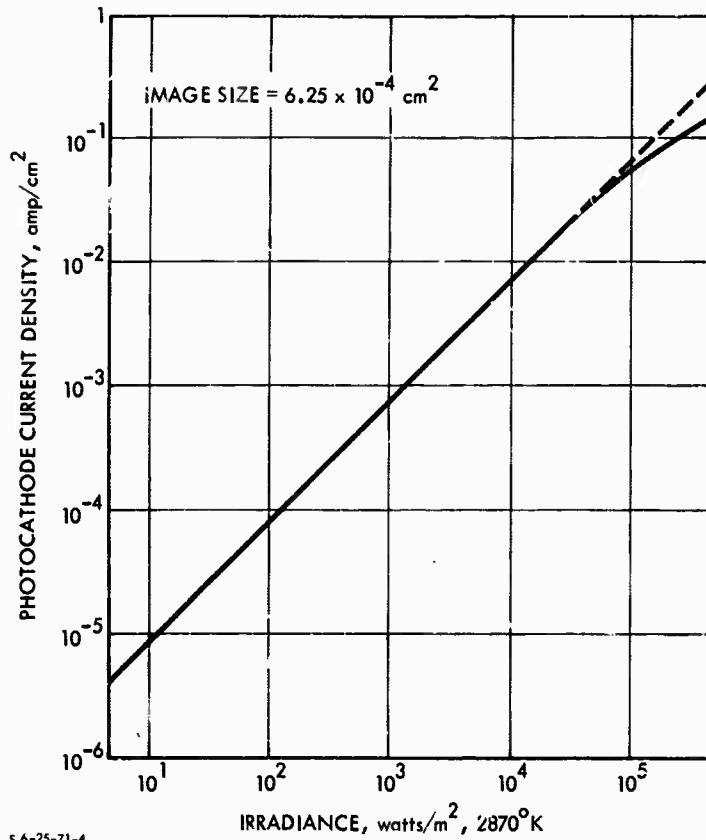
FIGURE VI-4. Proportionality of Response of SEC and SEBIR Tubes to Intense Irradiance
