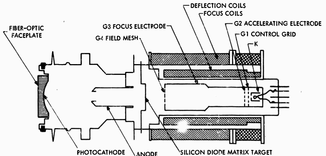
FIGURE V-F-1. Cross Section of a SEBIR Camera Tube
