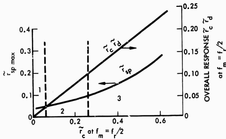
FIGURE II-9b. Maximum Spurious Response \tilde{r}_{sp}^{max} and Overall Response \tilde{r}_{c d} for MTF_d = MTF No. 3 and Various Camera MTF 's at f_m = f_r/2
