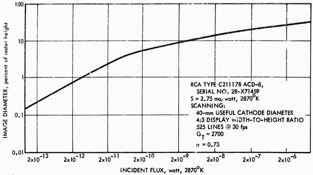
FIGURE VI-12. Image Spread in 40-mm RCA SEBIR Camera Tube Versus Incident Flux
