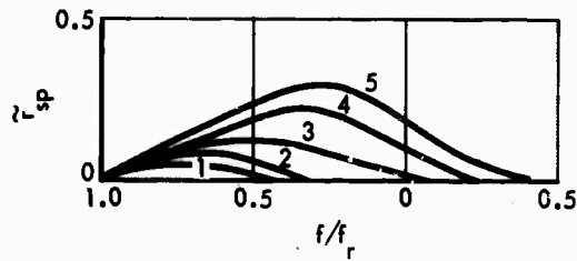
FIGURE II-9a. Cross Products \tilde{r}_{sp} for MTF_S = MTF No. 3 and Various MTF_c Curves 1 to 5
