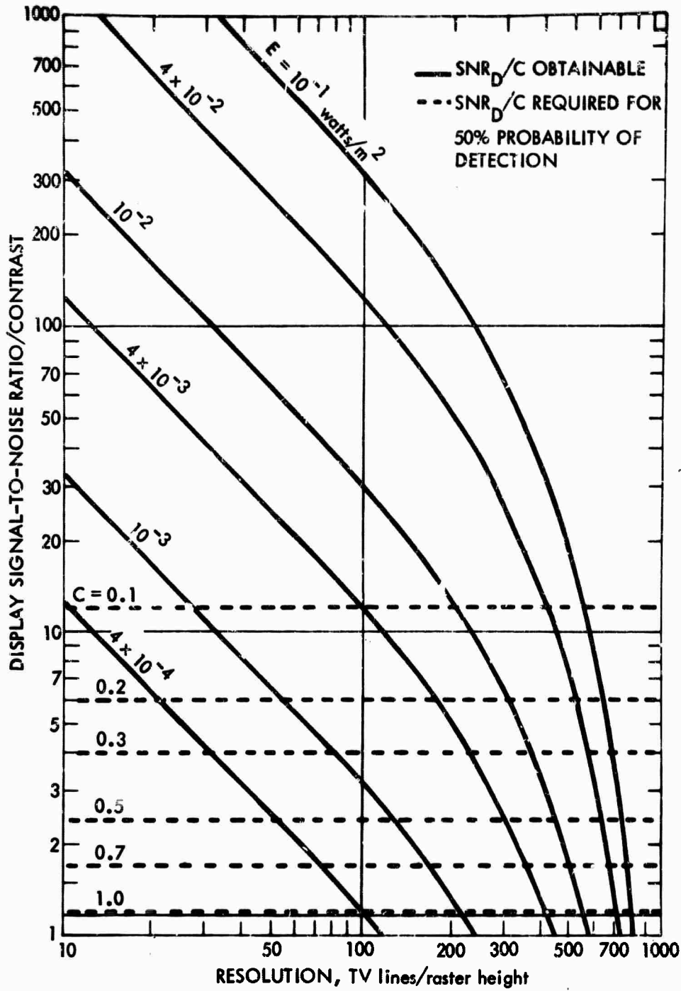
FIGURE V-C-5. Display Signal-to-Noise Ratio Versus Resolution for the Lead-Oxide Vidicon for Various Image Highlight Irradiances
