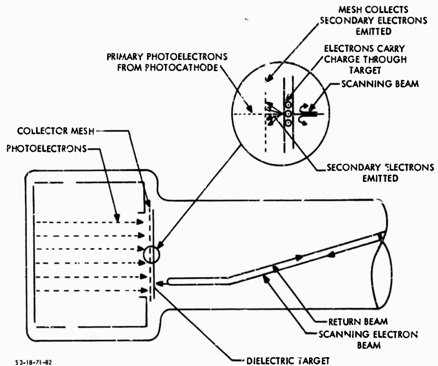
FIGURE V-E-2. Cross Section Showing Action of Image Orthicon Storage Target
