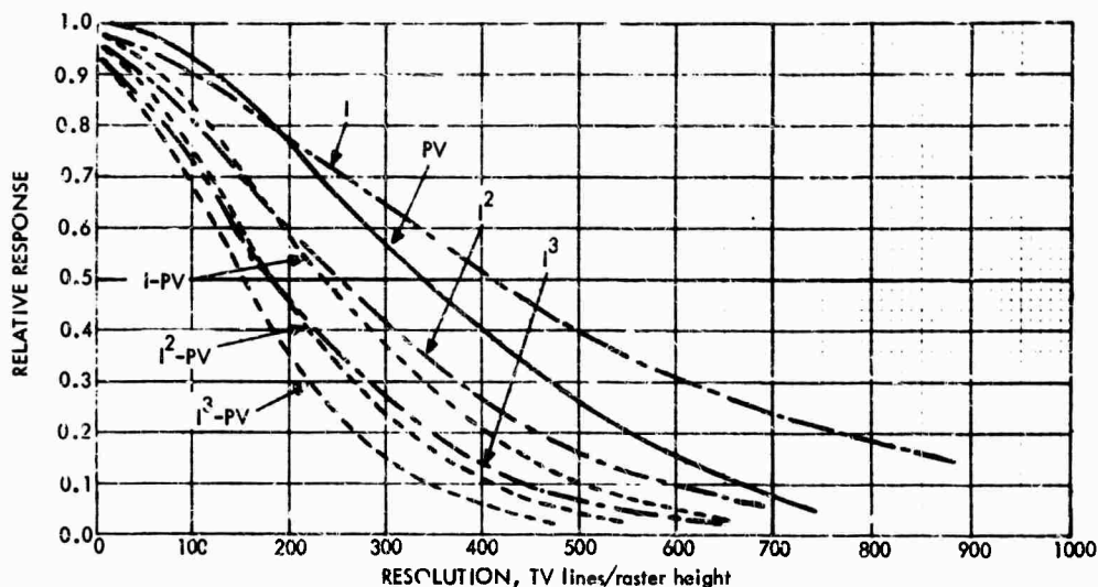
FIGURE V-C-3. Uncompensated Sine- or Square-Wave Responses for the Lead-Oxide Vidicon and its Combination with Intensifiers with 21.4-mm Phosphors. (Intensifier Response is Sine Wave; Lead-Oxide Vidicon and Intensifier Lead-Oxide Vidicon Response is Square Wave.)
