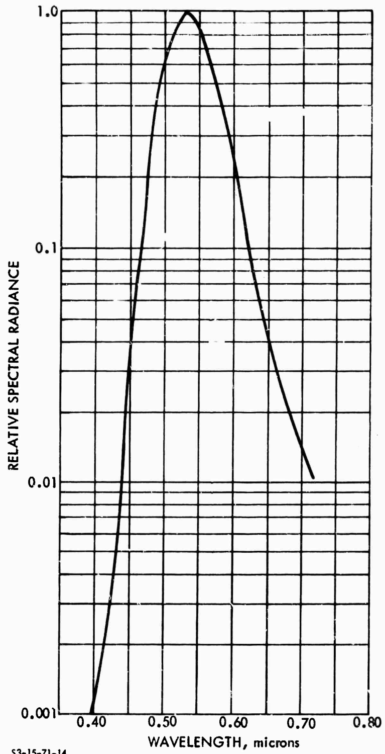
FIGURE III-6. Relative Spectral Radiance of a Modified P-20 Phosphor
