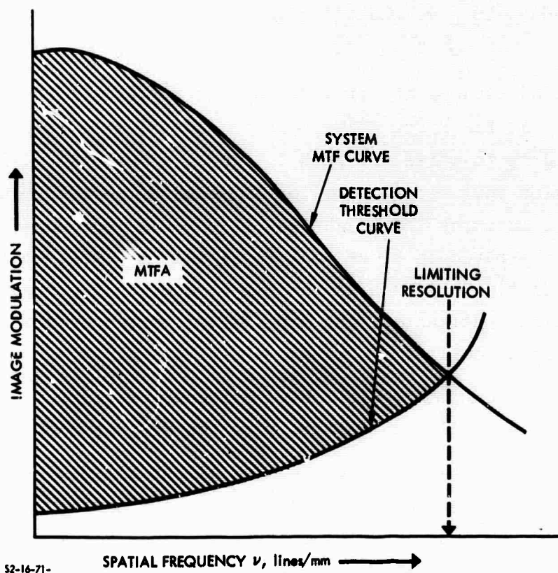
FIGURE 1. Modulation Transfer Function Area (MTFA)
