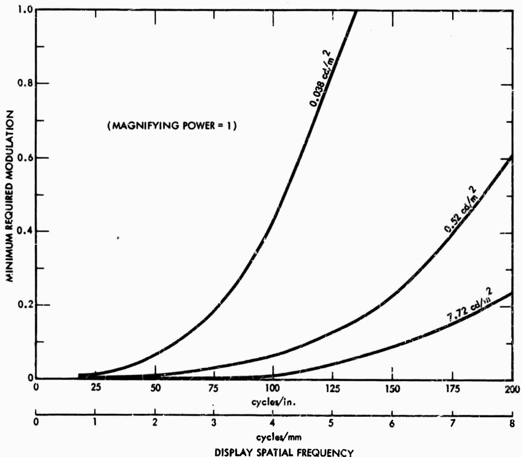
514-28-70-1 FIGURE III-10. Minimum Required Modulation for Detection of Sine-Wave Pattern by Eye (Ref. 9)
