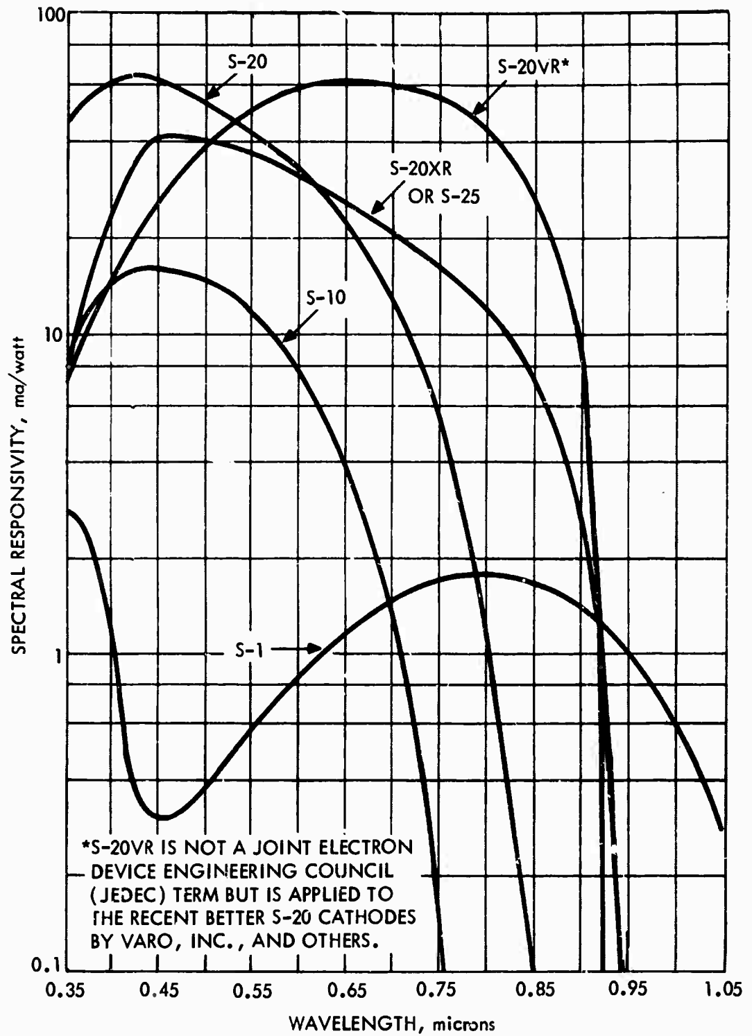
FIGURE III-5. Spectral Responsivity Versus Wavelength for Several Photoemissive Photocathodes
