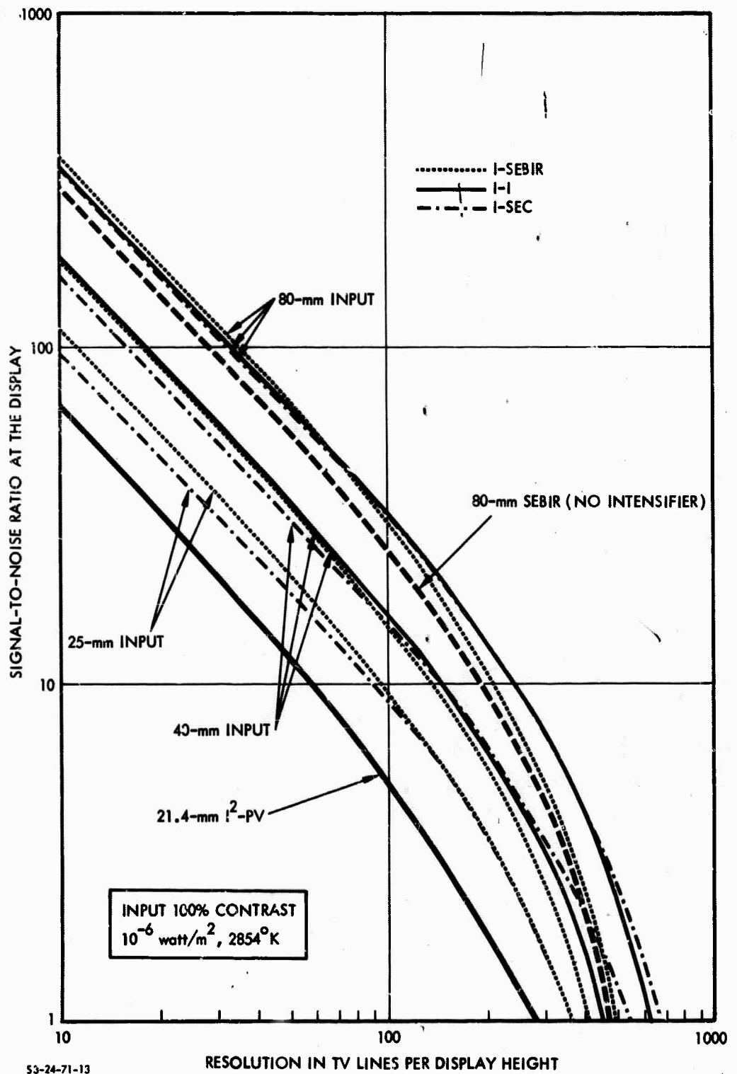
FIGURE VII-1. The Performance of Some Tube-Intensifier Combinations
