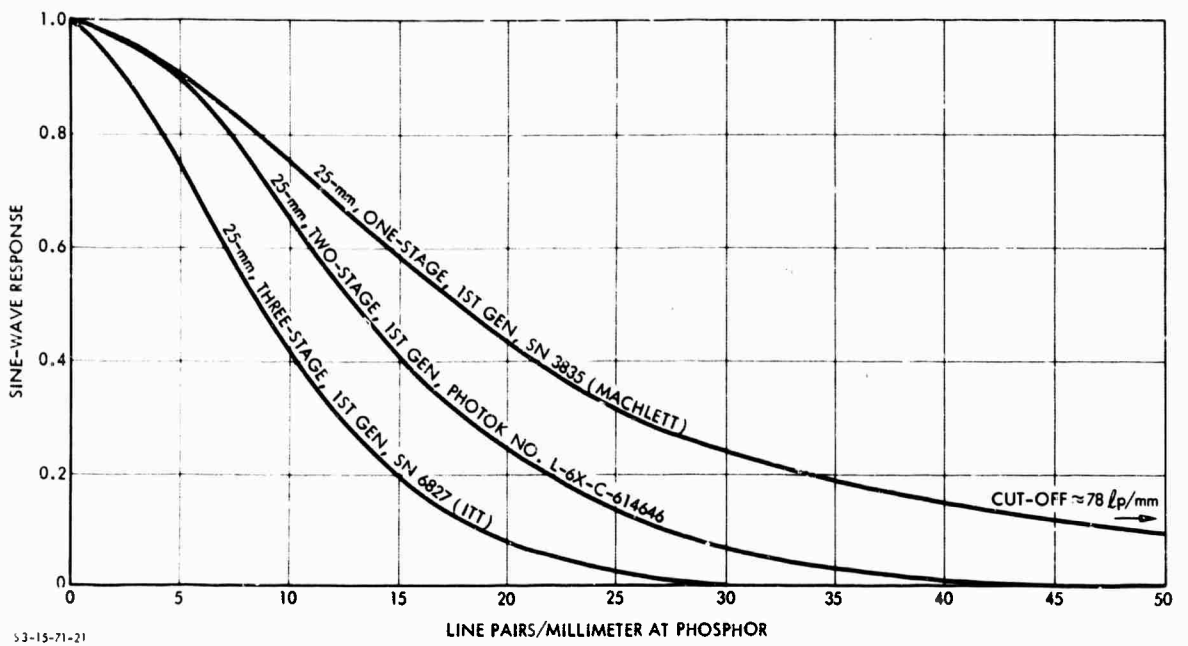
FIGURE III-8. Modulation Transfer Function of Image Intensifiers
