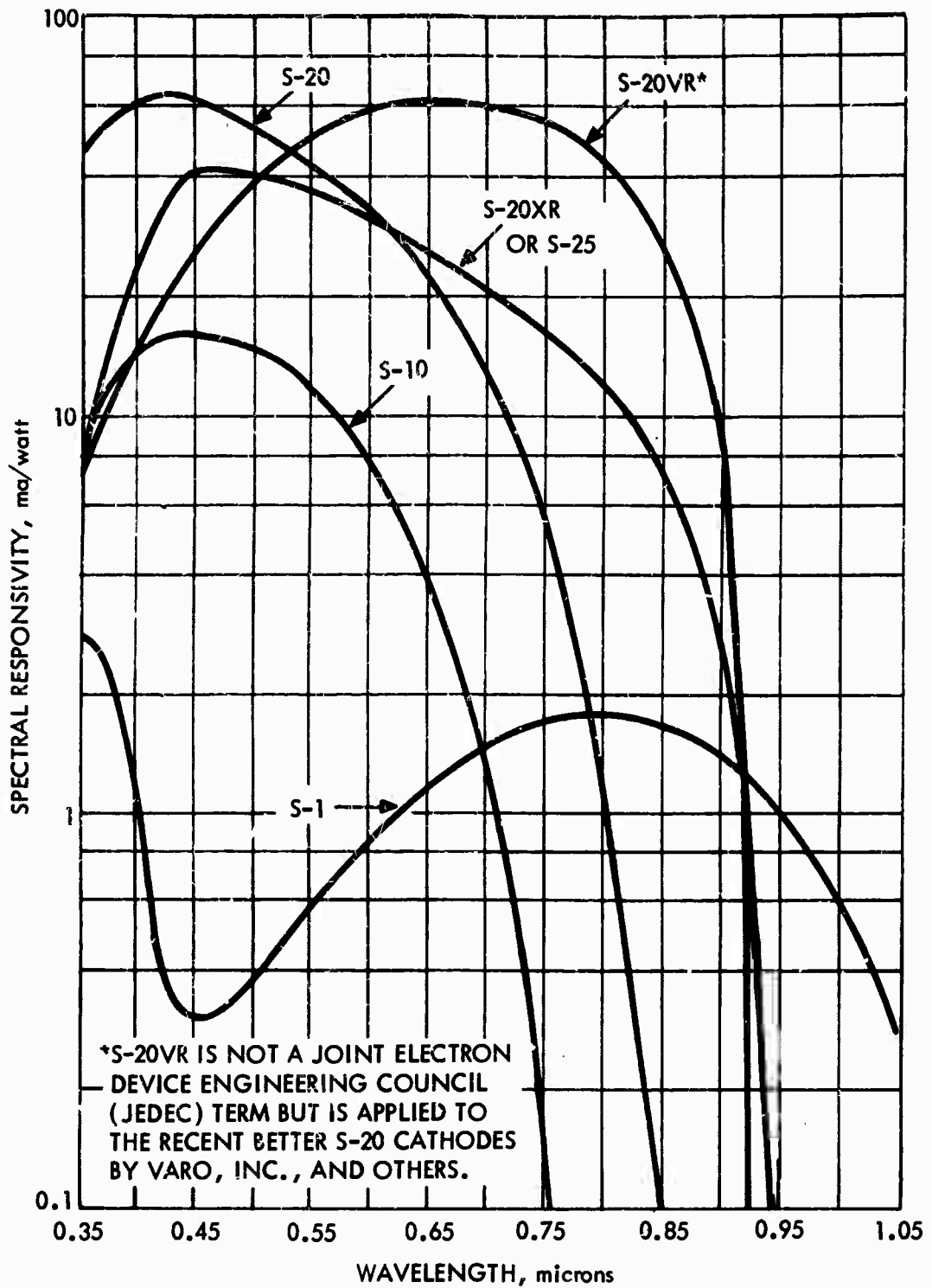
FIGURE V-B-2. Spectral Responsivity Versus Wavelength for Several Photoemissive Photocathodes. (S-20VR Substrate on Fiber Optics, Others on Lime Glass.)
