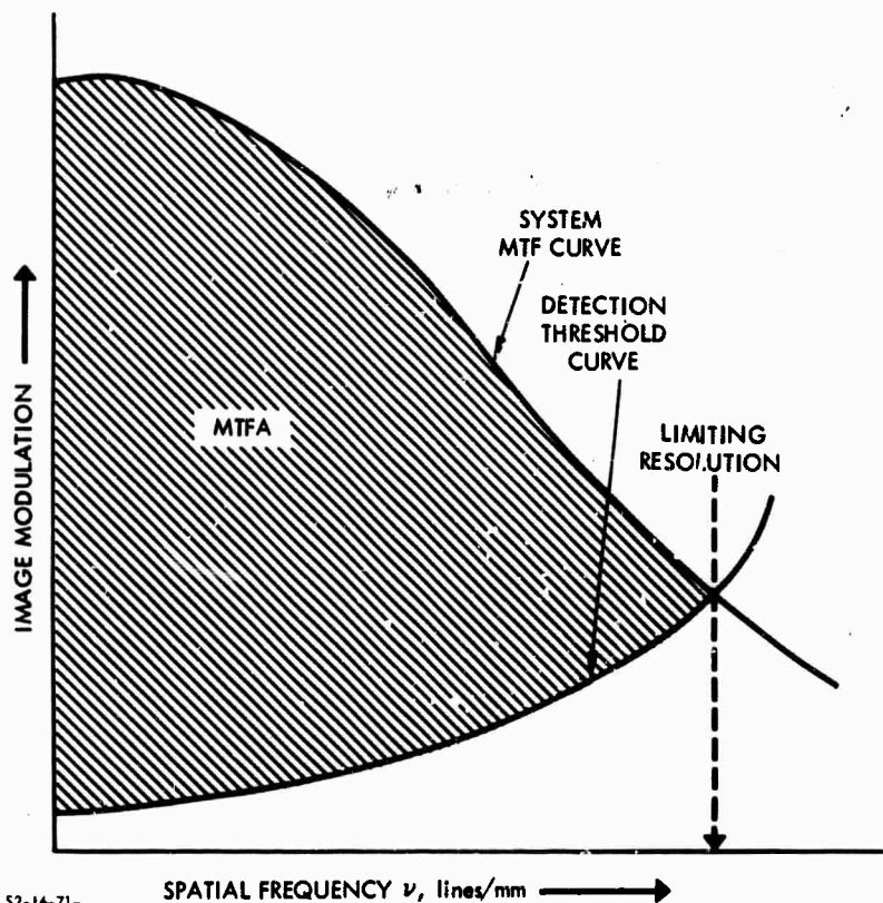
FIGURE II-1. Modulation Transfer Function Area (MTFA)
