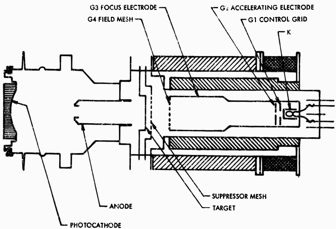
FIGURE V-3-1. Cross Section of an SEC Camera Tube
