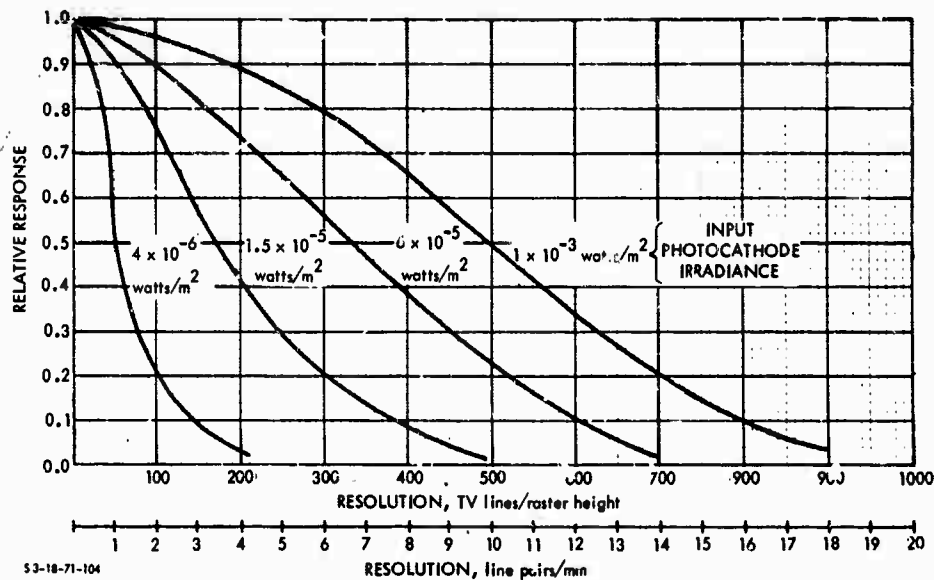
FIGURE V-E-24. Uncompensated Horizontal Square-Wave Response for the RCA C21095 Image Isocon at Various Input Photocathode Irradiance Levels. (See also Fig. V-E-36.)
