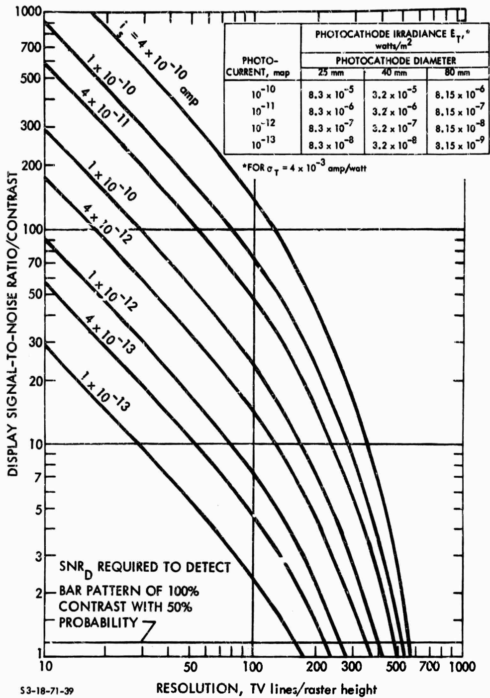
FIGURE V-C-21. Display Signal-to-Noise Ratio Versus Resolution for the Triple Intensifier Vidicon for Various Input Photocurrents, Using a 25-mm Vidicon TV Pickup Tube
