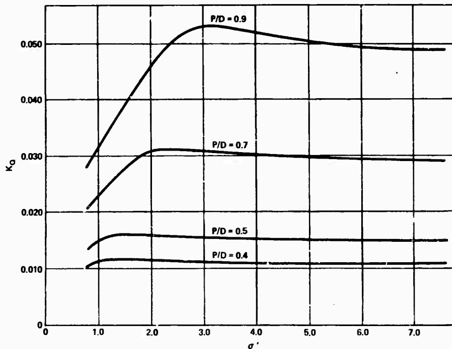
Figure 12b - Torque Coefficient
