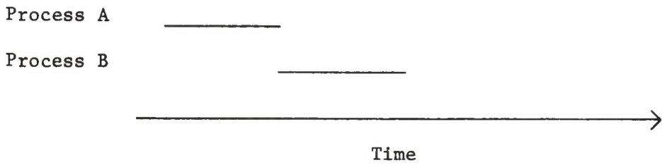
Figure 1. Consecutive Processes
