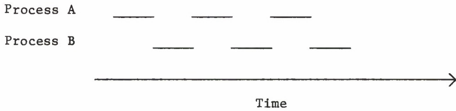
Figure 2. Interleaved Processes
