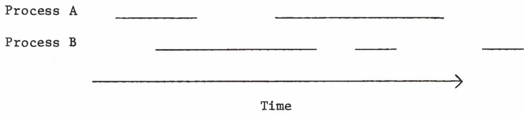
Figure 3. Overlapped Processes
