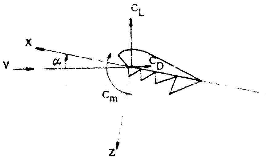
b) Longitudinal forces and moments (Pure Pitch)
