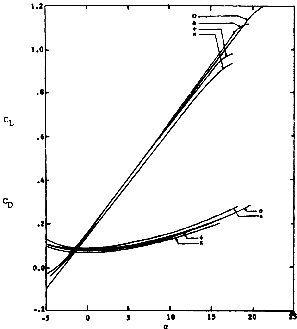
Figure 36. Rigid Airfoil with Model Variations
