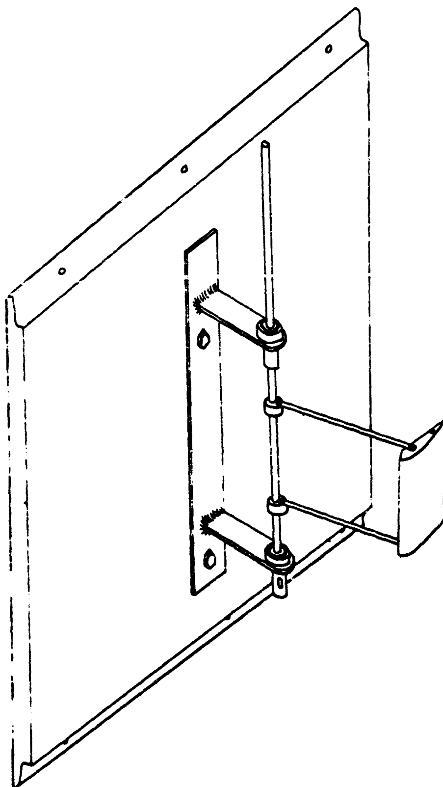
Fig. 25 Suspension System and Model Mounted on Wind Tunnel Door
