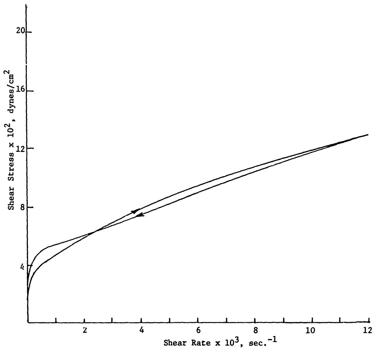
Fig. 15 - Hysteresis Loop of Gel C
