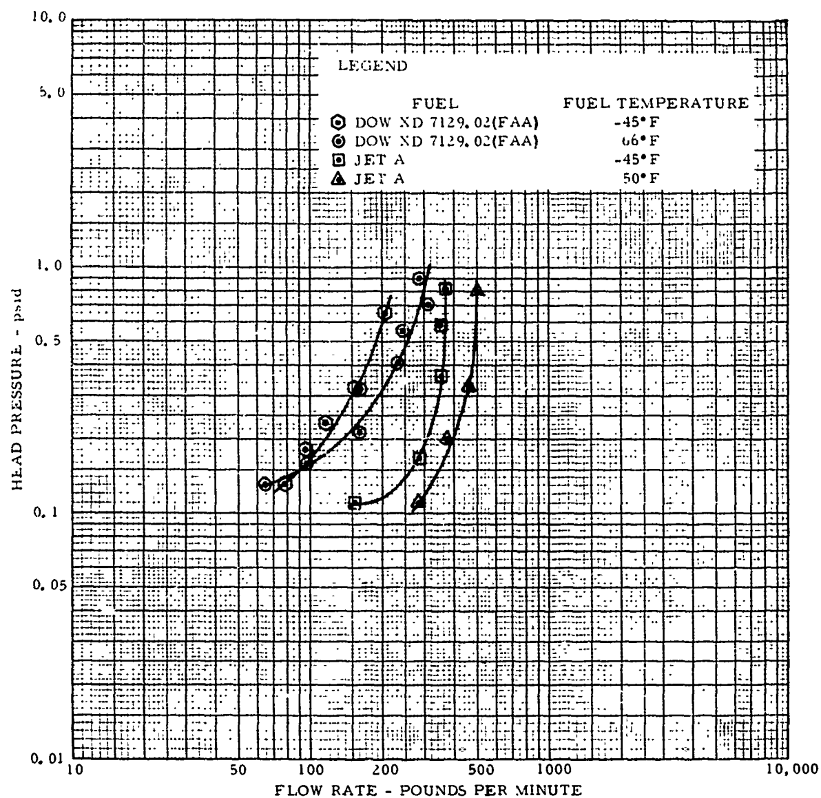
FIGURE 42B. PIPE FLOW - .062" x 2 1/2" x 72" LGT. (6° SLOPE)
