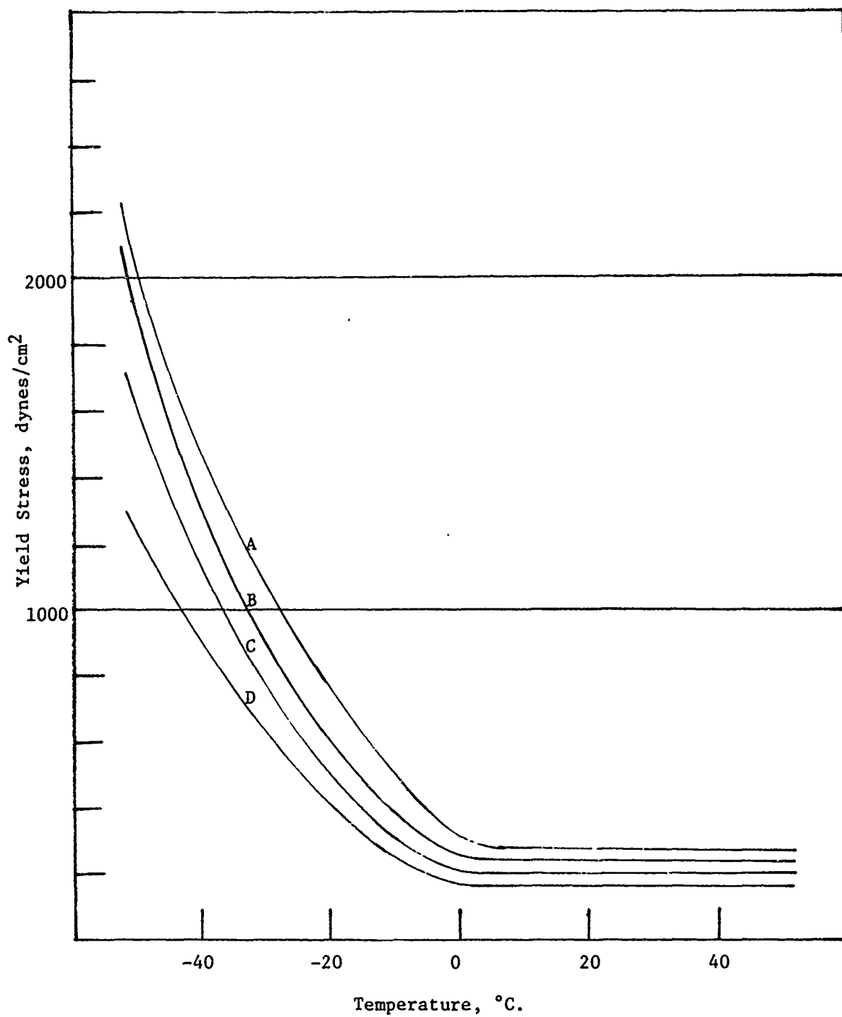
Fig. 1 - Yield Stresses of Gels at Various Temperatures
