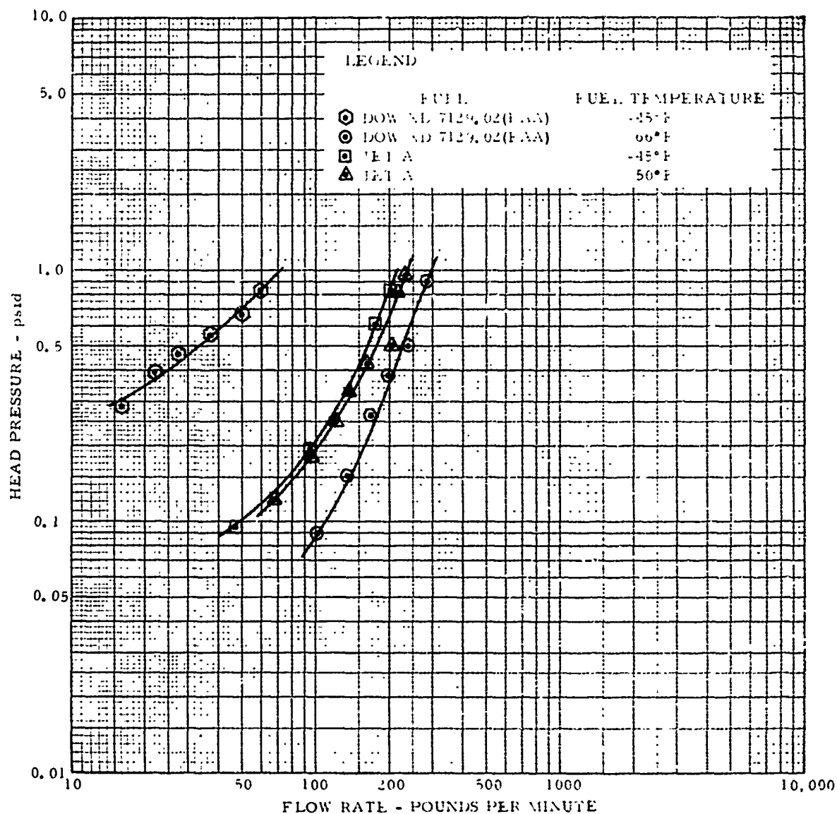
FIGURE 42A. PIPE FLOW - .049" x 1 1/2" x 72" LGT. (6° SLOPE)
