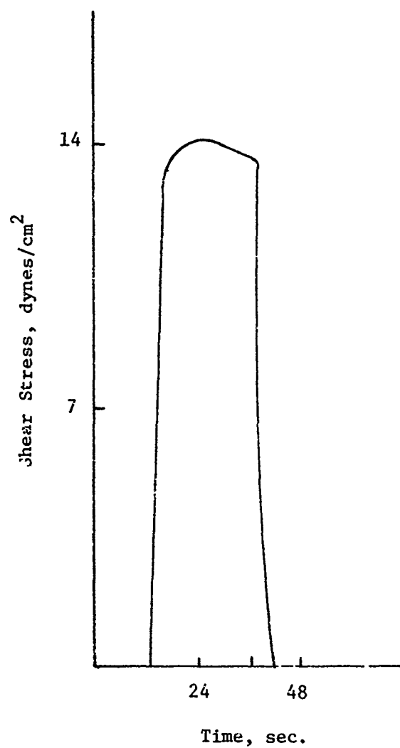
Fig. 23 - Viscoelasticity Measurements of Gel D - 20 sec. -1 Shear Rate at 10°C. Temperature
