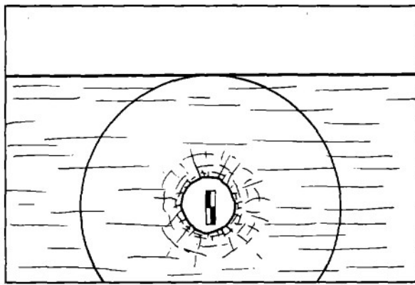
(a) Stress wave reaches surface
