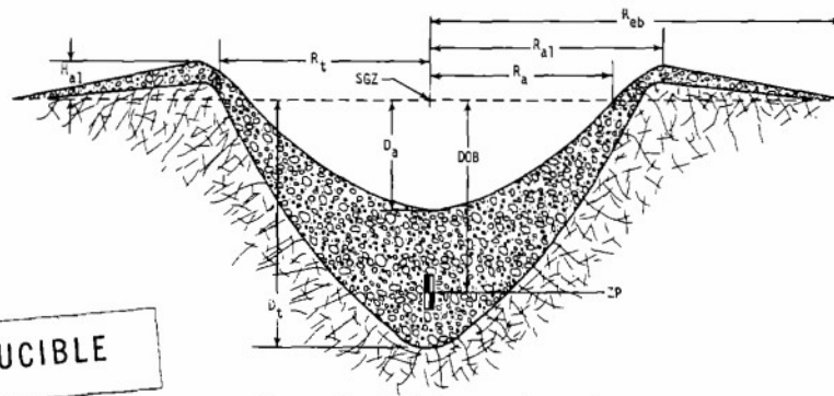
Cross section of a single or row-charge crater
