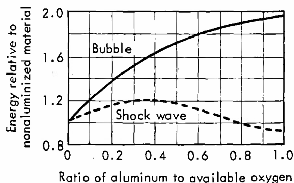
Fig. 16. Effect of aluminum on underwater shock and bubble energy 6 (calculation of aluminum-to-available-oxygen ratio is given in Appendix C).
