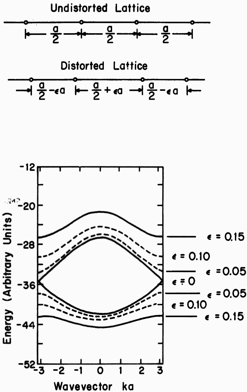
FIGURE I-3 The distortion parameter \epsilon and the dependence of E(k) on \epsilon in one dimension as calculated by Adler and Brooks [23].
