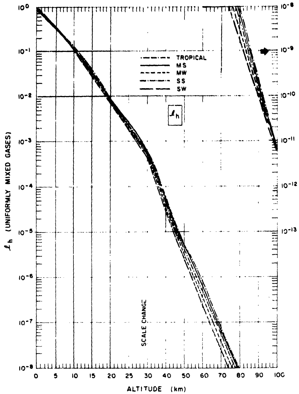
Figure 4. Equivalent Sea Level Path Length of Uniformly Mixed Gases as a Function of Altitude for Horizontal Atmospheric Paths
