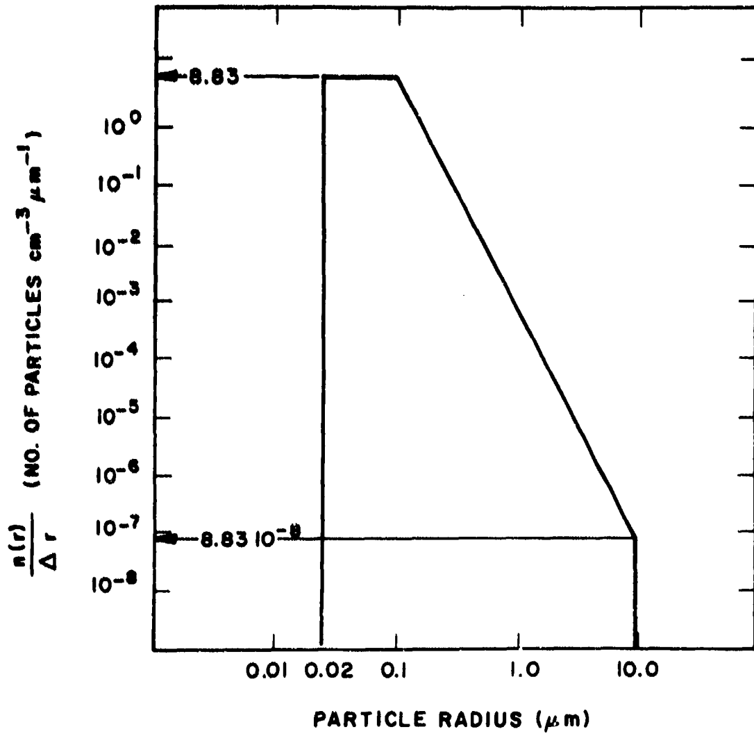
Figure 1. Normalized Particle Size Distribution for Aerosol Models
