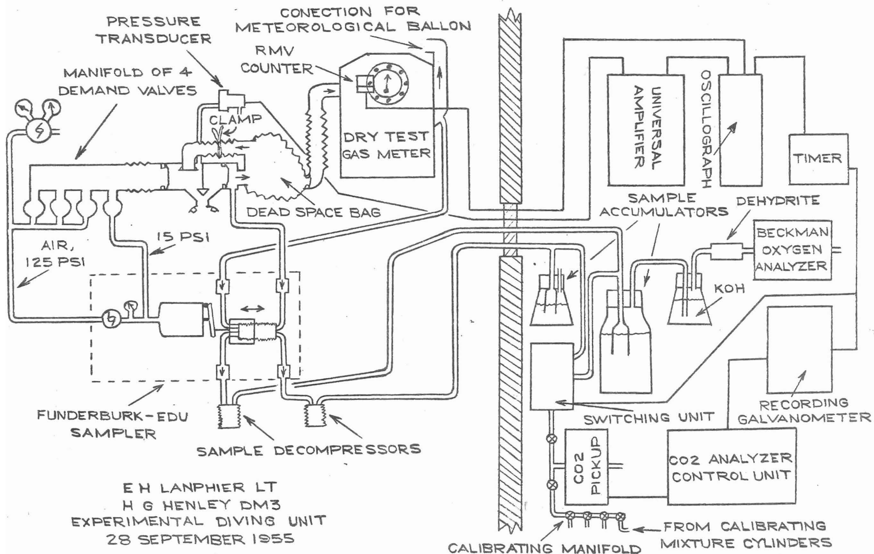
FIGURE 2 APPARATUS FOR DEAD SPACE STUDY
