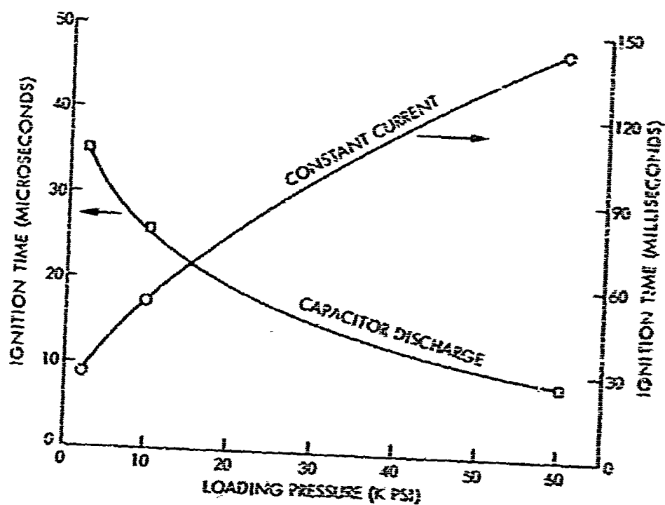
FIG. 4 EFFECT OF LOADING PRESSURE ON IGNITION TIME OF NORMAL LEAD STYHNATE BY CONSTANT CURRENT AND CAPACITOR DISCHARGE SIGNALS IN THEIR TYPICAL TIME REGIMES
