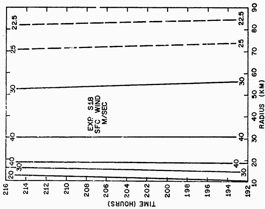
Figure C-3. Results from Experiment S18. Time-radius cross section of surface wind speed.
