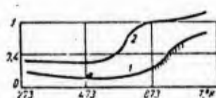
Fig. 5. Variation in Coefficient of Friction as a Function of Temperature and Method of \text{MoS}_2 Application on Friction Surface (Platinum):
