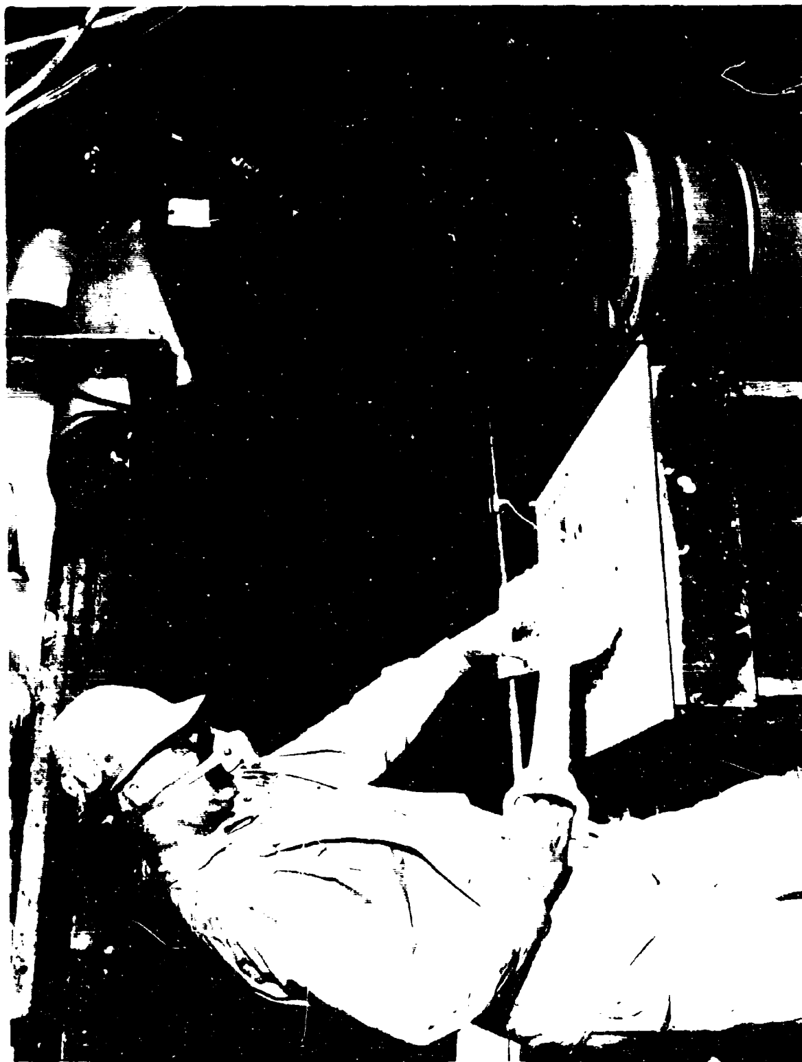
Figure 3. A portable downdraft table attached to a portable vacuum unit. The major portion of the saw cuttings are captured.
