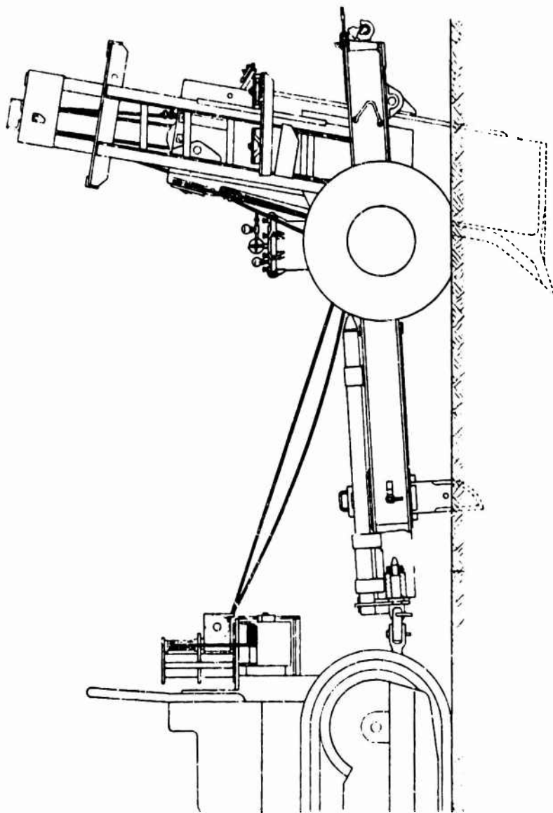
PLOW EQUIPPED FOR CABLE LAYING
