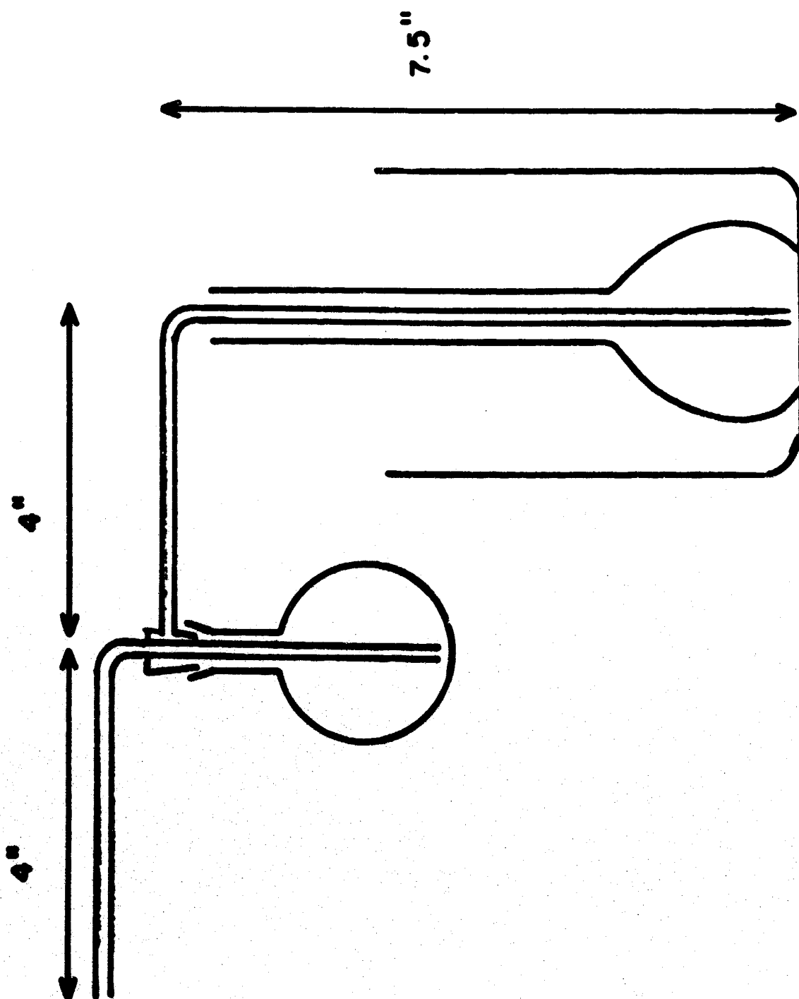
FIGURE 1. DISTILLATION APPARATUS
