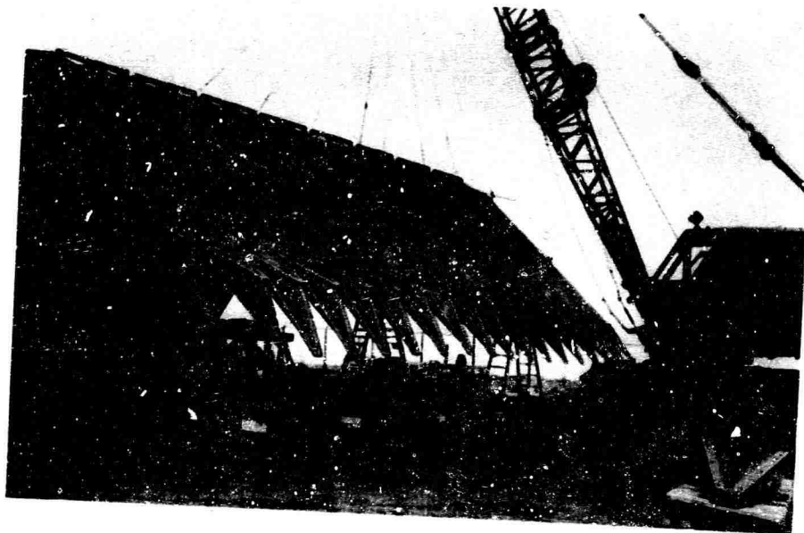
Fig. 21. Structure erection – 60 percent complete.
