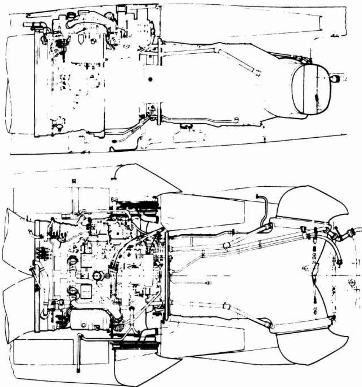
Fig.9 Harrier engine installation
