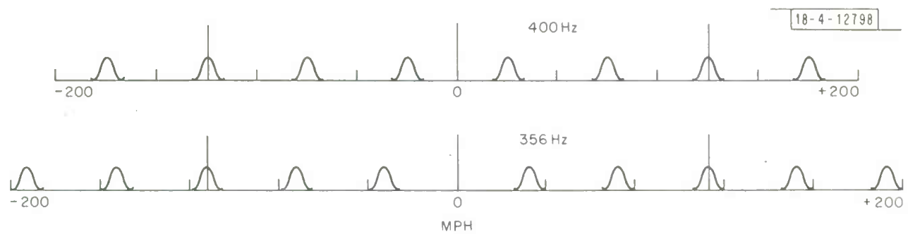
Fig. III-1. Velocity ambiguity diagram for two repetition notes.
