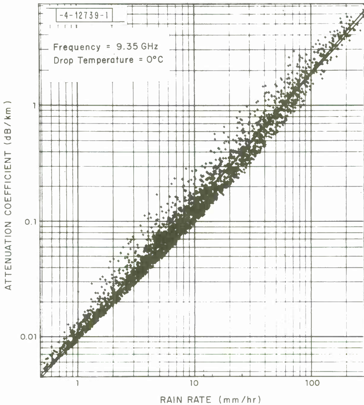
Fig. 11. Attenuation coefficient as a function of rain rate computed from drop size distributions as measured in Miami.
