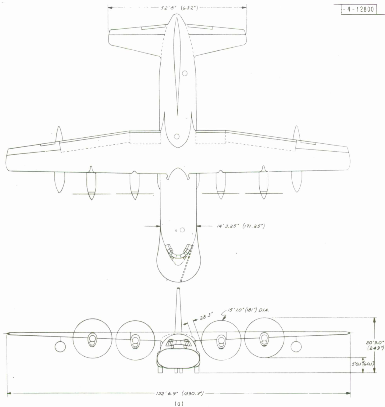
Fig. 14. Conceptual drawing of enlarged radome installed on the nose of the WC-130.
