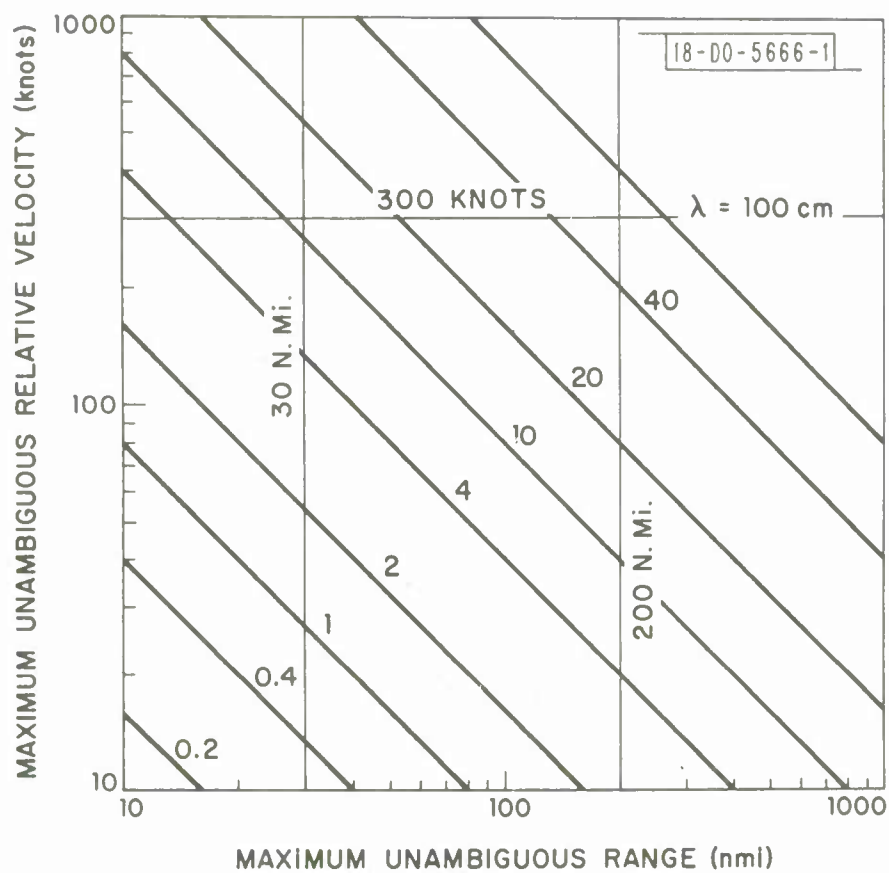
Fig. 18. Maximum unambiguous relative velocity vs maximum unambiguous range for a pulse Doppler radar with operating wavelength as a parameter.
