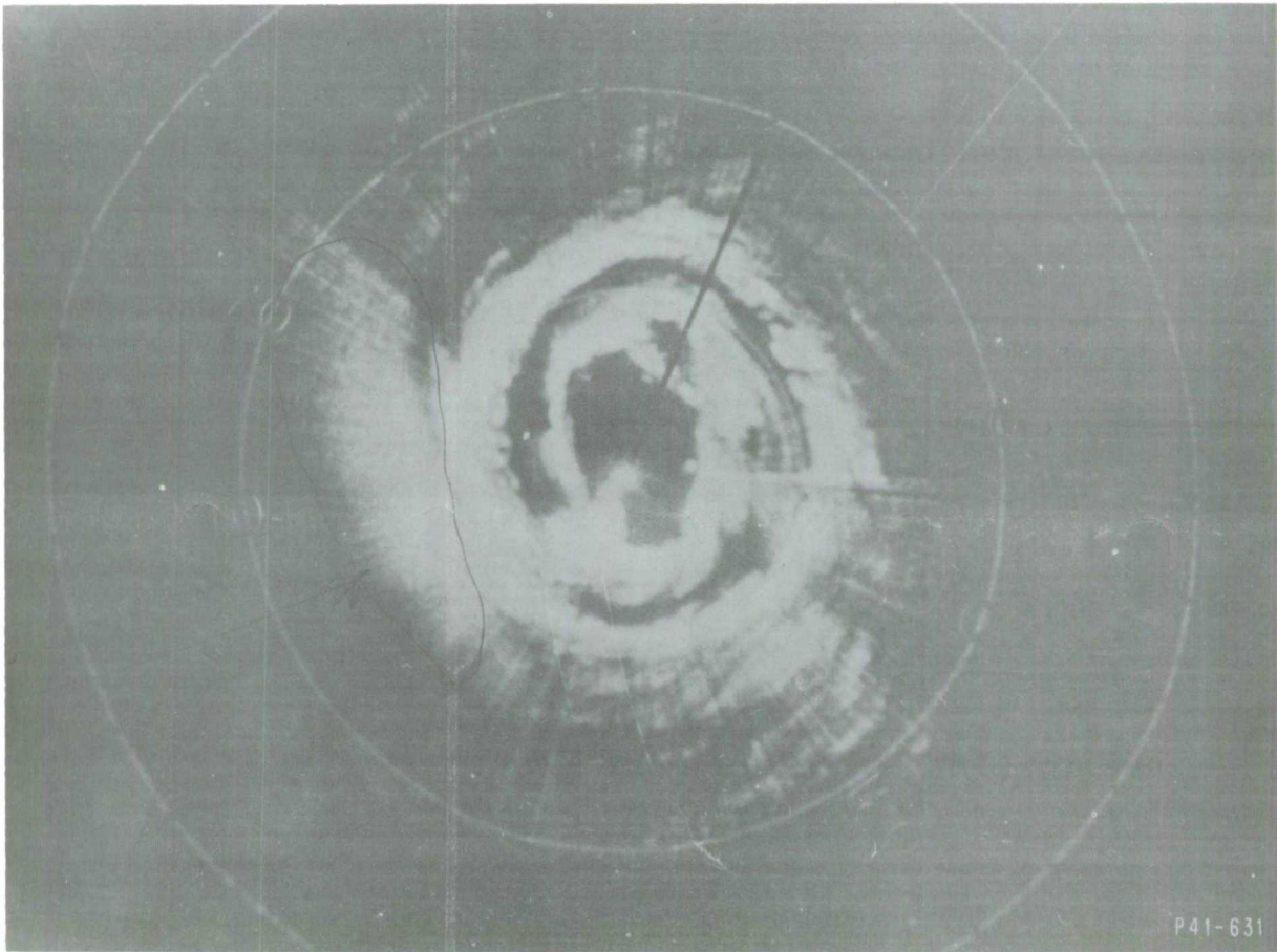
Fig. 16. Photograph of the PPI display of the APS-45 radar on a Navy WV-2 aircraft. Photo taken from inside the eye of the storm.
