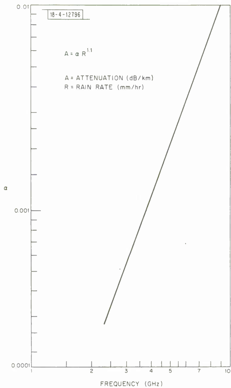
Fig. 12. Coefficient \alpha as a function of frequency.
