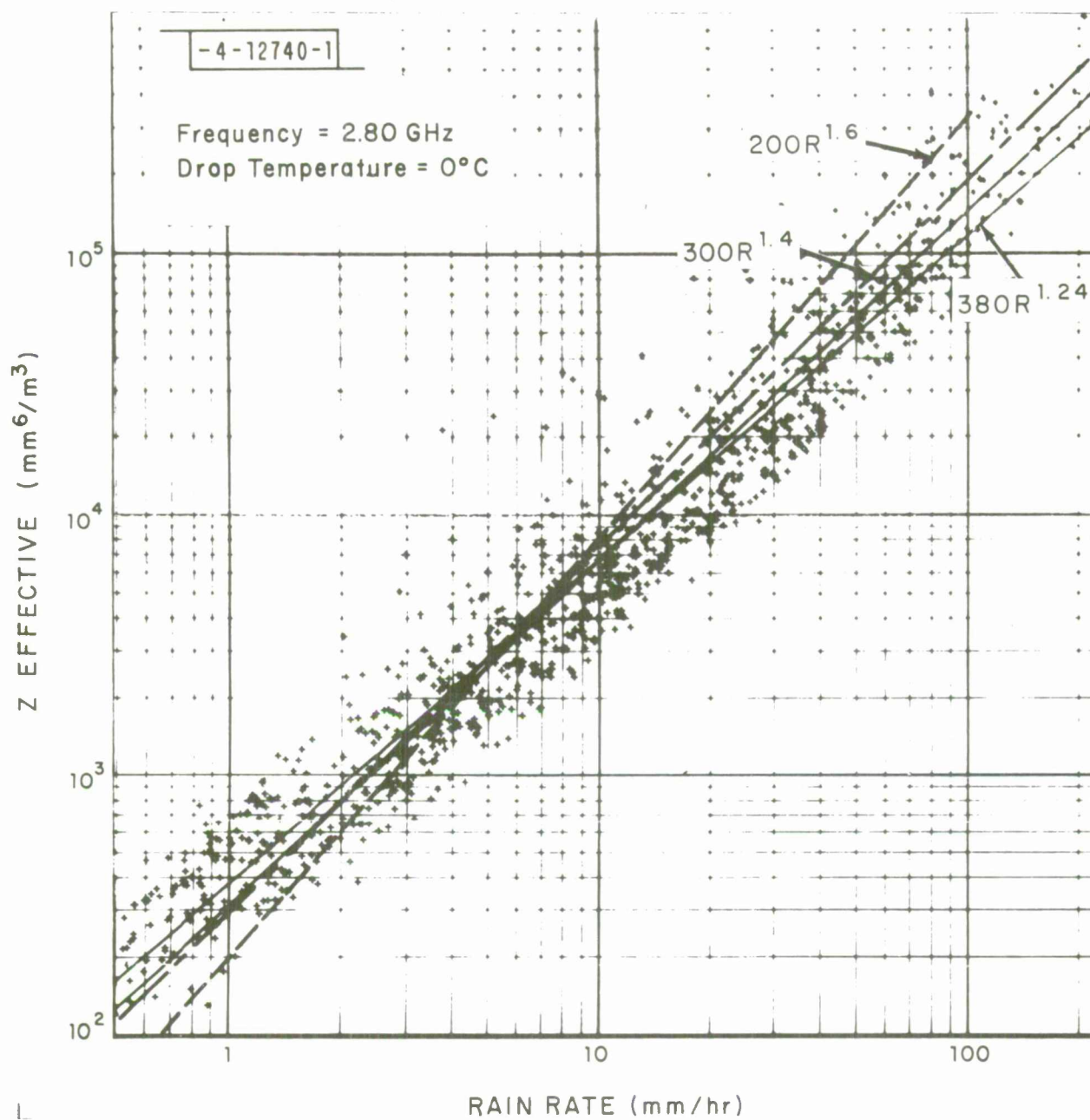
Fig. 9. Backscatter cross section as a function of rain rate computed from drop size distributions as measured in Miami.
