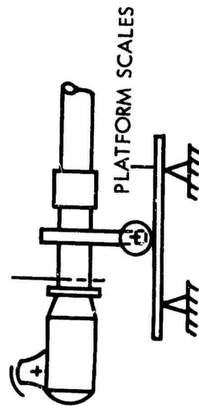
FORCE MEASURING SYSTEM FOR TEST VALVE CONFIG. NO'S. 1 & 2
