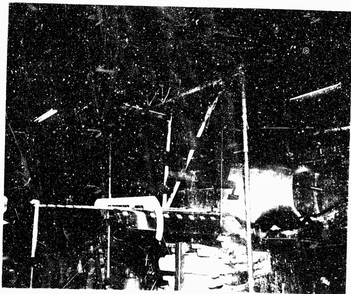
FIGURE 36 - FLAP PROOF TEST FIXTURE
