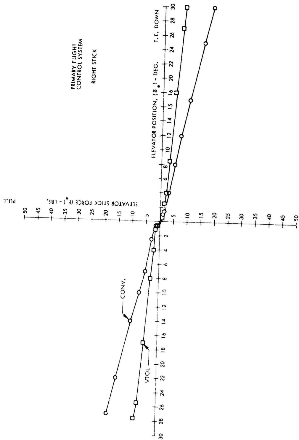
FIGURE 42 - ELEVATOR CONTROL SYSTEM CALIBRATION
