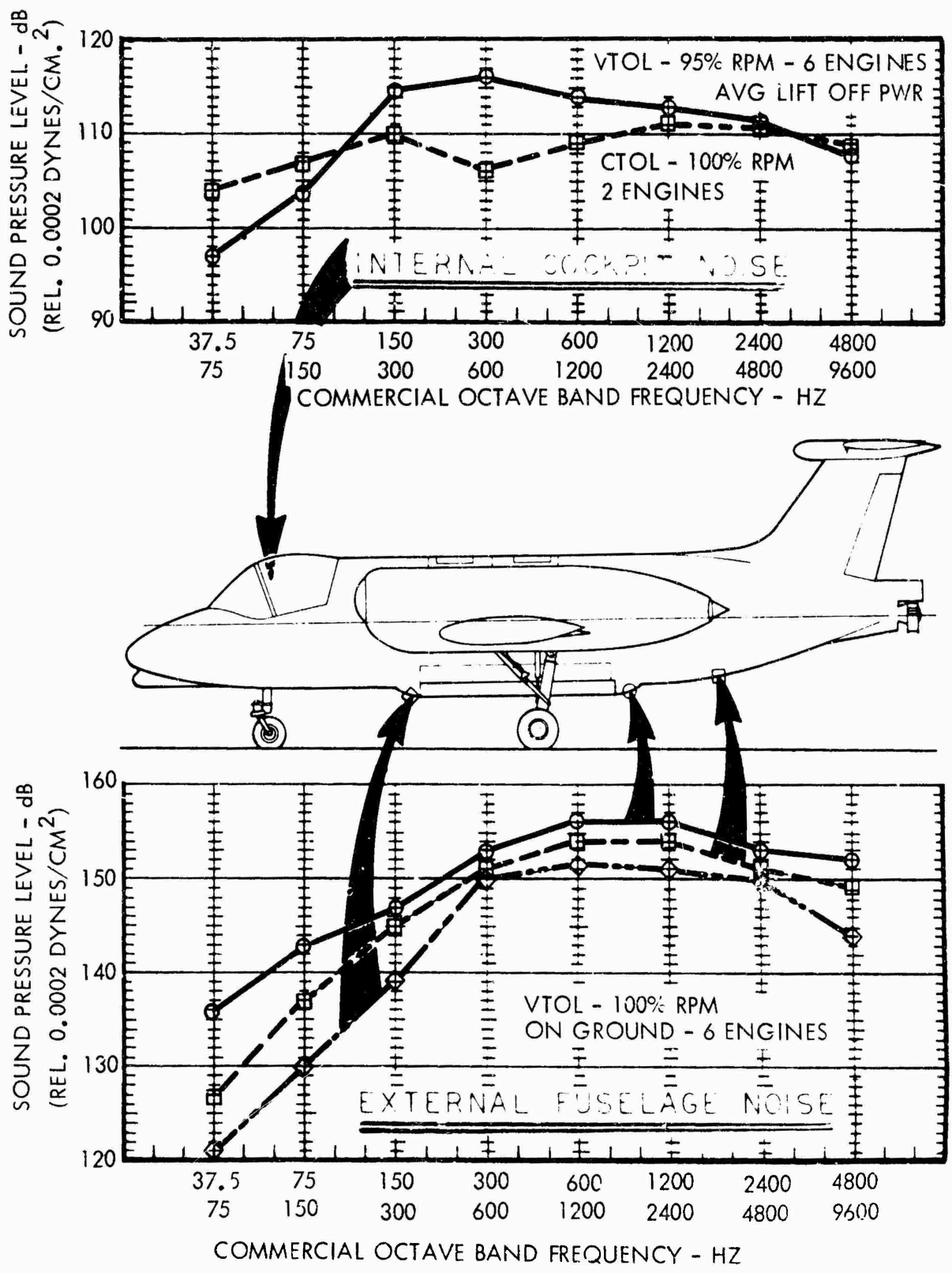
FIGURE 39 - MEASURED NOISE LEVELS
