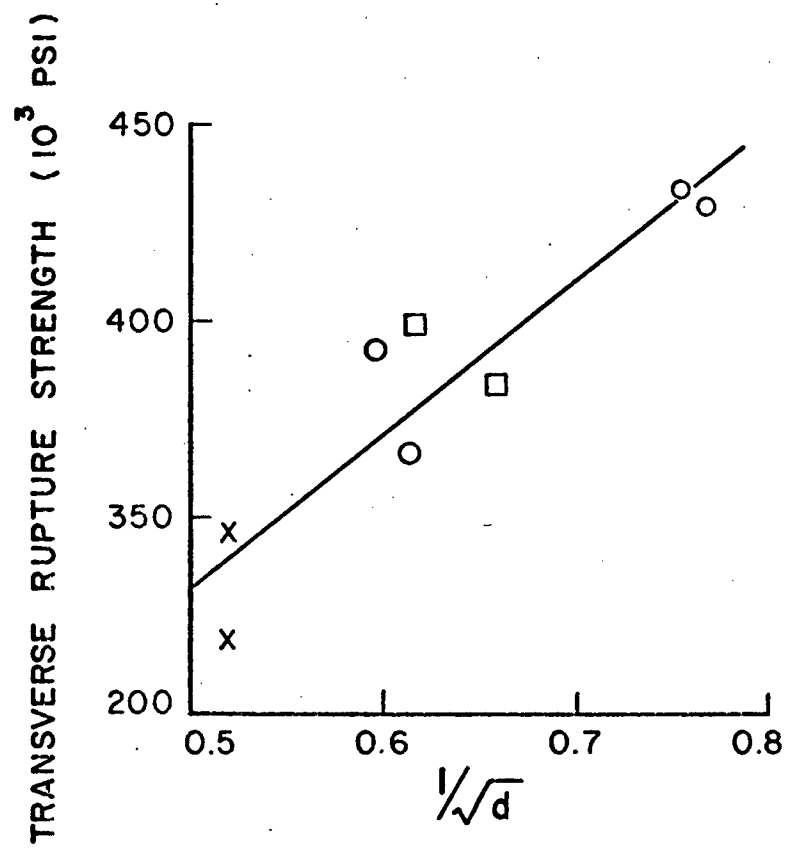
FIG. 5 TRANSITION STRENGTH
