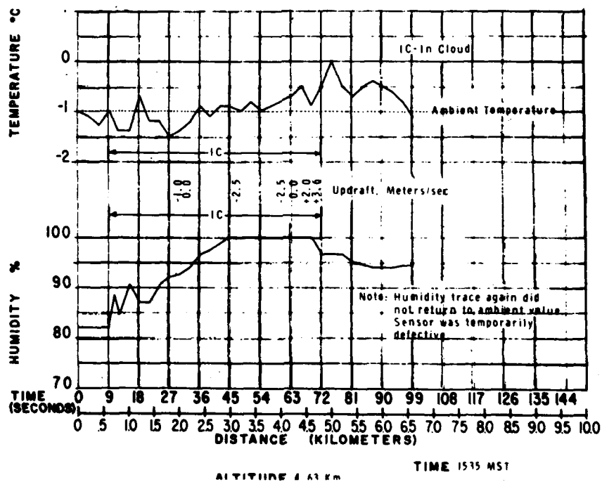
Figure 42. Cloud temperatures and humidities, 20 Jul 66, Flight No. 2, Cloud B (sixth pass).
