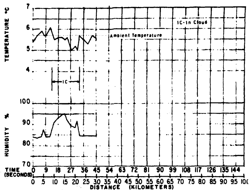
Figure 25. Cloud temperatures and humidities, 20 Jul 66, Flight No. 1, Cloud F.
