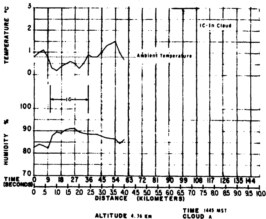
Figure 12. Cloud temperatures and humidities, 19 Jul 66, Flight No. 1, Cloud A.
