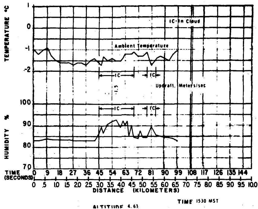
Figure 41. Cloud temperatures and humidities, 20 Jul 66, Flight No. 2, Cloud B (fifth pass).
