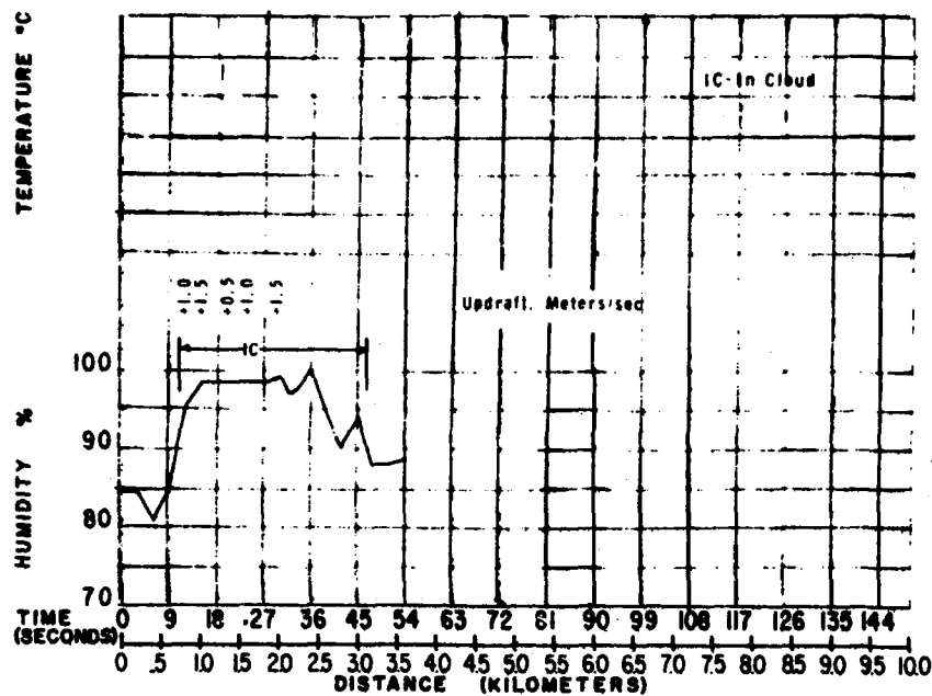
Figure 11. Cloud temperatures and humidities, 15 Jul 66, Flight No. 2, Cloud 7.
