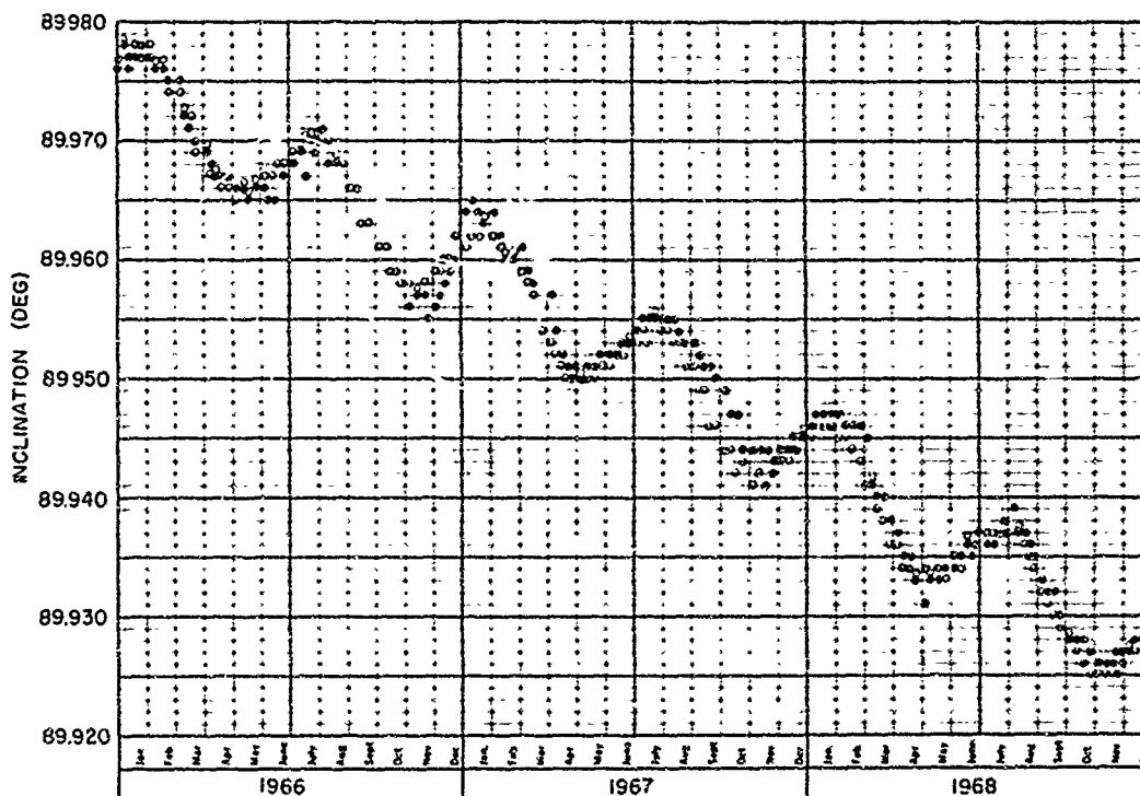
Fig. 13 - Theoretical and observed inclination for Satellite 1420. • Data o Theoretical
