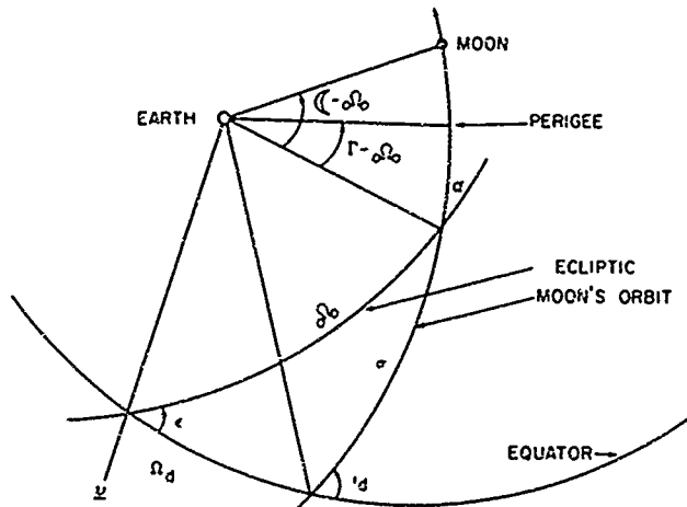
Fig. 2 - The orbital elements of the moon (modified from Ref. 1)
