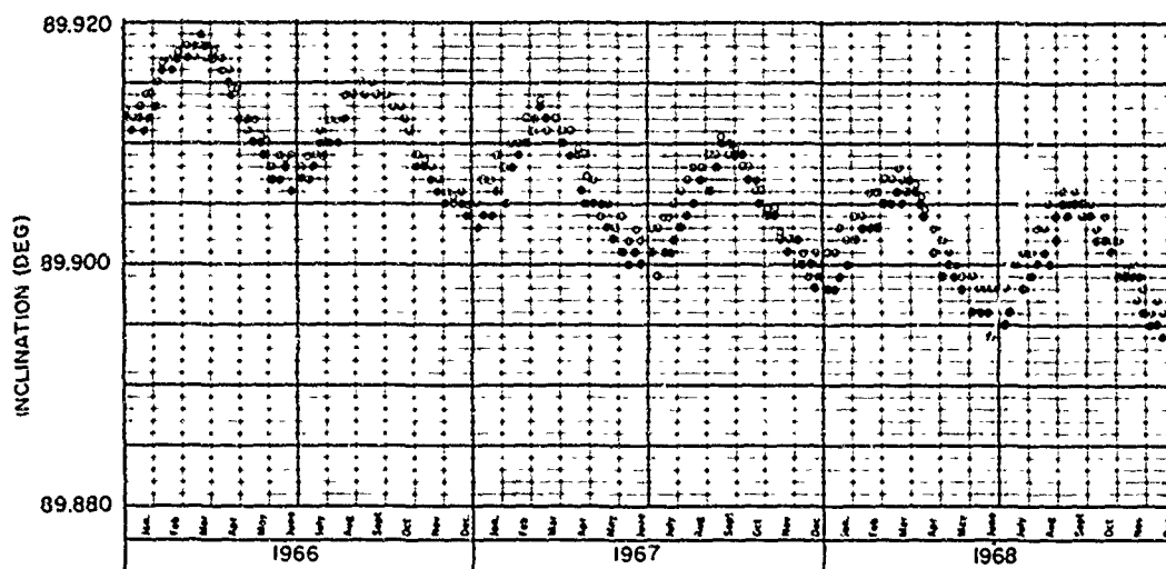
Fig. 6 - Theoretical and observed inclination for Satellite 671
