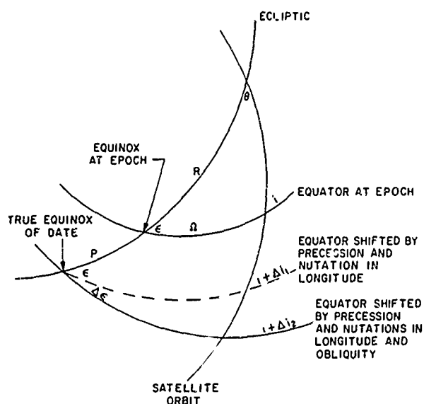
Fig. 4 - Precession and nutation effects on inclination
