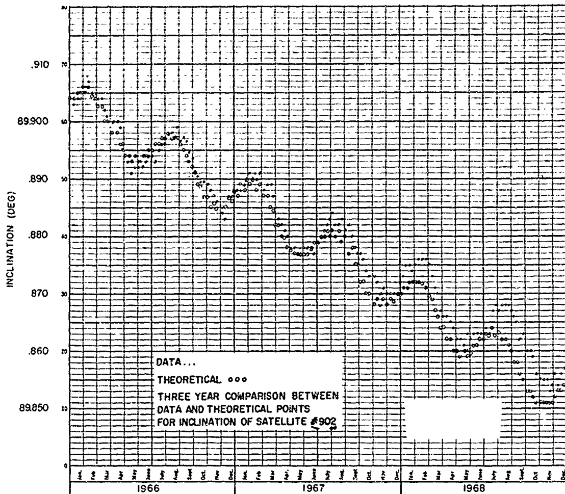
Fig. 3 - Theoretical and observed inclination for Satellite 902 before correction for precession and nutation
