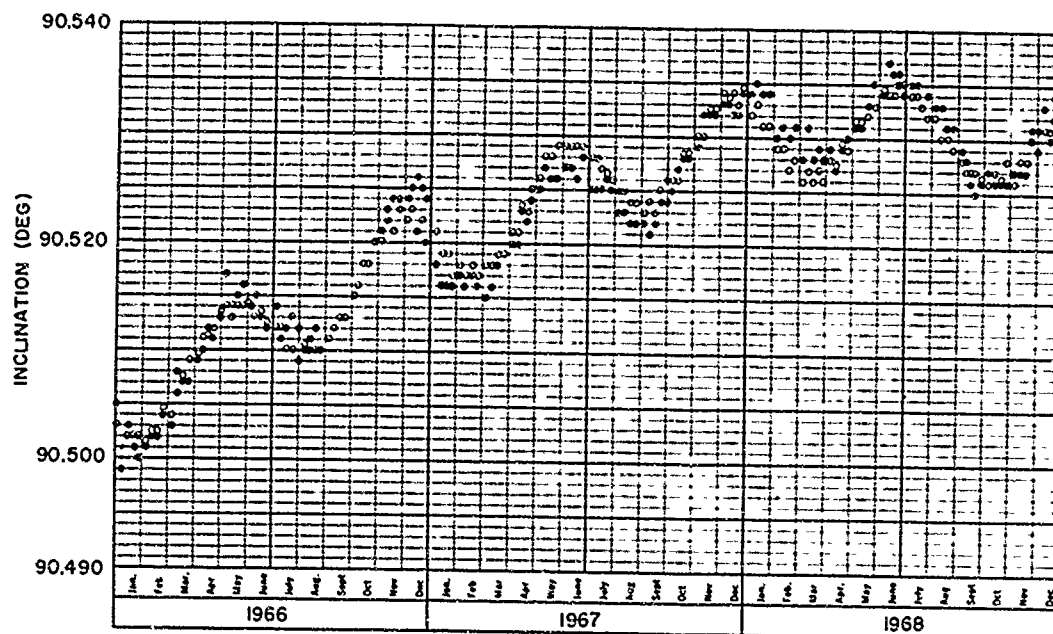
Fig. 11 - Theoretical and observed inclination for Satellite 801. ● Data ○ Theoretical
