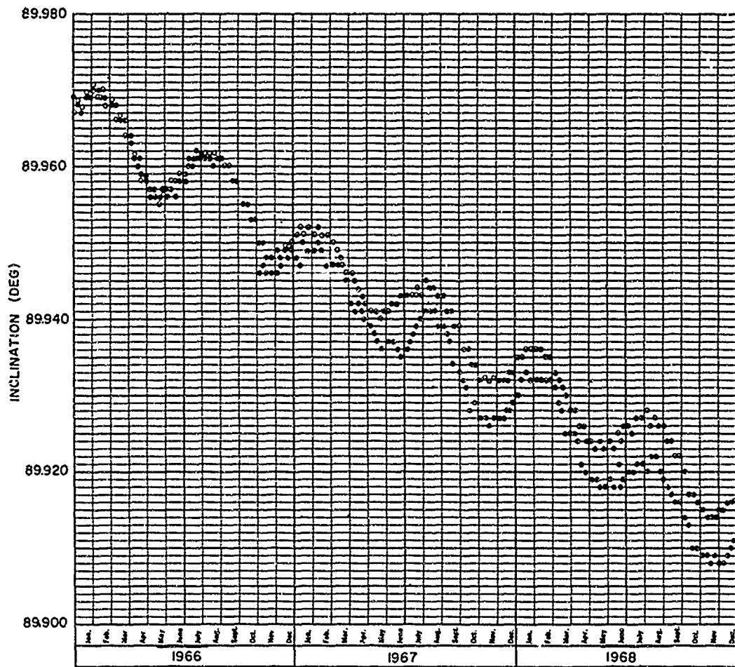
Fig. 9 - Theoretical and observed inclination for Satellite 959. ● Data ○ Theoretical
