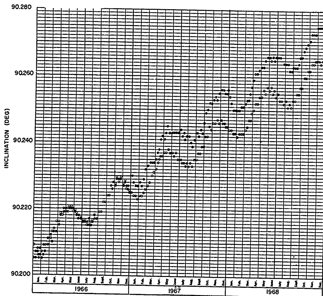
Fig. 12 - Theoretical and observed inclination for Satellite 1314. ● Data ○ Theoretical
