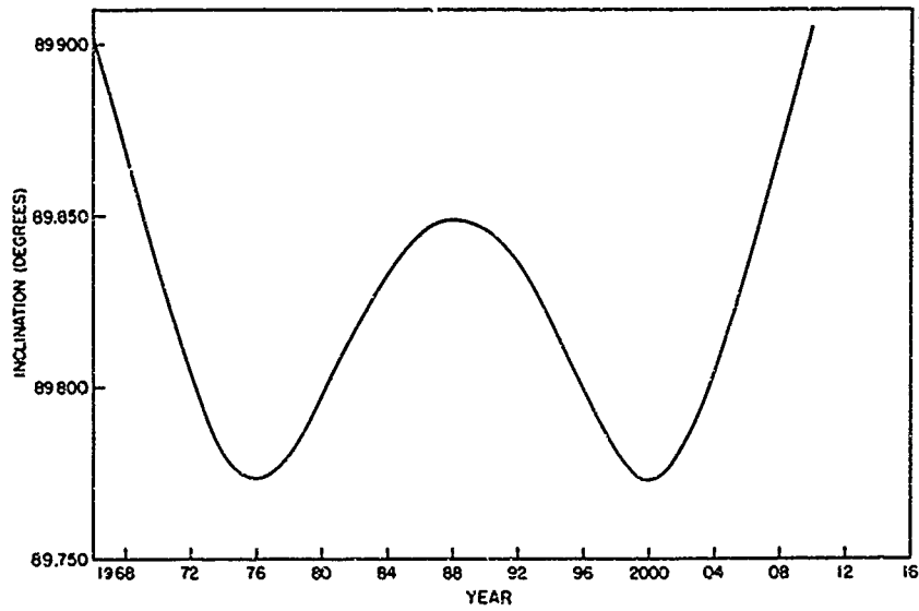
Fig. 16 - Smoothed 40-year variations in inclination of Satellite 902
