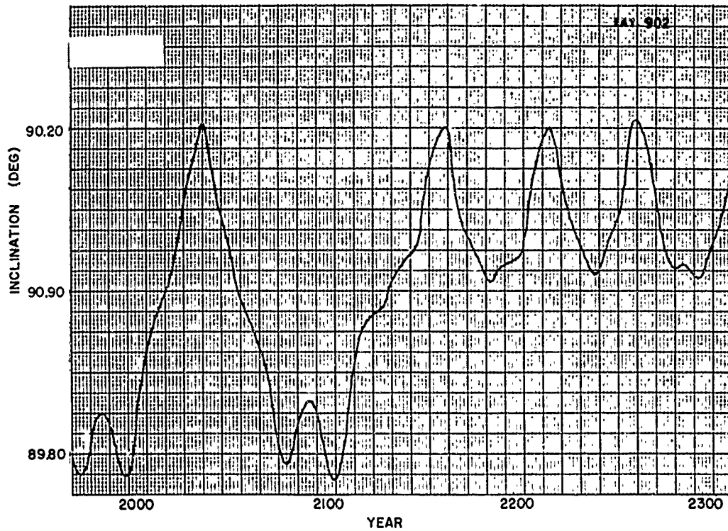
Fig. 17 - Long-term (300-year) predicted inclination for Satellite 902
