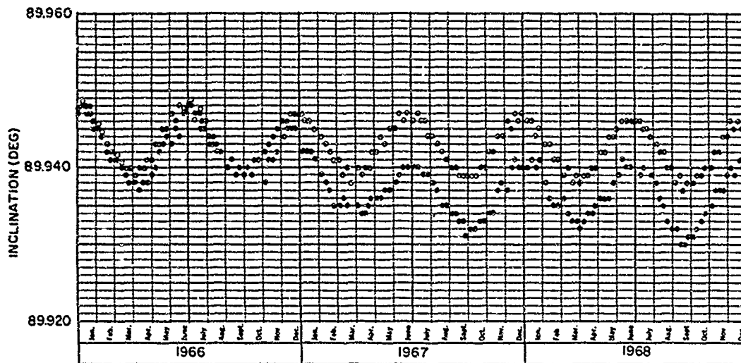
Fig. 7 - Theoretical and observed Inclination for Satellite 704 ● Data ○ Theoretical
