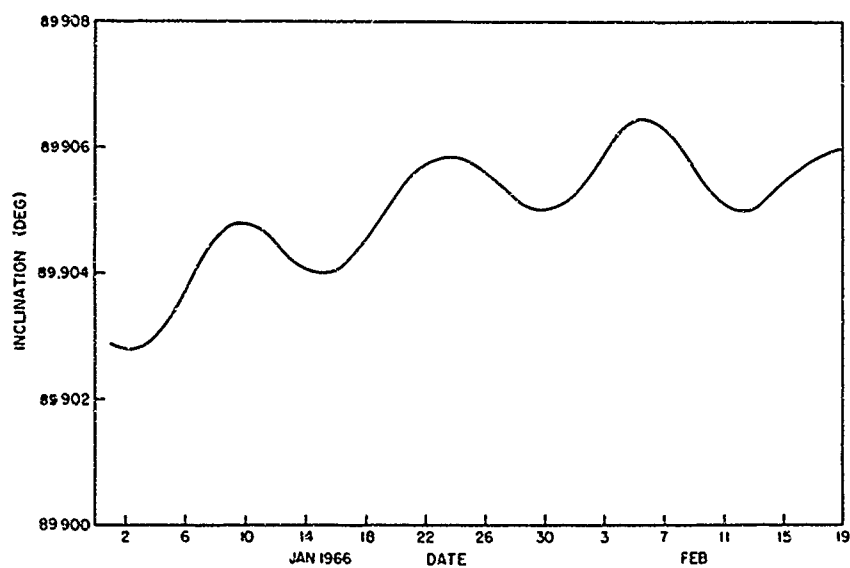
Fig. 14 - Short-term predicted inclination for Satellite 902
