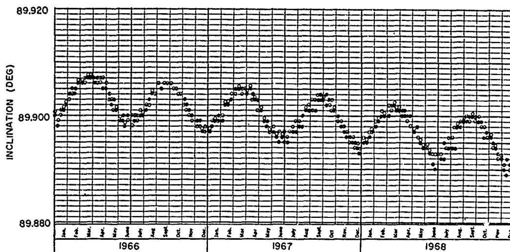
Fig. 8 - Theoretical and observed inclination for Satellite 1514 ● Data ○ Theoretical
