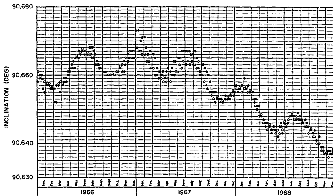
Fig. 10 - Theoretical and observed inclination for Satellite 509. ● Data ○ Theoretical
