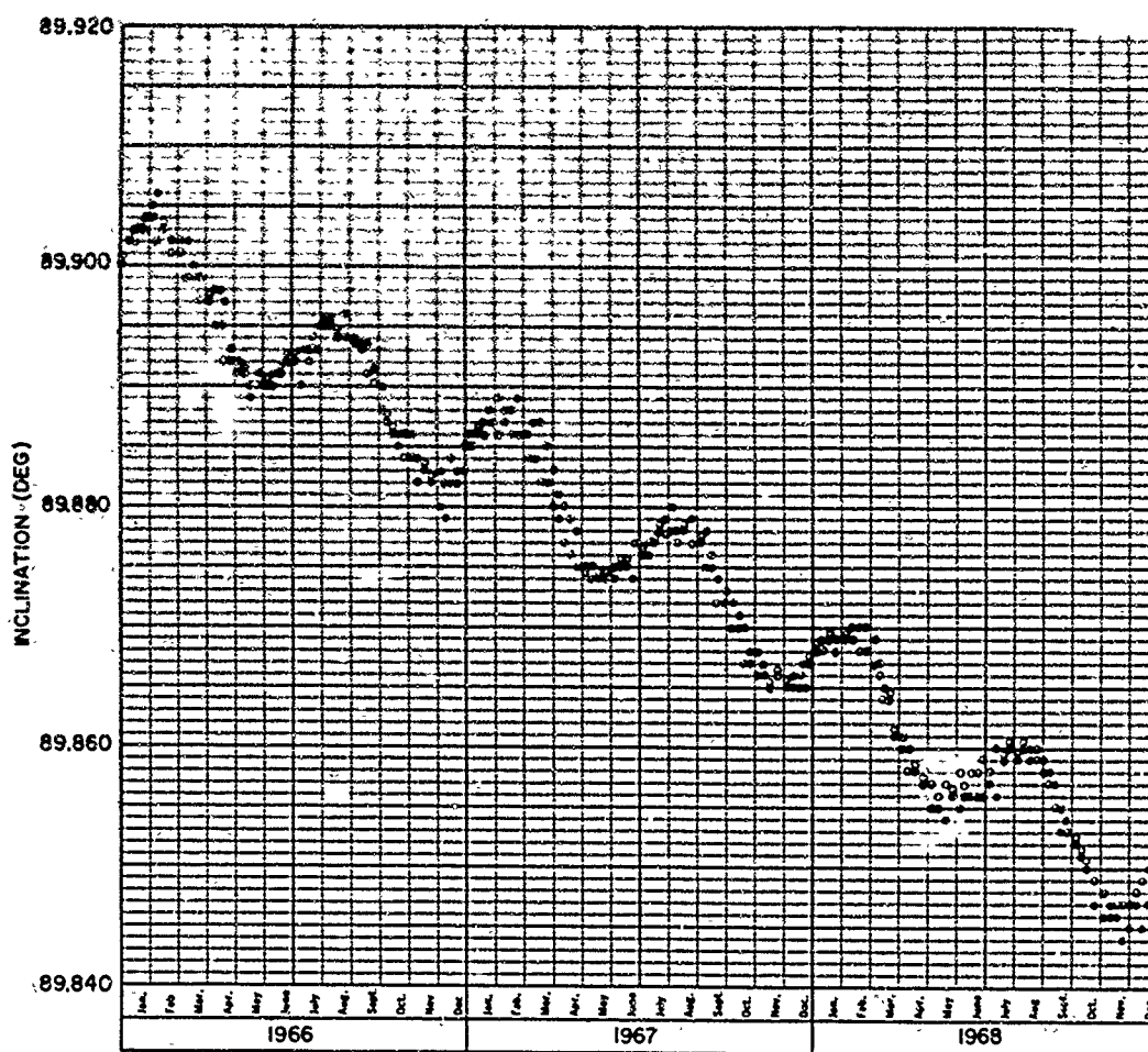
Fig. 5 - Theoretical and observed inclination for Satellite 902 after correction for precession and nutation
