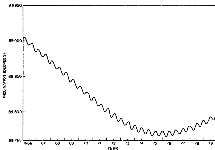
Fig. 15 - Long-term variations in inclination of Satellite 902
