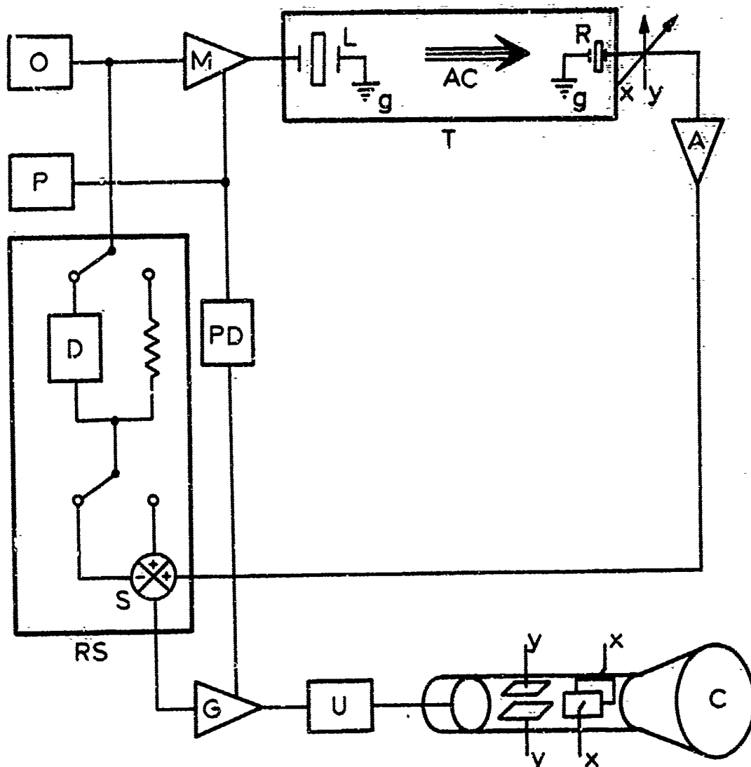
Figure V.7. Schematic of Inclined Reference Simulation
