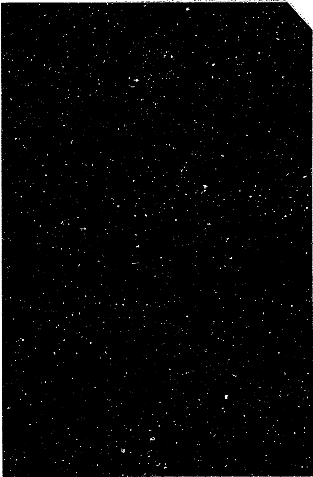
Figure V.34. Reconstruction from Hologram #13
