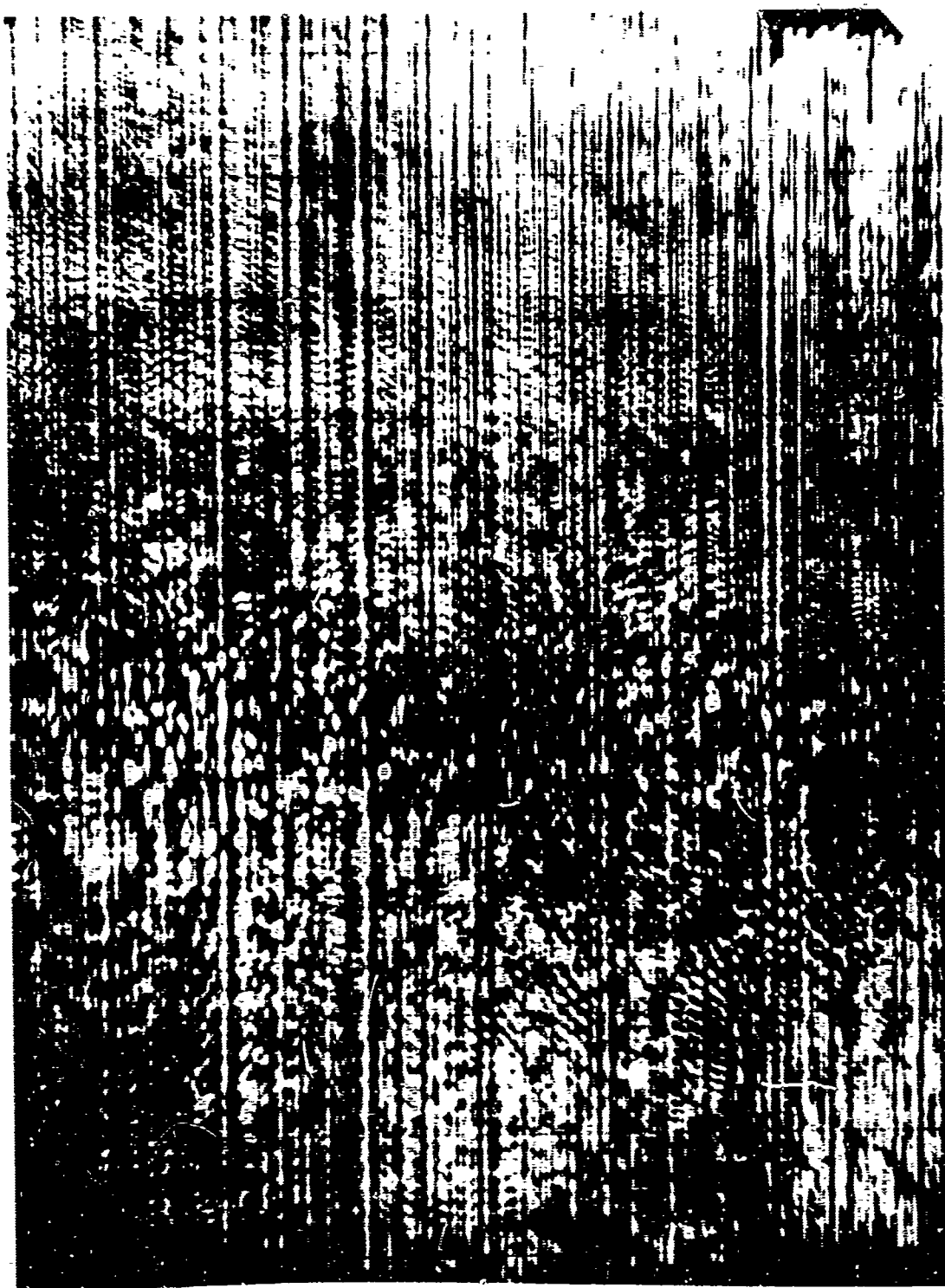
Figure V.36. Hologram #14, 0° Simulated Reference Angle
