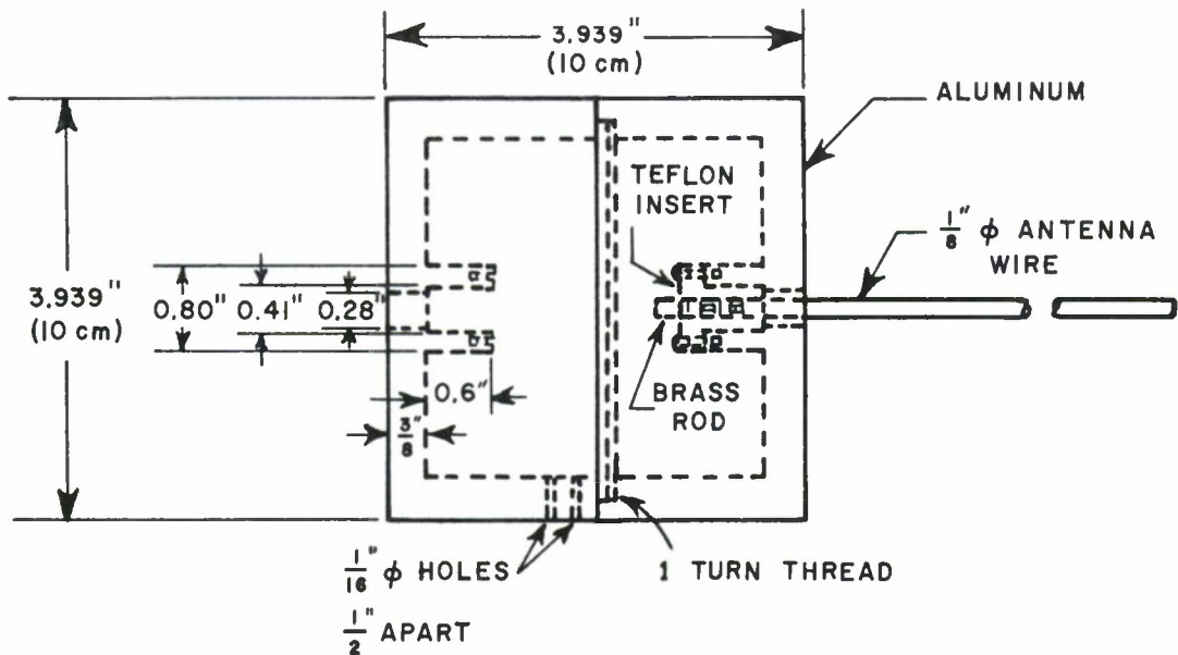
(a) MODIFIED DIPOLE ANTENNA WITH CYLINDRICAL SHELL
