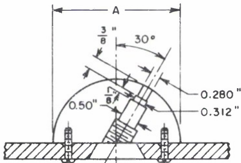
SPHERE ( VEE-ANTENNA )
