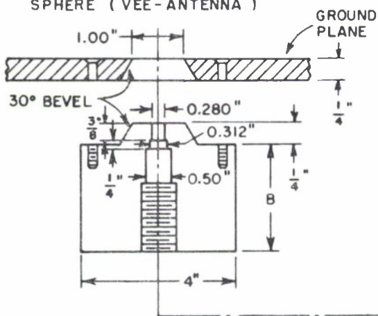
BASE FITTING FOR MONOPOLE AND VEE-ANTENNA ON GROUND PLANE
