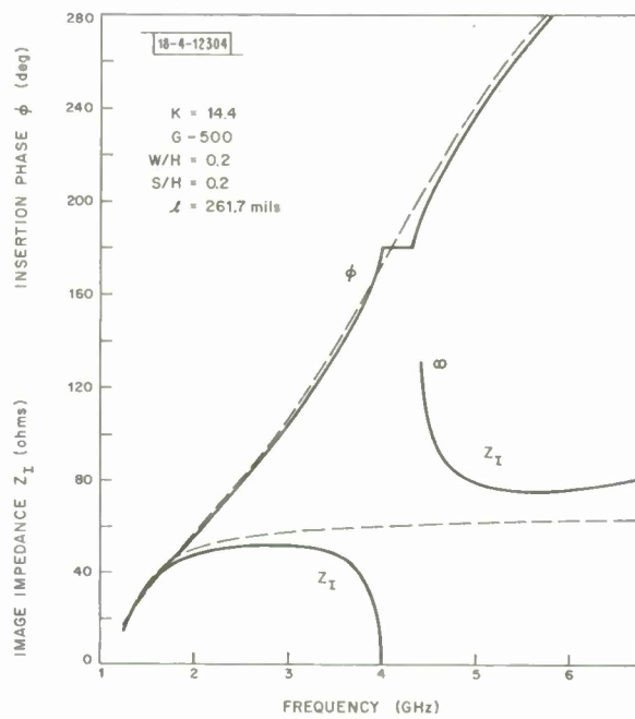
Fig. 25. Theoretical image impedance and insertion phase of a microstrip meander line on a demagnetized ferrite (G500) substrate.
