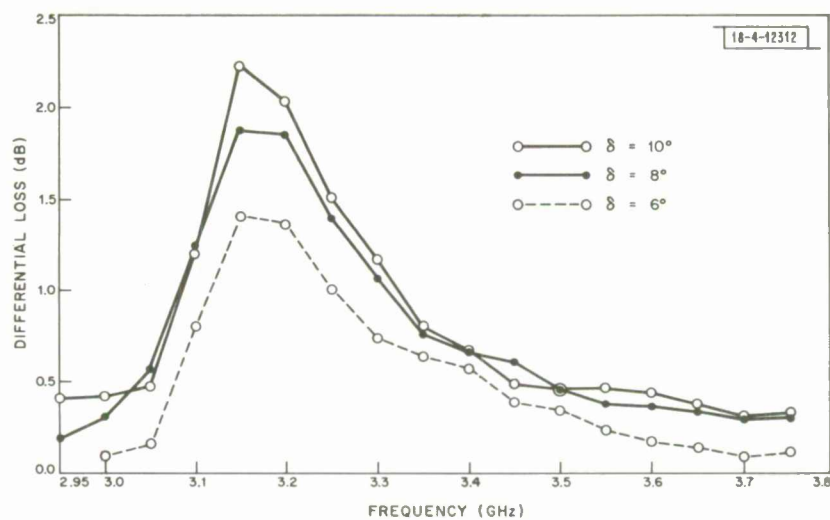
Fig. 40. Curves of differential loss in decibels vs frequency for differential attenuator with 6°, 8°, and 10° of differential phase shift.
