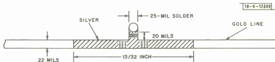
Fig. 32. Enlarged diagram of experimental bilateral attenuator.
