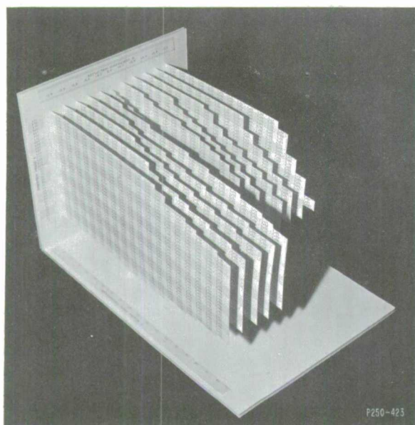
Fig. 14. Three-dimensional representation showing all possible problem solutions of |G| > 1 in reflection-insertion phase-differential phase space.
