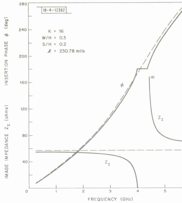
Fig. 23. Theoretical image impedance and insertion phase of microstrip meander line on dielectric ( K = 16 ) substrate.
