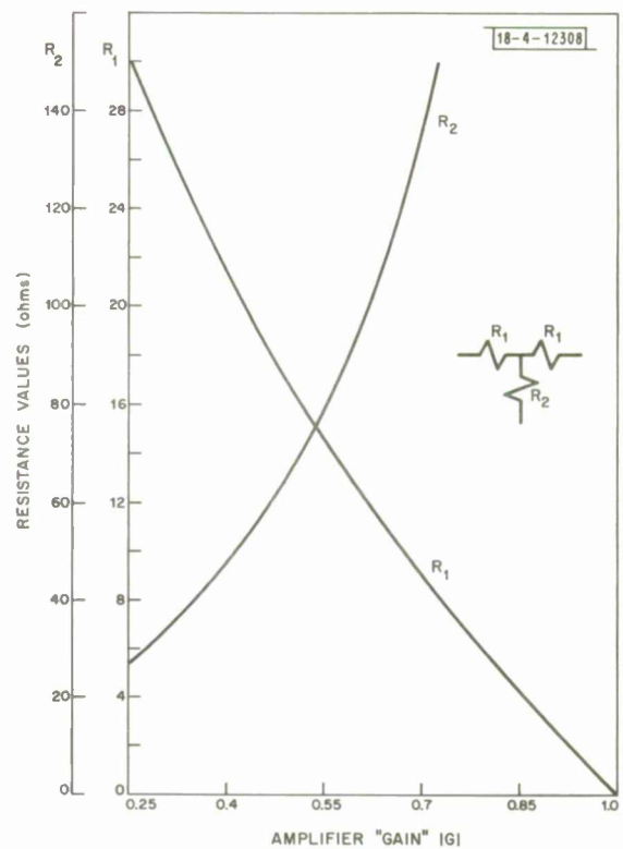
Fig. 31. Resistance values for T networks with various "gains."
