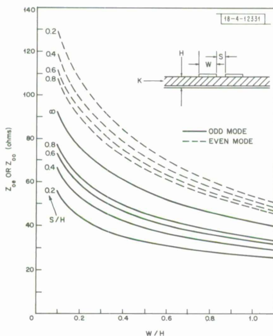
Fig. B-8(a). Even- and odd-mode impedances for coupled microstrips with parameter S/H ; substrate K = 14.4 (dielectric).
