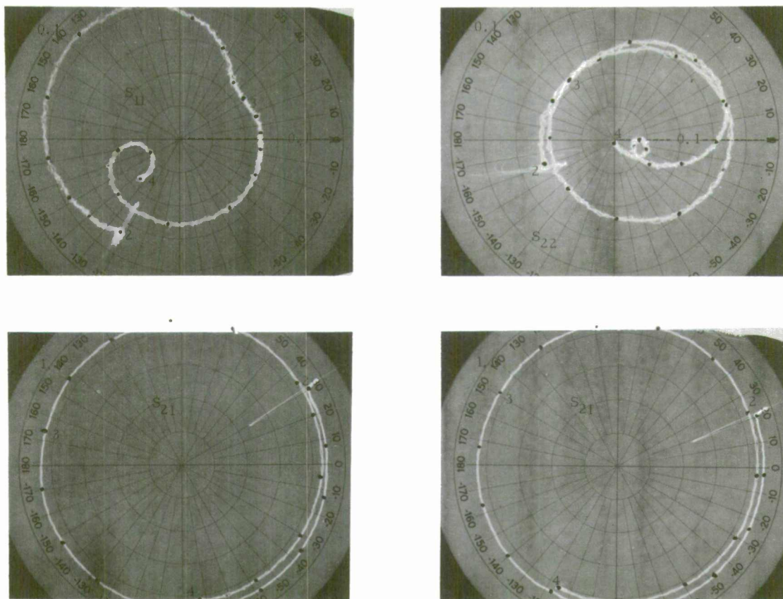
Fig. 27. Polar display of complex reflection coefficients and transmission coefficients for two-meander, chrome-gold line on G500 ferrite. Graphs are swept from 2 to 4 GHz.
