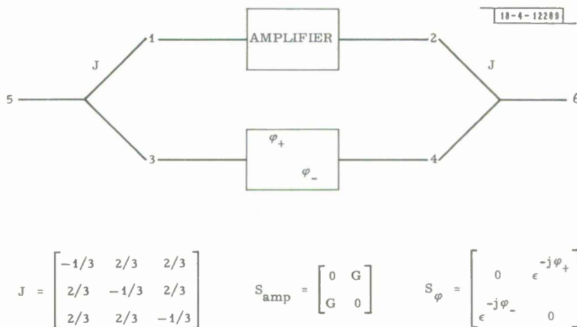
Fig. 2. Parallel-parallel circuit arrangement.
