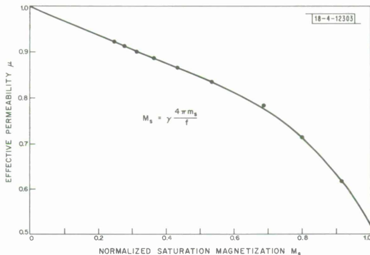
Fig. 24. Curve of effective permeability vs normalized saturation magnetization for a microstrip line on demagnetized ferrite substrate.
