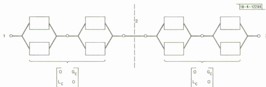
Fig. 20. Iteration of two composite cascaded differential networks.
