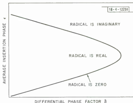
Fig. 6. Diagram identifying areas of gain profiles of Figs. 4 and 5 with certain constraints on Eq. (59).
