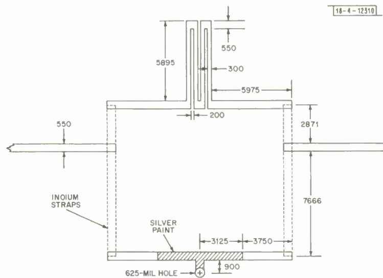
Fig. 34. Layout of differential attenuator model as cut from a Rubylith; all dimensions are in mils magnified by 25.
