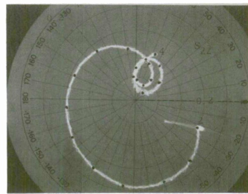
Fig. 37. Polar display of complex reflection and transmission coefficients of meander-line section of differential attenuator. Graphs are shown swept from 2 to 4 GHz.
