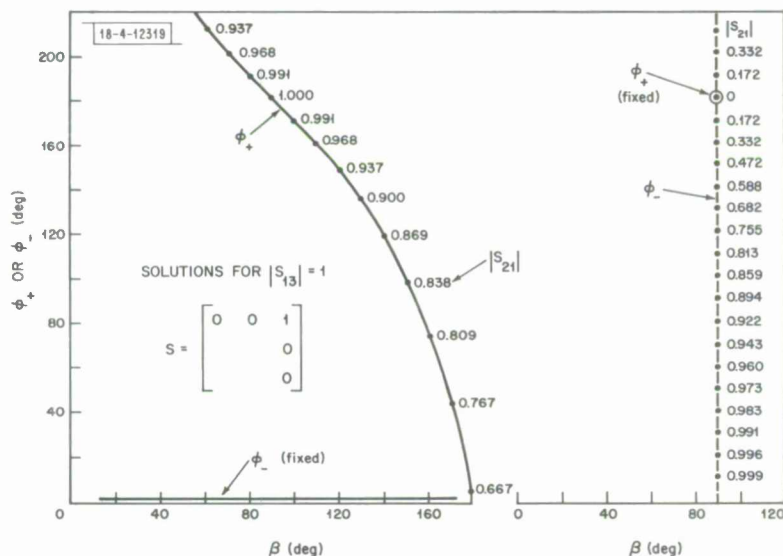
Fig. A-8. Relations among variables required for |S_{13}| = 1.0 in scattering matrix of single phase-shift Diphalator.
