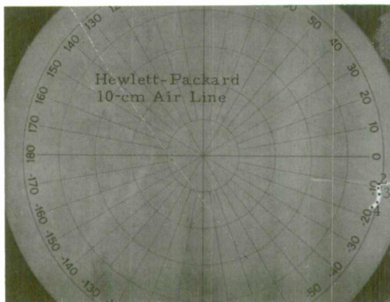
Fig. 30. Polar display of phase correction to be added to all transmission coefficient measurements. Curve is shown swept from 2 to 4 GHz.
