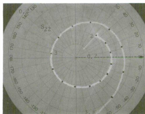
Fig. 38. Polar display of complex reflection and transmission coefficients of bilateral attenuator section from differential attenuator. Graphs are shown swept from 2 to 4 GHz.
