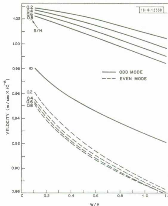
Fig. B-7(b). Even- and odd-mode velocities for coupled microstrips with parameter S/H ; substrate K = 16 (dielectric).
