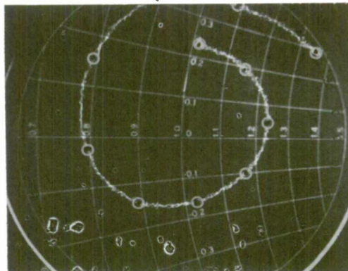
S_{22} : scale 0.2 at outer circle.
