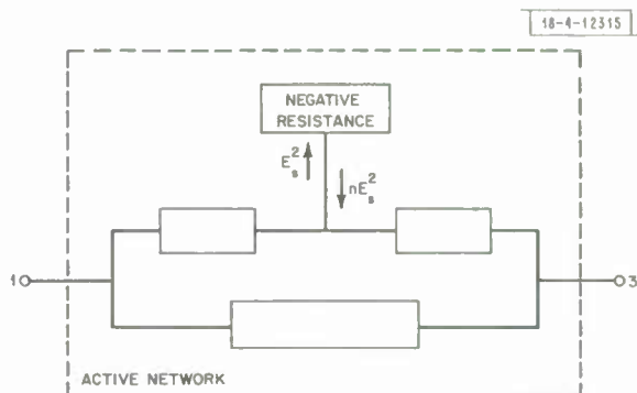
Fig. A-2. Two-port active network obtained from negative resistance and basic lossless three-port circuit.
