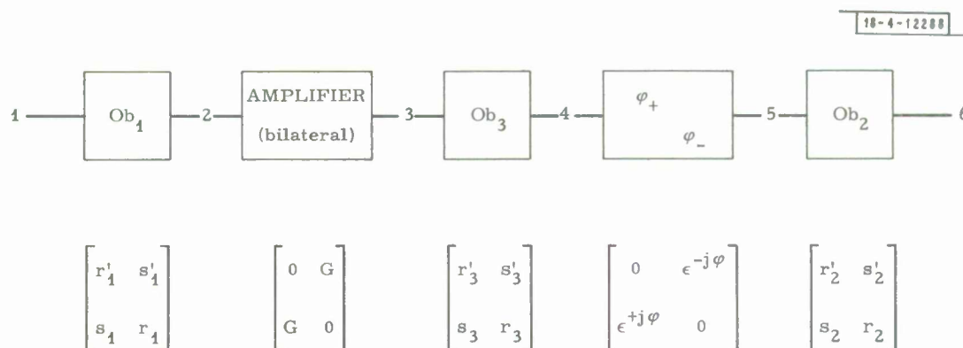
Fig. 1. General cascade connection.
