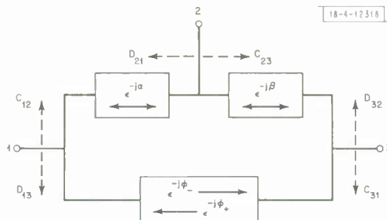
Fig. A-6. Schematic diagram of Diphallator with single differential phase-shift element.
