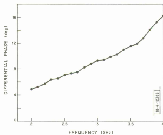
Fig. 28. Curve of differential phase shift vs frequency for two-meander, chrome-gold line on G500 ferrite.
