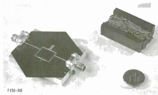
Fig. 36. Microstrip differential attenuator shown with microstrip latching yoke.
