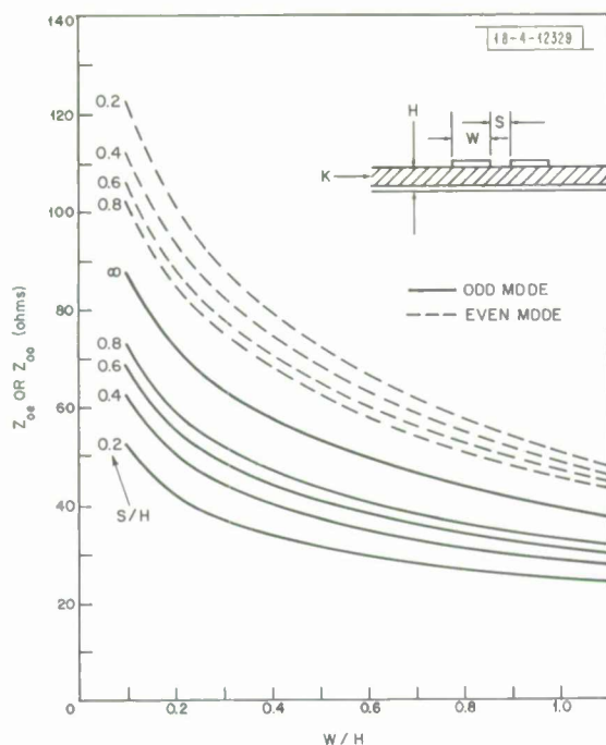
Fig. B-7(o). Even- and odd-mode impedances for coupled microstrips with parameter S/H ; substrate K = 16 (dielectric).
