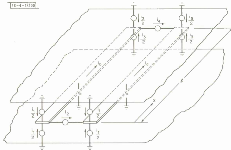
Fig. 21. Notation used in deriving all-pass filter characteristics in stripline transmission system. After E. M. T. Jones and J. T. Bolljahn. 18
