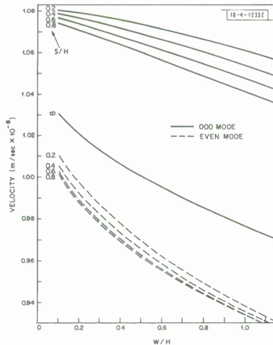
Fig. B-8(b). Even- and odd-mode velocities for coupled microstrips with parameter S/H ; substrate K = 14.4 (dielectric).
