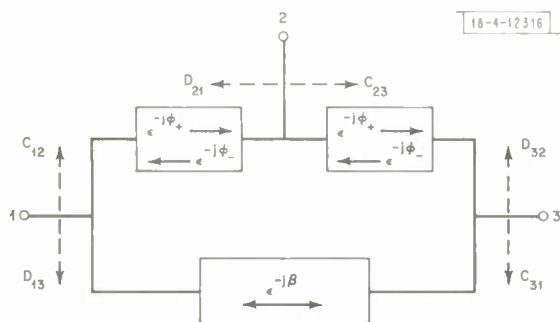
Fig. A-3. Schematic diagram of Diphilator with two differential phase-shift elements.
