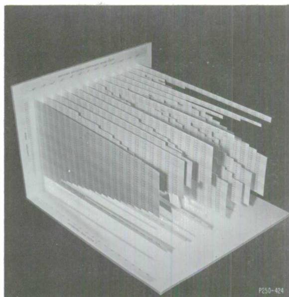
Fig. 15. Illustration showing all solutions of |G| > 1 as a function of amplifier reflection coefficient phase angle, insertion phase \epsilon , and differential phase factor \delta ; omplifier reflection coefficient |R| = 0.2 .
