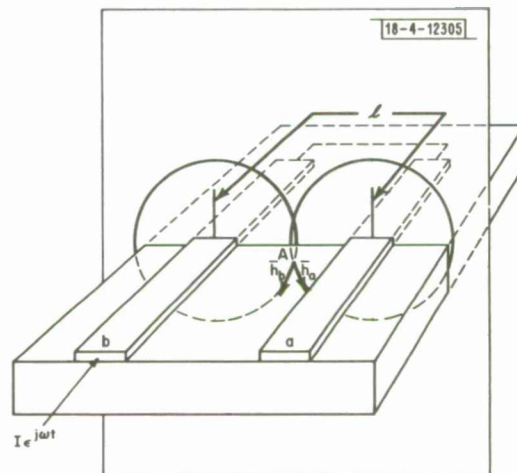
Fig. 26. Spatial configuration used in deriving requirements for magnetic field circular polarization.
