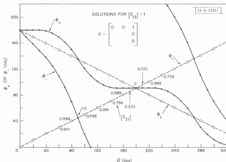
Fig. A-5. Relations among variables required for |S_{13}| = 1.0 in scattering matrix of two phase-shift Diphalator.
