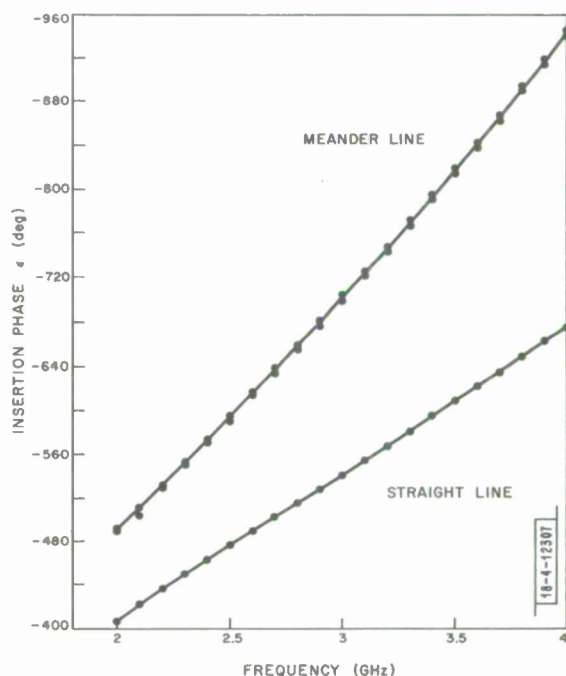
Fig. 29. Curves of insertion phase vs frequency for line with two meanders and straight line both on 2-inch ferrite G500 substrate.
