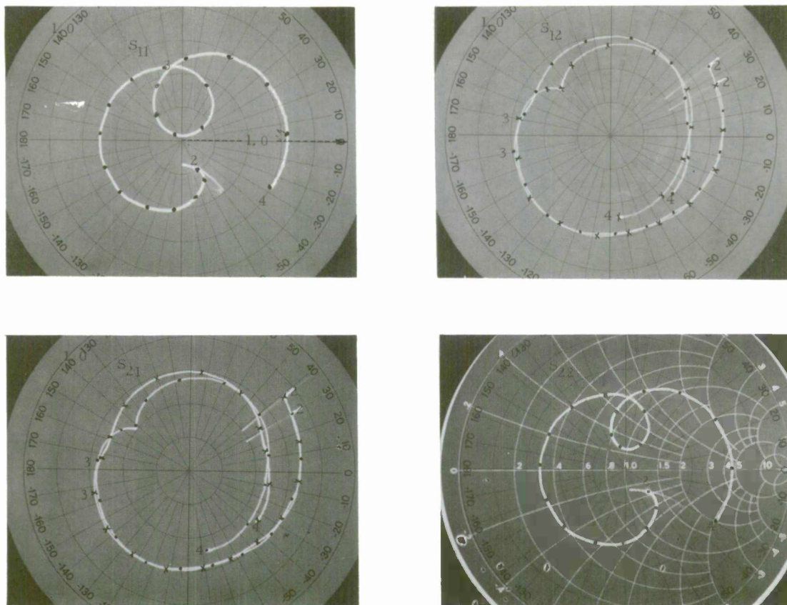
Fig. 39. Polar display of complex scattering coefficients for differential attenuator. Graphs are shown swept from 2 to 4 GHz.
