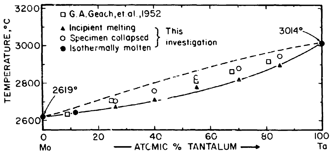
Figure III.A.32.2: Melting Temperatures of Ta-Mo Alloys.
