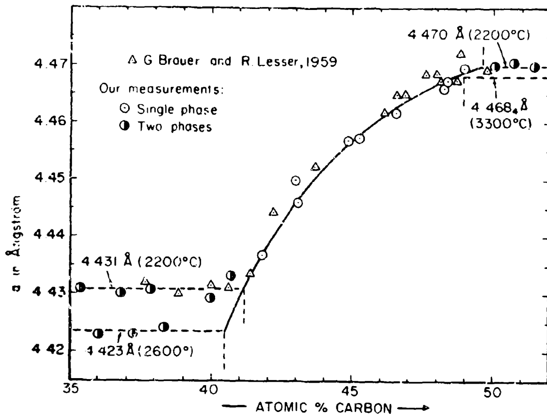
Figure III.B.5.3: Lattice Parameters of the Niobium Monocarbide Phase.
