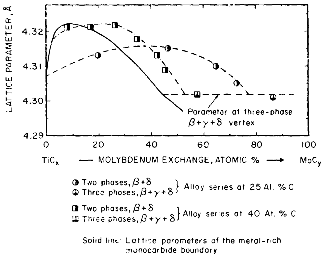
Figure III.E.6.18. Determination of the Coexisting Monocarbide Compositions in Two-Phase, \beta+\delta , Alloys by Lattice Parameter Measurements
