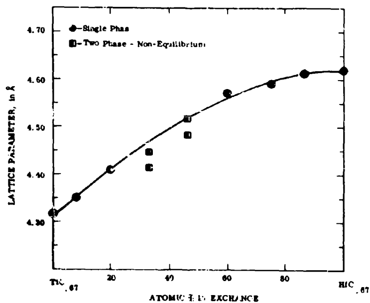
Figure III.E.2.3: Lattice Parameters of the (\text{Ti, Hf})\text{C}_{1-x} Solid Solution at 40 At.% C. Alloys Equilibrated at 1500°C.
