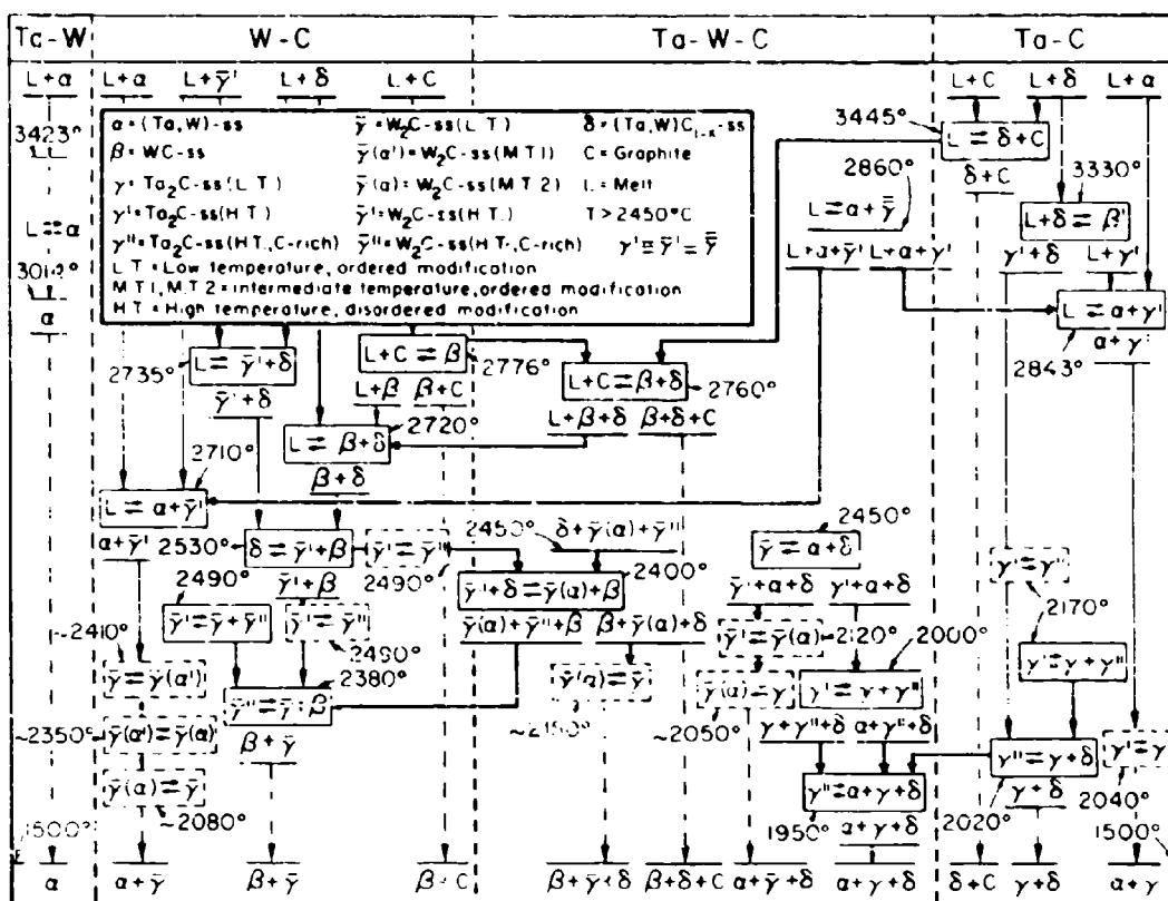
Figure III.E.15.2. Reaction Diagram for the Ta-W-C System
