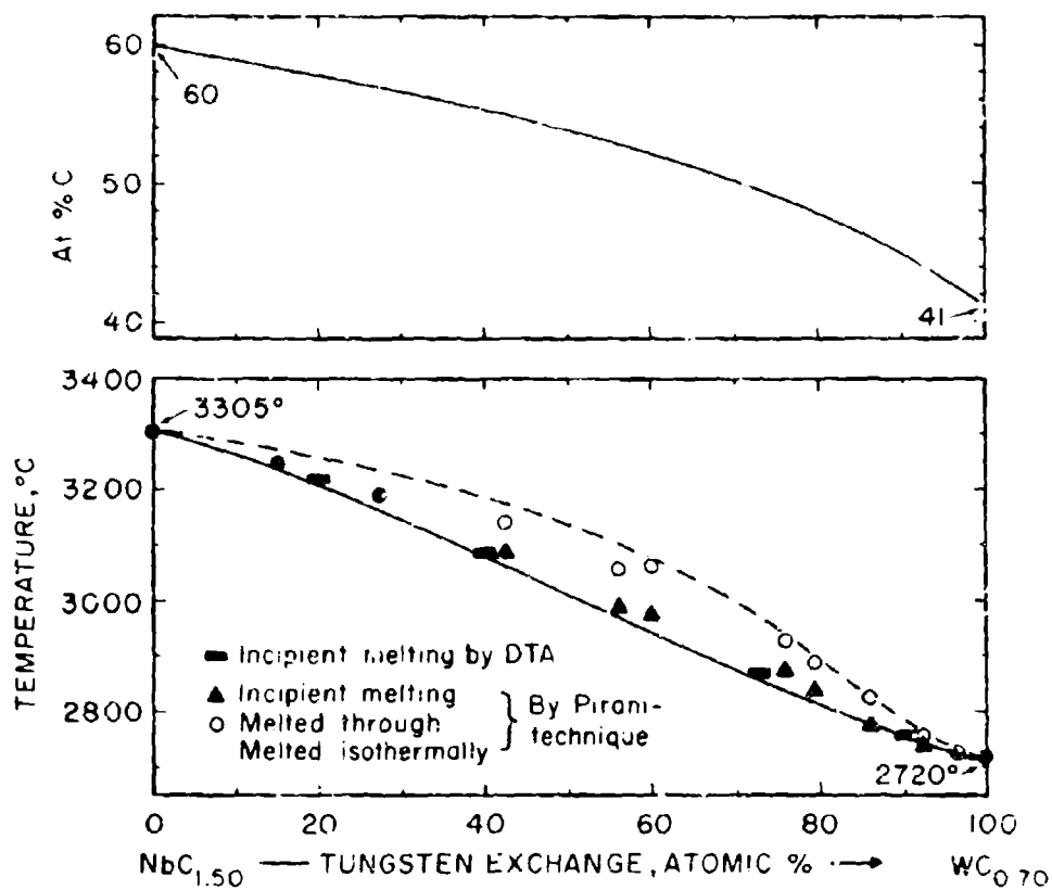
Figure III. E. 13.15: Melting Along the (\text{Nb}_2\text{W})\text{C}_{1-x} + \text{C} Eutectic Trough.
