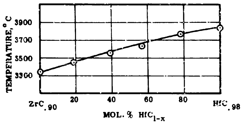
Figure III.E.7.22. Melting Temperatures of Monocarbide Alloys at (Zr,Hf)C 0.90-.98
