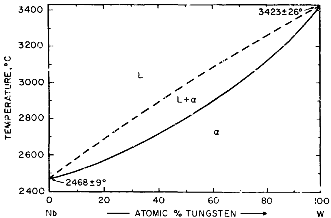
Figure III.A.30.1: Constitution Diagram of the System Nb-W.
