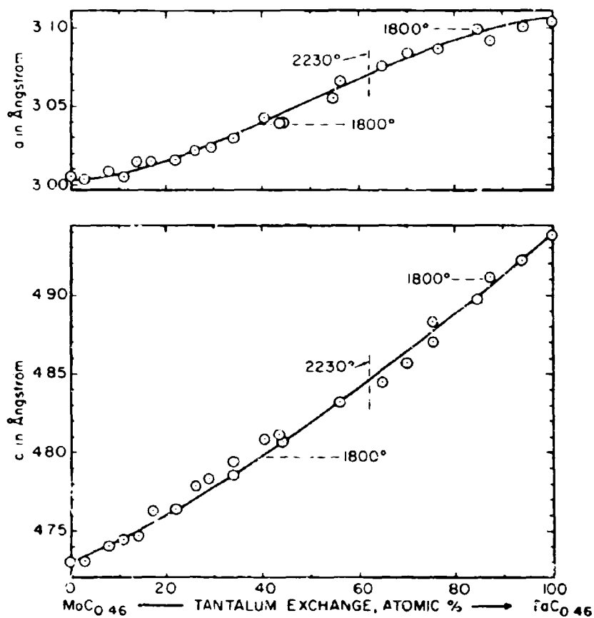
Figure III.E.14.18: Lattice Parameters of the (\text{Ta}, \text{Mo})_2\text{C} Solid Solution. Alloys Rapidly Cooled from 2500°C. Parameters are Based on Indexing According to the L'3-Type.
