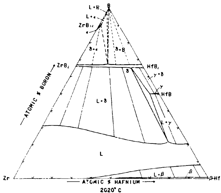
Figure III.1.3.14. Isothermal Section of the Zr-Hf-B System at 2020°C
