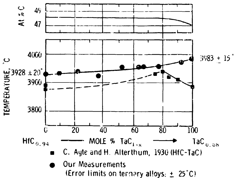
Figure III.E.9.31. Maximum Solidus Temperatures of the Monocarbide Solid Solutions
