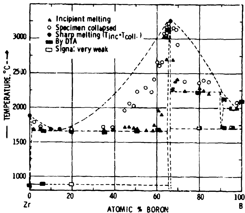
Figure III.C.2.2: Melting Temperatures of Zr-B Alloys.
