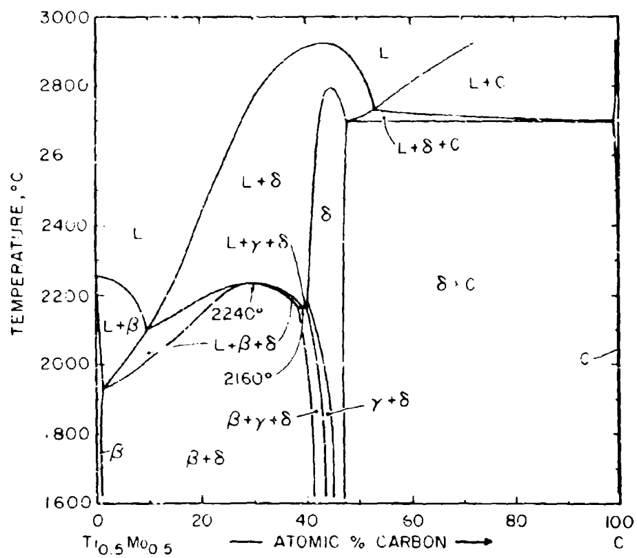
Figure III.E.6.6. Isopleth \text{Ti}_{0.5}\text{Mo}_{0.5}\text{-C}
