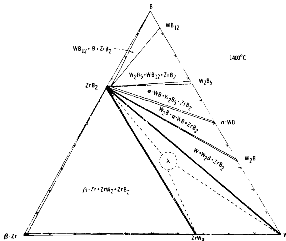
Figure III.1.4.1. Isothermal Section of the Zr-W-B System at 1400°C
