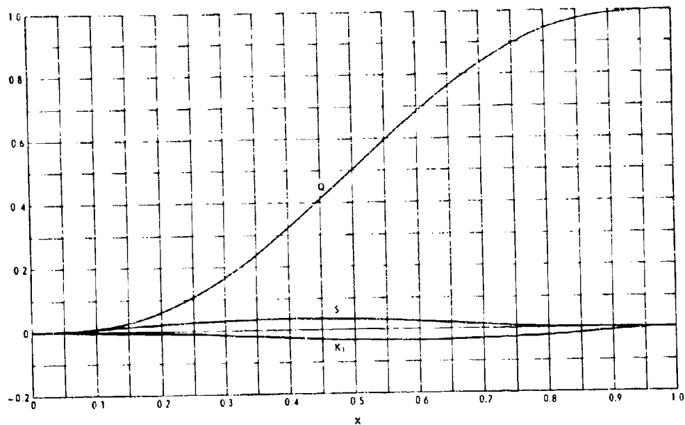
Figure 5 - "Quadratic" Polynomial: Pointed End - Variation of Independent Polynomials
