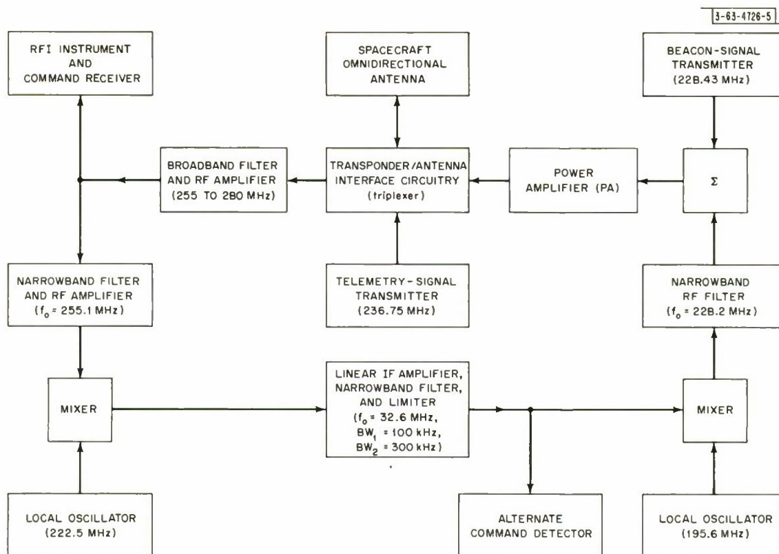
Fig. 4. LES-5 transponder and communications-associated equipments.
