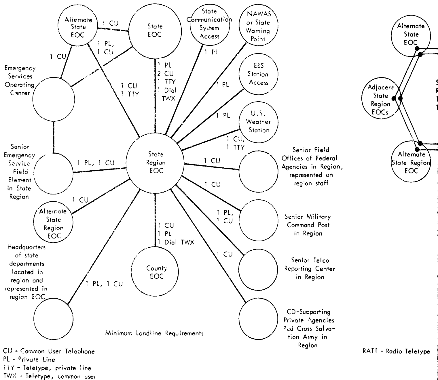
Figure 4 MINIMUM CIVIL DEFENSE LANDLINE AND RADIO REQUIREMENTS FOR A STATE SUBDIVISION (e.g. State Mutual Aid Region) -- SCHEMATIC
