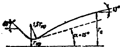
Fig. 3.5. Optimum shaped nozzle: ----- conical nozzle; ———— shaped
