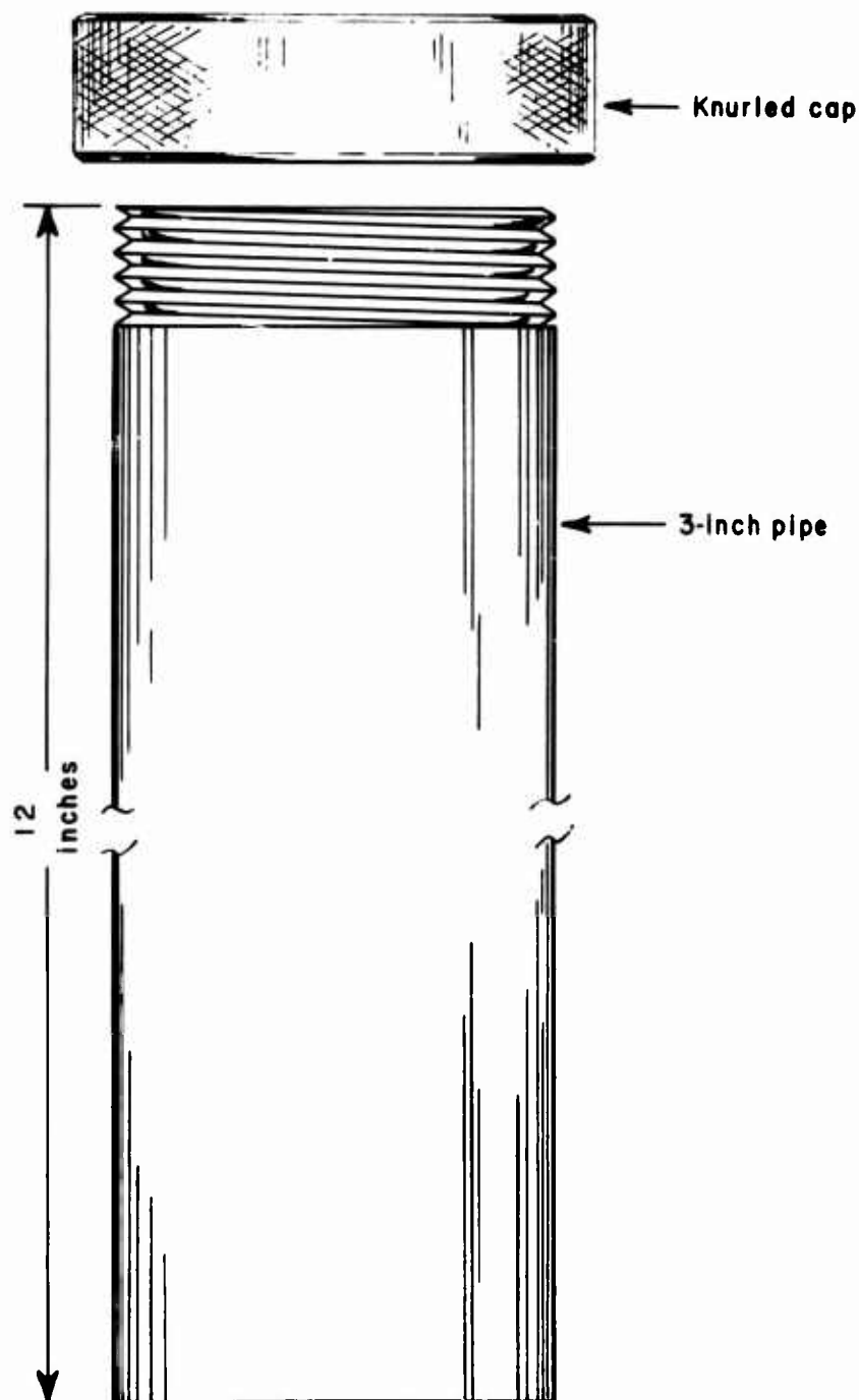
FIGURE 1. - Metal Safety Shield for Beverage Bottle Oven Test.
