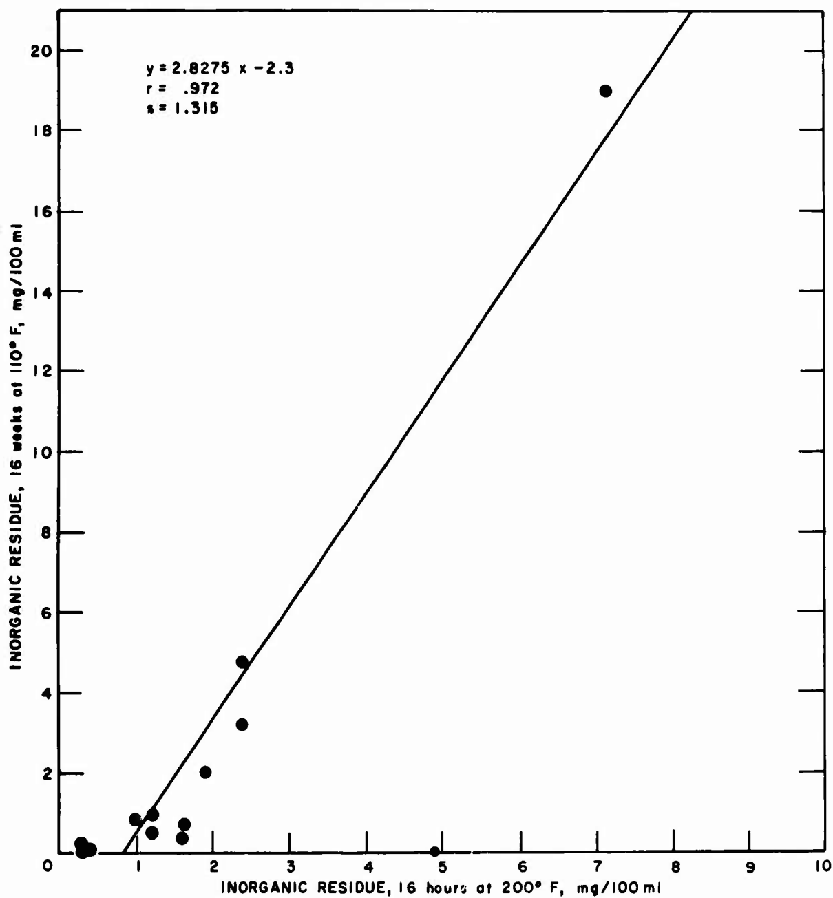
FIGURE 10. - Inorganic Residue Formed in 16 Weeks of 110° F Storage Versus Inorganic Residue Formed in 16-Hour 200° F Oven Test.
