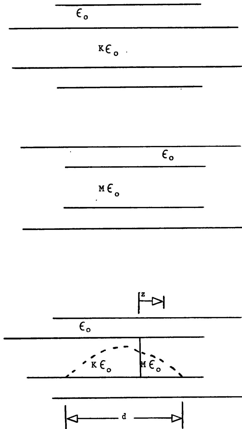
Fig. 6 Steps of the Resonance Calculation
