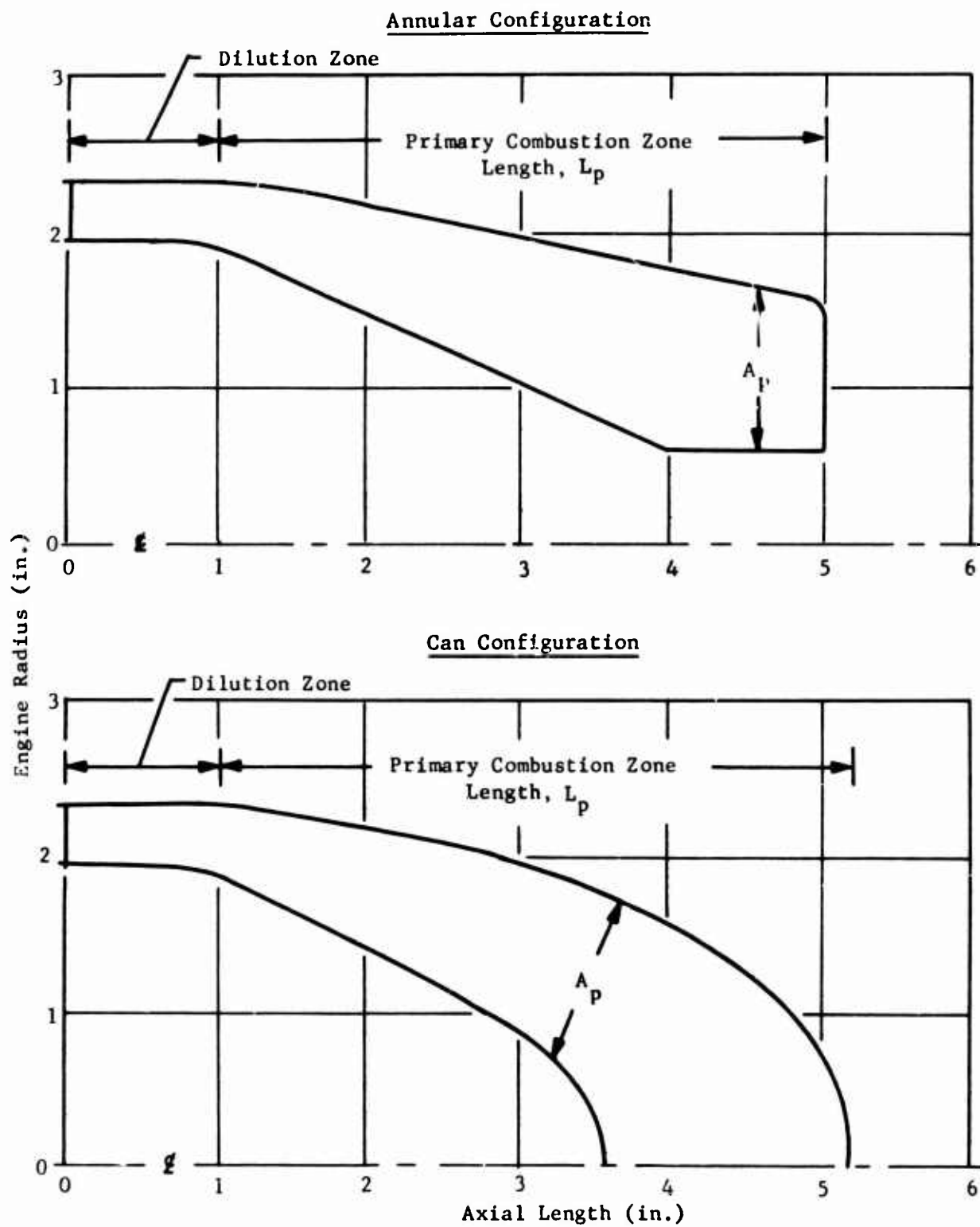
Figure 8. Schematic of Basic End-Mounted Combustor Envelopes.
