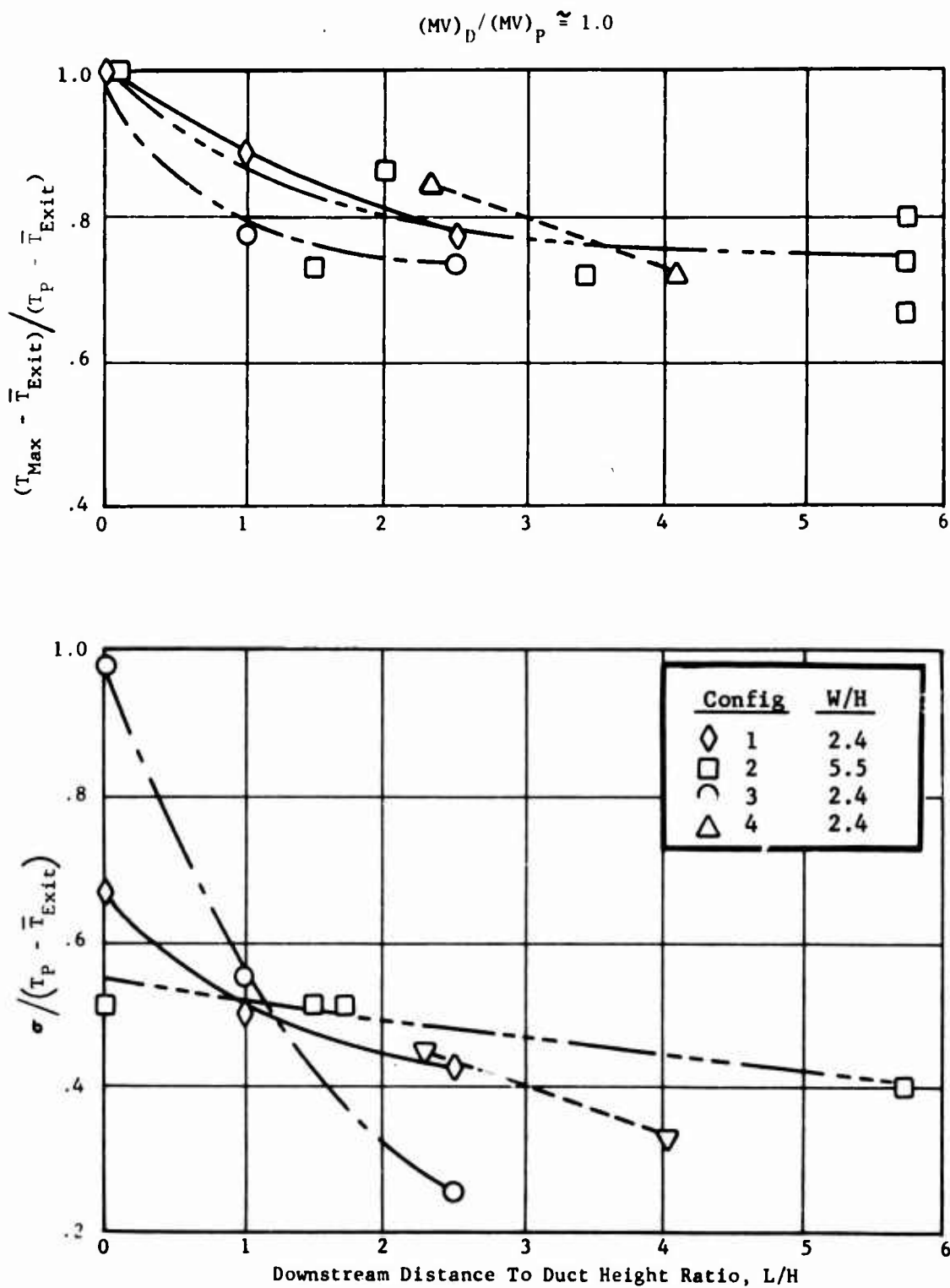
Figure 42. Mixing Efficiency as a Function of Downstream Distance to Duct Height Ratio.
