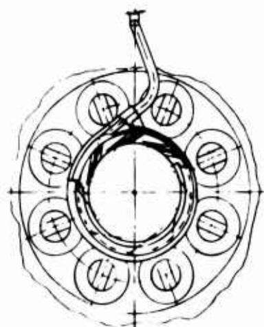
SECT B-B
