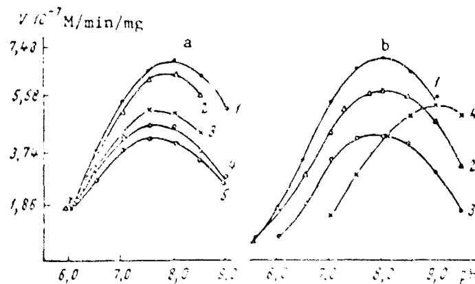
Fig. 1. The effect of various cations (a) and anions (b) on the form of the relation of v_1 to pH : ( [S]=1 \times 10^{-5} M)
