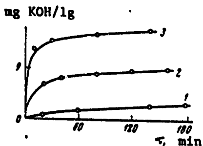
Fig. 3. Increase in acidity of the reaction medium for experiments with various initial acidity (mg KOH/1 g):
