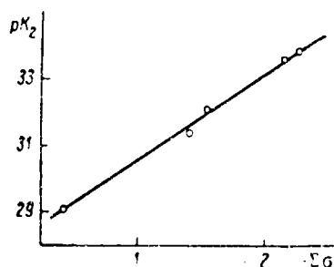
Fig. 2. Correlation of the values of instability constants of Hg phosphorus dithio acids complexes with \Sigma\sigma of the substituents at P atom
