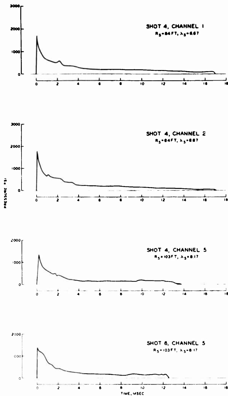
Figure A8 Pressure-time traces for values listed in Table 5.5.
