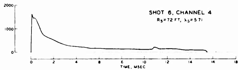
Figure A7 Pressure-time traces for values listed in Table 5.5.
